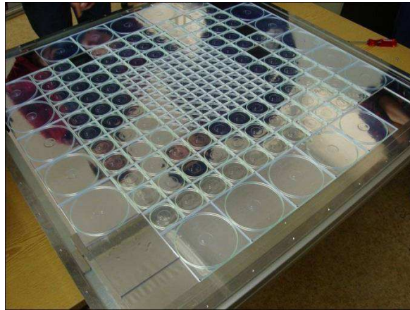
FIGURE 5.34. A scintillator tile plane for the 1 m 3 prototype calorimeter. Each tail is equipped with a wavelength shifting fiber read out by a SiPM.
