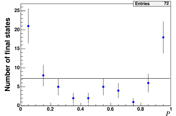
FIG. 9: The distribution of \tilde{P} in the data, with one entry for each final state considered by SLEUTH.
