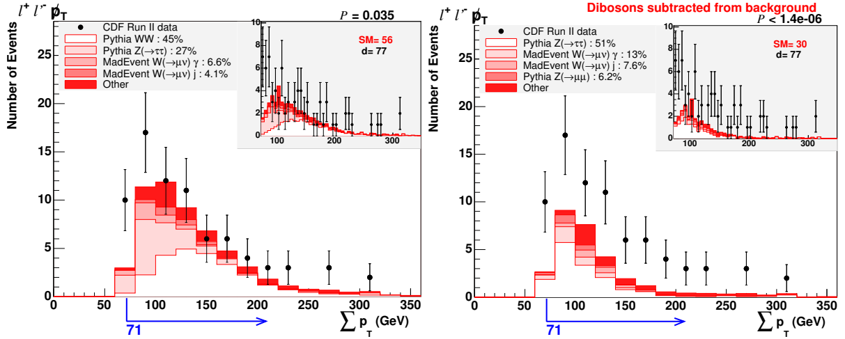
FIG. 8: (Left) The final state \ell^+\ell'^-\not{p} , consisting of events with an electron and muon of opposite sign and missing transverse momentum, in 927 \text{ pb}^{-1} of CDF data. (Right) The same final state with standard model WW , WZ , and ZZ contributions subtracted, and with the VISTA correction factors re-fit in the absence of these contributions. SLEUTH finds the final state \ell^+\ell'^-\not{p} to contain a discrepancy surpassing the discovery threshold of \tilde{P} < 0.001 with the processes WW , WZ , and ZZ removed from the standard model background.
