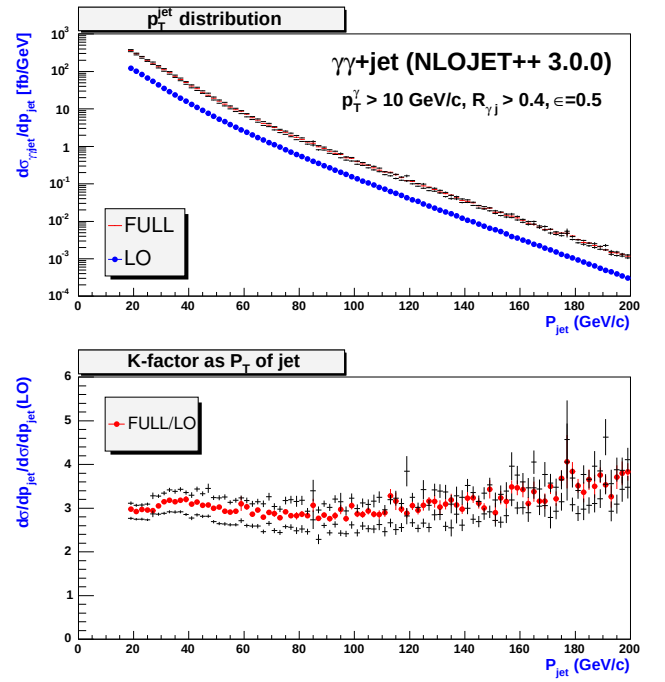
FIG. 17: Calculation of the \gamma\gamma k -factor, as a function of jet transverse momentum. The effect of changing the factorization scale by a factor of two in either direction is also shown (small black points with error bars).
