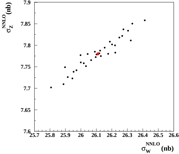
FIG. 16: Variation of the k -factors for inclusive W and Z production under different choices of parton distribution functions, from the Alekhin parton distribution error set [47]. The correlation of the uncertainty on these two k -factors due to uncertainty in the parton distribution functions is 0.955.
