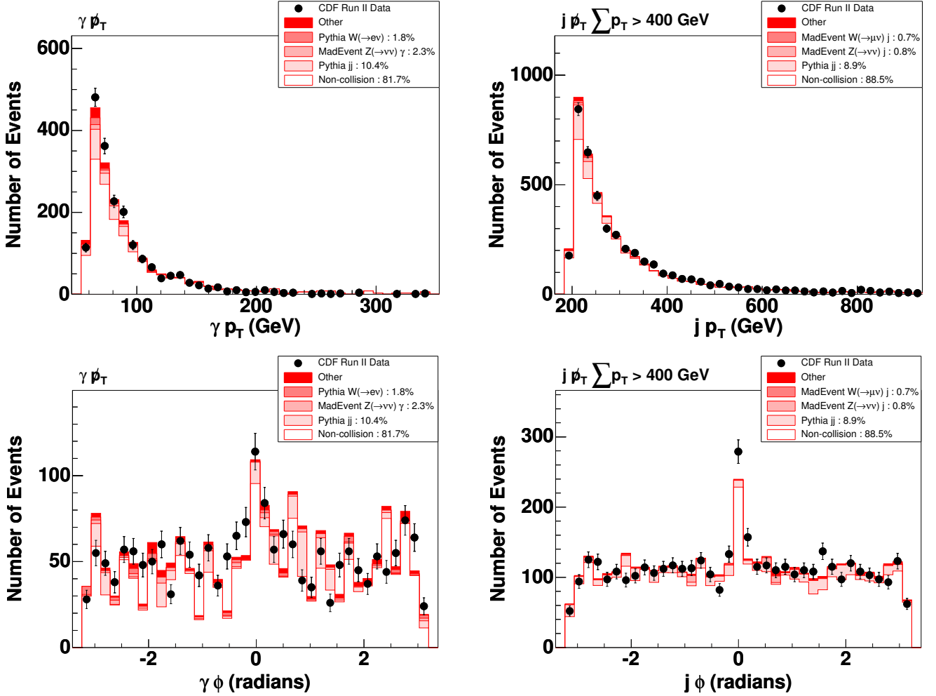
FIG. 15: The distribution of transverse momentum and azimuthal angle for photons and jets in the \gamma p_T and j p_T final states, dominated by cosmic ray and beam halo muons. The vertical axis shows the number of events in each bin. Data are shown as filled (black) circles; the standard model prediction is shown as the shaded (red) histogram. Here the “standard model” prediction includes contributions from cosmic ray and beam halo muons, estimated using events containing fewer than three reconstructed tracks. The contribution from cosmic ray muons is flat in \phi , while the contribution from beam halo is localized to \phi = 0 . The only degrees of freedom for the background to these final states are the cosmic \gamma and cosmic j correction factors, whose values are determined from the global VISTA fit and provided in Table I.
