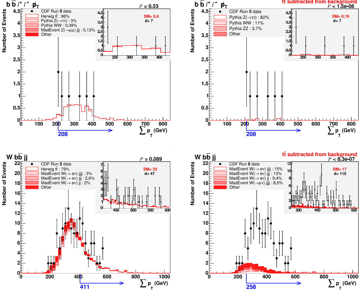
FIG. 7: (Top left) The SLEUTH final state b\bar{b}\ell^+\ell'^-\not{p}_T , consisting of events with one electron and one muon of opposite sign, missing momentum, and two or three jets, one or two of which are b -tagged. Data corresponding to 927\text{ pb}^{-1} are shown as filled (black) circles; the standard model prediction is shown as the (red) shaded histogram. (Top right) The same final state with t\bar{t} subtracted from the standard model prediction. (Bottom row) The SLEUTH final state Wb\bar{b}jj , with the standard model t\bar{t} contribution included (lower left) and removed (lower right). Significant discrepancies far surpassing SLEUTH's discovery threshold are observed in these final states with t\bar{t} removed from the standard model background estimate. If the top quark had not been predicted, SLEUTH would have discovered it.
