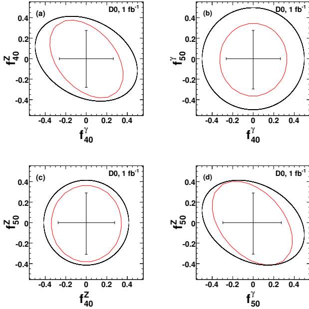
FIG. 1: Limits on anomalous couplings for \Lambda = 1.2 TeV: (a) f_{40}^\gamma vs. f_{40}^Z , (b) f_{40}^\gamma vs. f_{50}^\gamma , (c) f_{40}^Z vs. f_{50}^Z , and (d) f_{50}^\gamma vs. f_{50}^Z , assuming in each case that the other two couplings are zero. The inner and outer curves are the 95% C.L. two-degree of freedom exclusion contour and the constraint from the unitarity condition, respectively. The inner crosshairs are the 95% C.L. one-degree of freedom exclusion limits.
