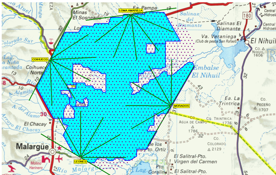
Figure 1: Layout of the Pierre Auger Southern Observatory. The dots represent the position of each of the 1600 SD stations. The 1430 SD stations deployed and activated as of 30 September 2007, lie in the area shaded blue. The 4 FD sites are labeled in yellow, with green line indicating the field of view of the 6 telescopes at each site. To give the scale of the Observatory, the lengths of the green line correspond to 20 km.
