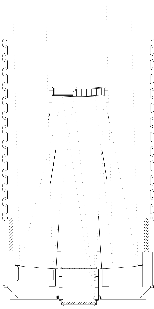
Fig. 3.— SDSS 2.5 m telescope optical configuration, showing the light baffles and a set of rays from the extreme field edge. The first transmissive corrector (the “Gascoigne”, or “common”, corrector) is nearly coincident with the vertex of the primary mirror. The second transmissive corrector, which forms the main structural element of the SDSS mosaic camera (Gunn et al. 1998) is just before the focal service. In spectroscopic mode, the imaging camera, including this corrector, is dismantled and replaced with the spectroscopic corrector and the spectroscopic plug plate and fiber harnesses. The baffle system consists of the wind baffle (outside the beam to the primary mirror) and the secondary, conical and primary baffles (inside). The conical baffle is suspended about halfway between the primary and secondary. Light enters the wind baffle through the annular opening at the top. The outer interlocking “C”-shaped baffles which form the upper tube are carried by an independently mounted and driven wind baffle mechanism and take the major wind loads on the telescope.
