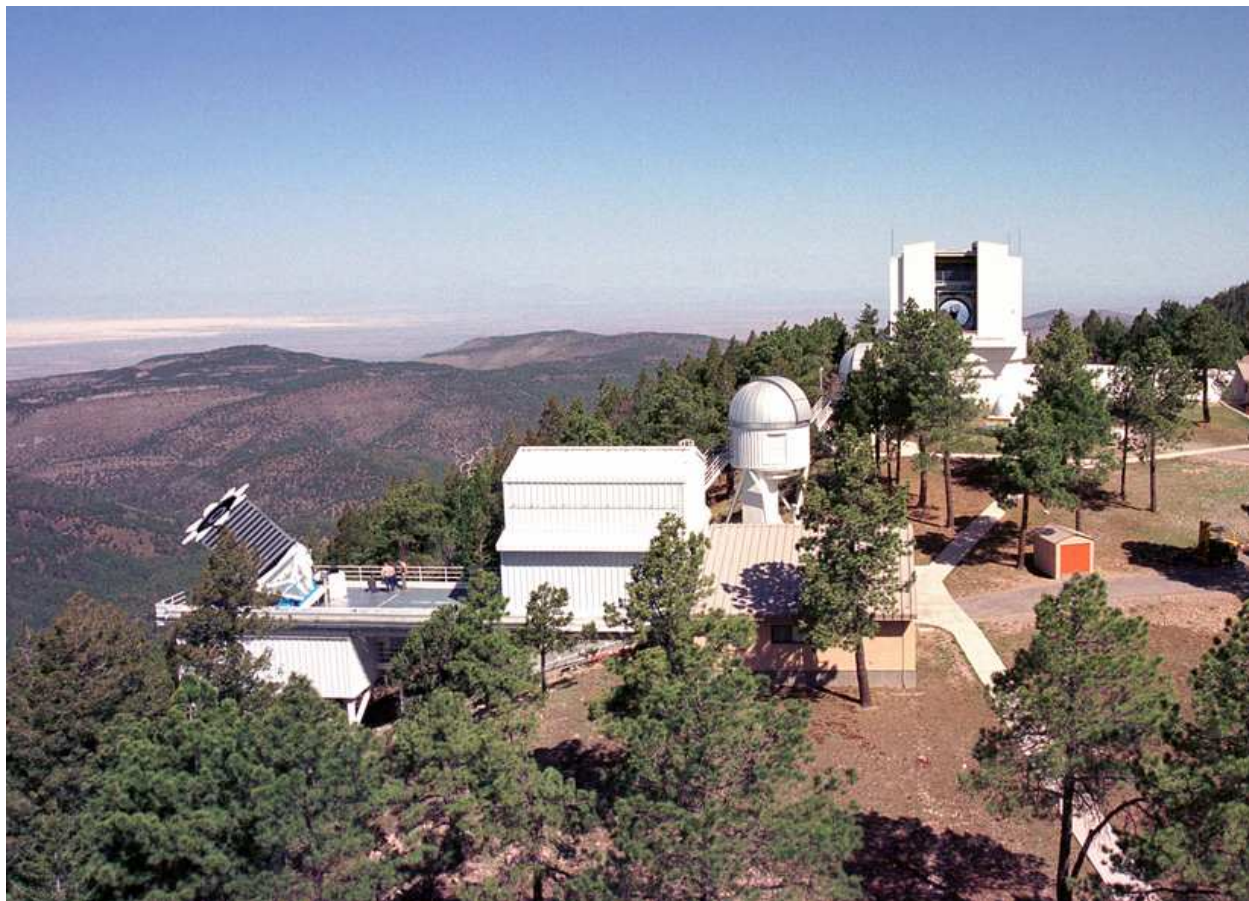
Fig. 1.— Apache Point Observatory, facing north. The SDSS telescope on its west-facing platform is in the foreground. Note the people standing on the platform behind the telescope to get an idea of the scale. The roll-away enclosure is retracted and can be seen on the right. Note the azimuth bearing and the support structure below the platform. The small round dome below the enclosure houses the 0.5 m Photometric Telescope, and the ARC 3.5 m telescope is in the background. White Sands National Monument can be seen to the north-west. with the SDSS telescope in the foreground.
