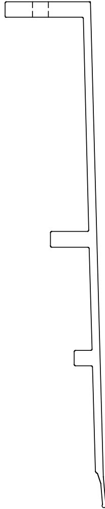
Fig. 20.— Section through the right side of the secondary baffle showing the baffle tip with the vanes that are necessary to interrupt grazing scattered light paths. The baffle tip, machined from aluminum alloy, is 1285 mm in outside diameter and 206 mm high. Above the tip are a series of smaller diameter aluminum annuli each 4.8 mm thick.
