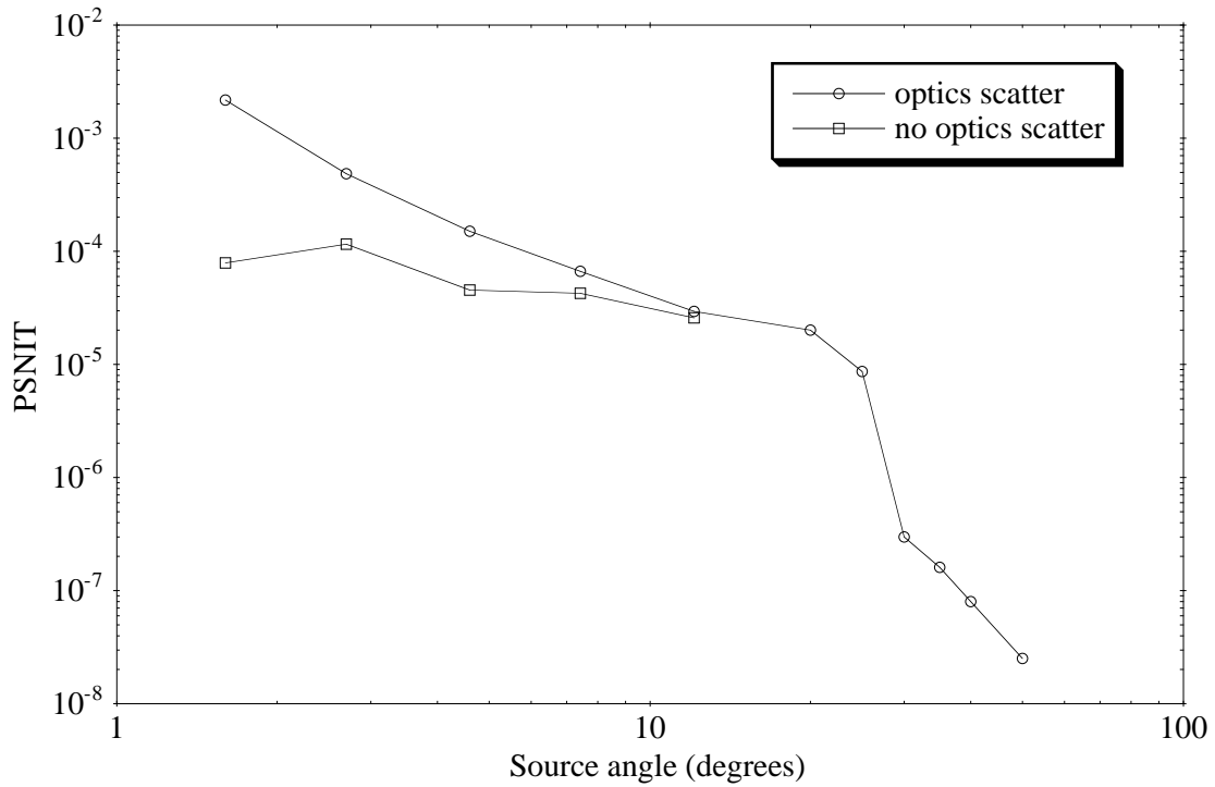
Fig. 16.— Calculated point source normalized irradiance transmission (PSNIT) versus source off-axis angle for the fully baffled SDSS 2.5 m telescope. The two curves for angles less than 20^\circ show the illumination with and without scattering from clean optics. The steep drop at 25^\circ is due to the source moving so far off axis that the aperture stop at the primary mirror is no longer directly illuminated.
