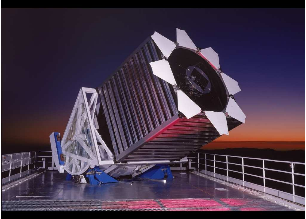
Fig. 2.— The SDSS 2.5 m at sunset, ready for a night's observing. The picture is taken facing west, with the rolled-off telescope enclosure behind the viewer. The telescope is enclosed in its rectangular wind baffle.
