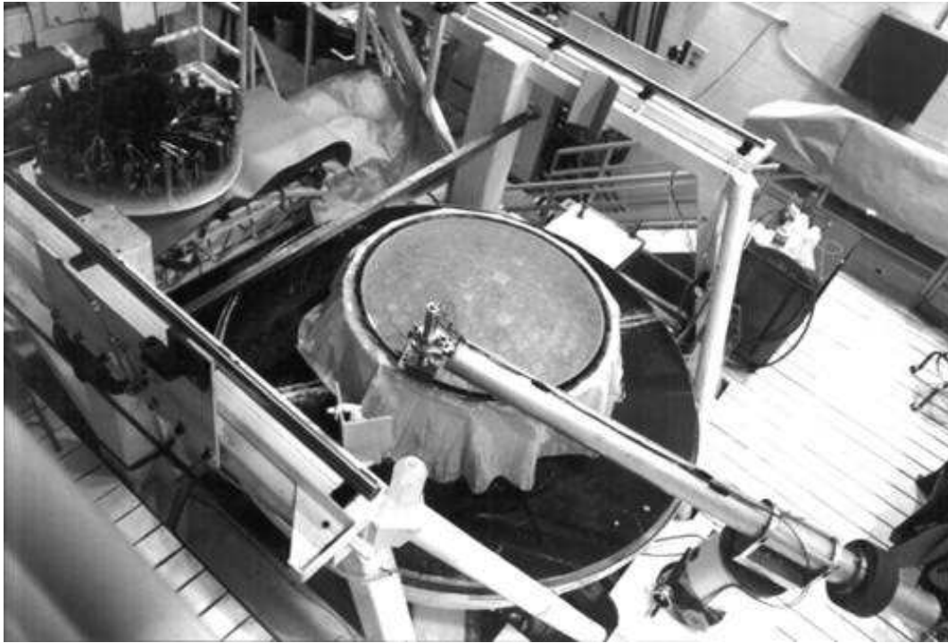
Fig. 9.— The secondary mirror of the SDSS 2.5 m telescope on the polishing turntable at the Steward Observatory Mirror Laboratory. The swing-arm profilometer is seen at the lower right, and the stressed-lap polisher at the upper left.
