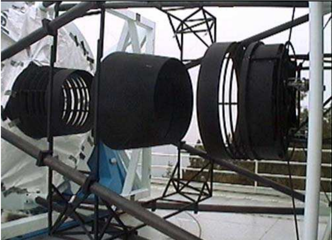
Fig. 22.— The completed internal baffling system installed in the SDSS telescope. From left to right: primary baffle, conical baffle and secondary baffle.
