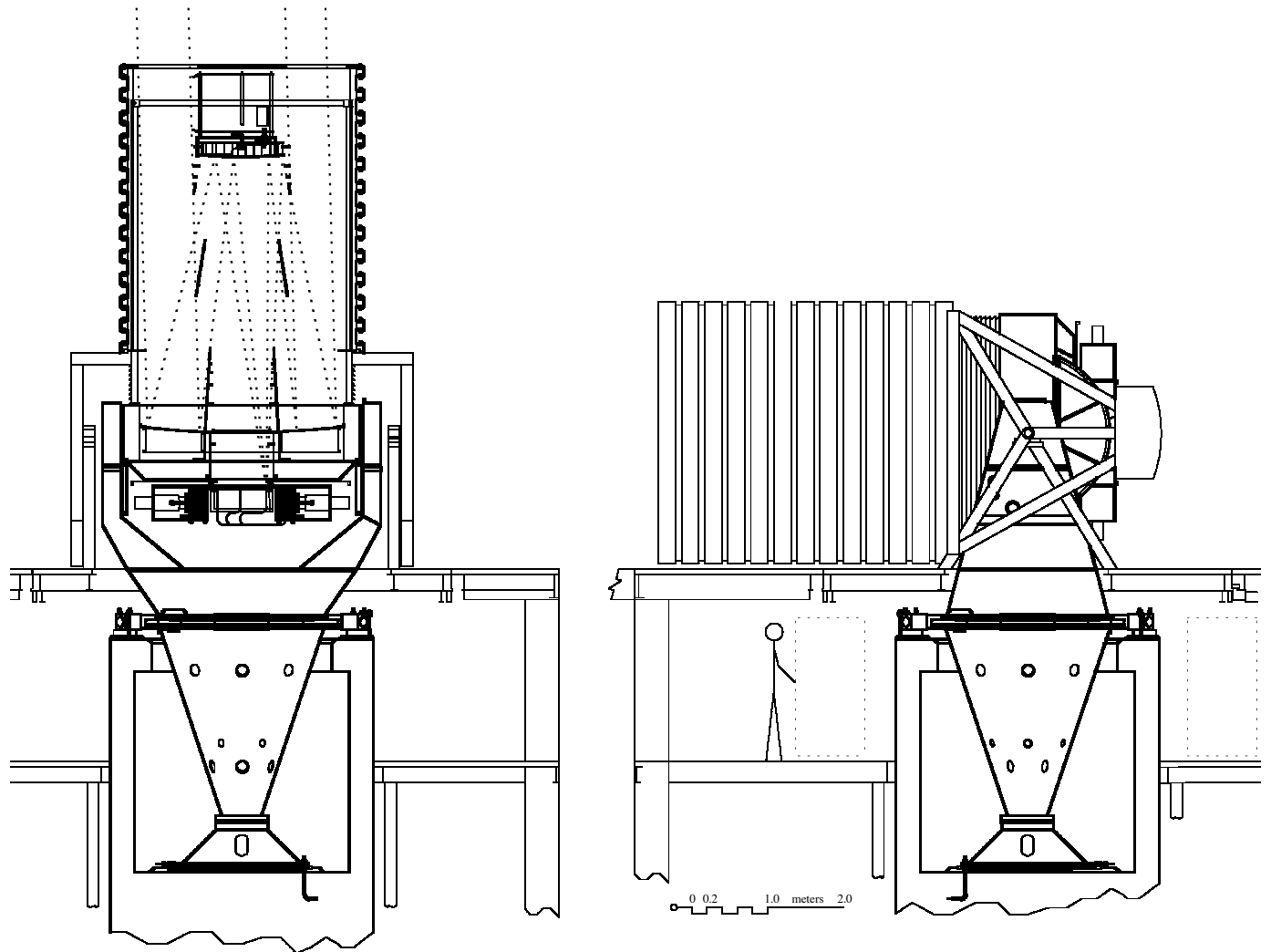
Fig. 12.— Two views of the 2.5-meter telescope. The mechanical design is essentially a scaled version of the WIYN 3.5-m instrument. The wind baffle and the light baffles are shown in relation to rays from the edge of the 3^\circ field of view.
