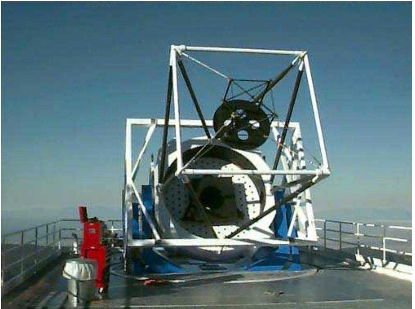
Fig. 13.— The 2.5-m telescope as installed in October, 1995. Centered on the telescope azimuth axis is a circular floor panel that rotates with the telescope. Access to the telescope is along a horizontal ramp from the support building through the telescope enclosure (at the right edge of the photo) which is in its open position. The secondary truss (black) is graphite fiber epoxy, while the secondary frame (white) is steel.
