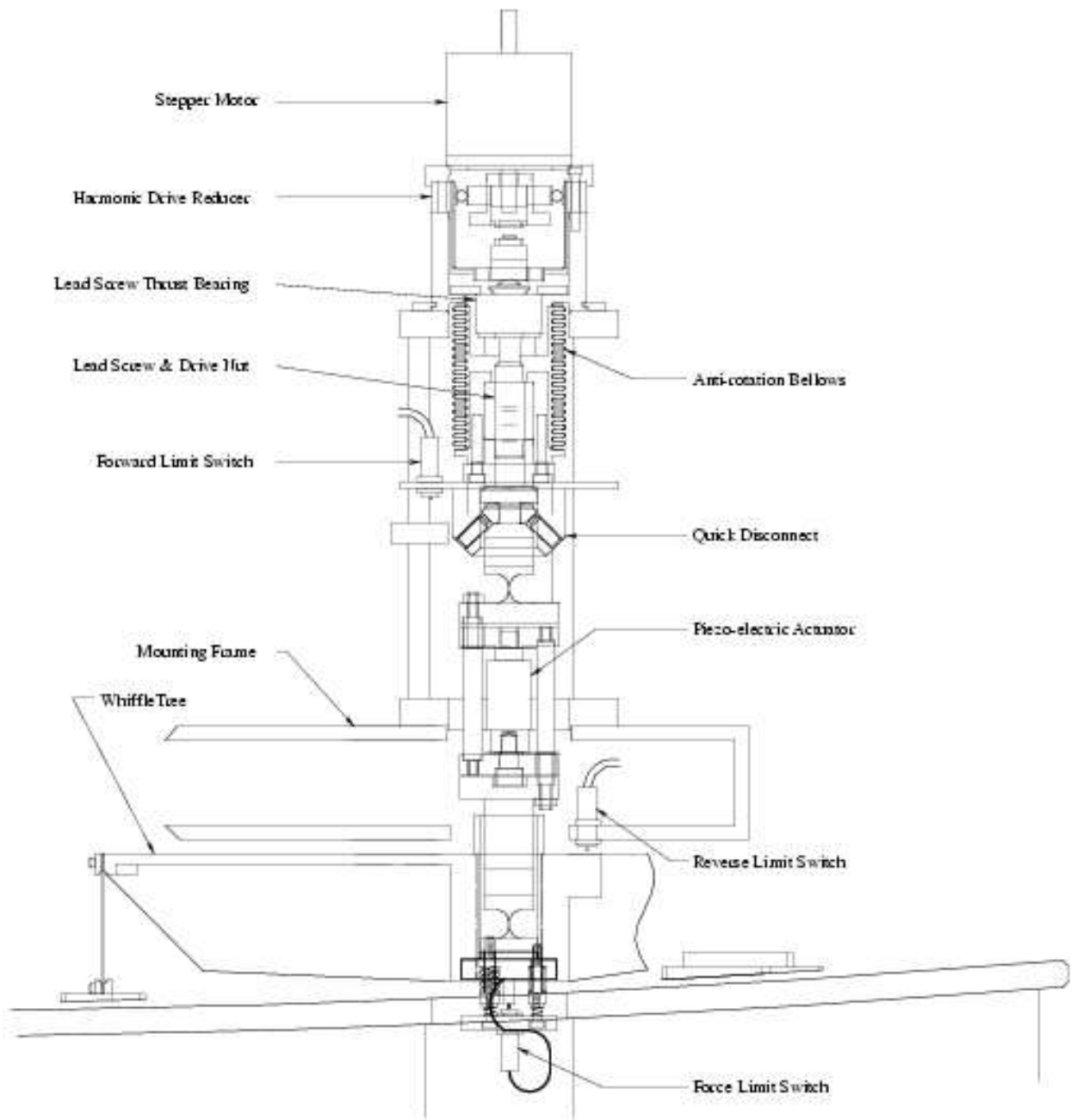
Fig. 15.— Secondary mirror axial actuator assembly
