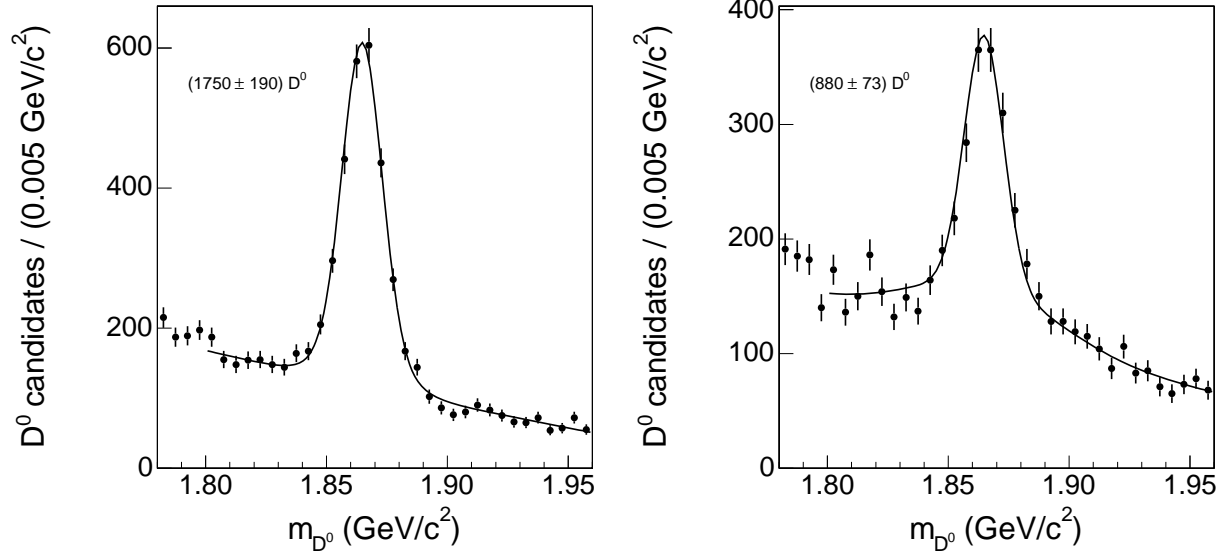
FIG. 23: Invariant mass distribution of D^0 candidates with (left) a kaon or (right) a pion leg identified as a CMUP muon. Solid lines represent the fits described in the text.
