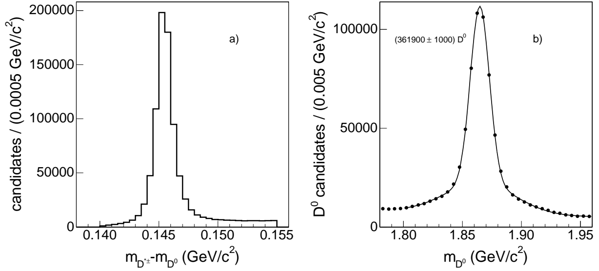
FIG. 22: Distributions of (a) m_{D^{*\pm}} - m_{D^0} and (b) the invariant mass of D^0 candidates (the solid line represents the fit described in the text).
