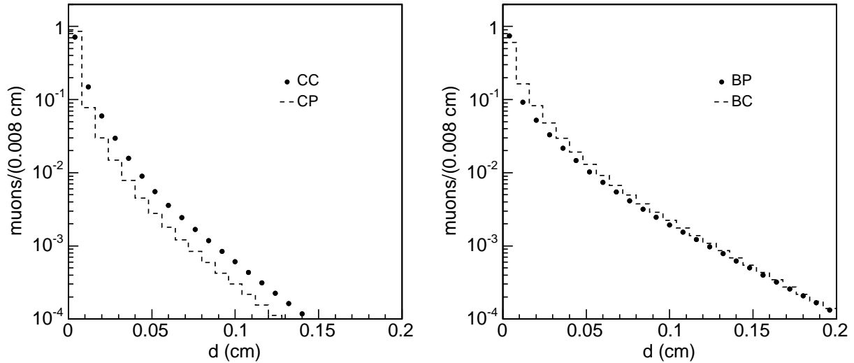
FIG. 3: Projections of the two-dimensional impact parameter distributions of some components used to fit the dimuon data (see text).
