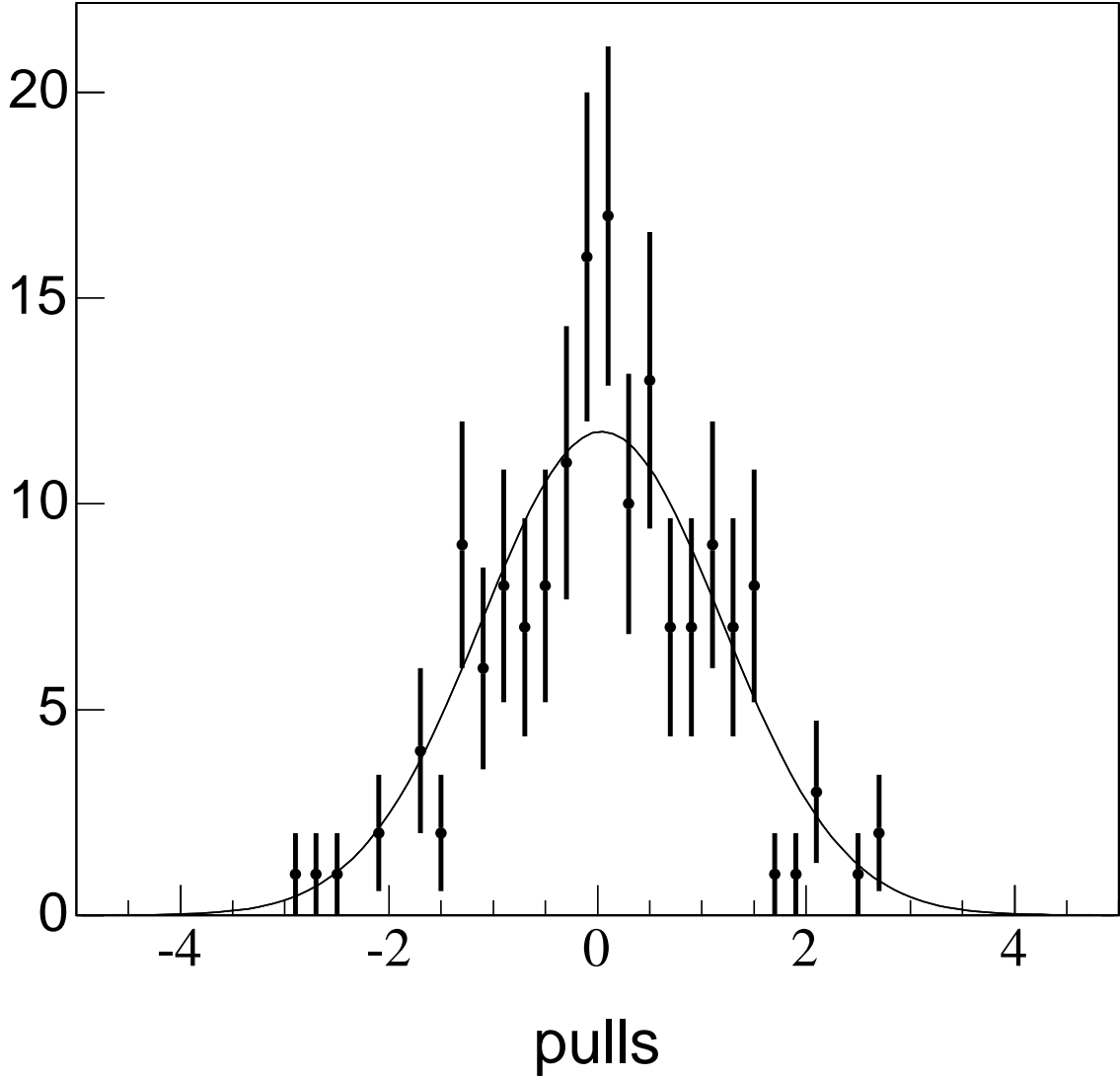
FIG. 7: Distribution of the pulls - (\text{data}-\text{fit})/\sqrt{\text{fit}} - of the fit listed in Table I for the impact parameter bins with at least 10 entries. The solid line represents a Gaussian distribution with unit RMS.
