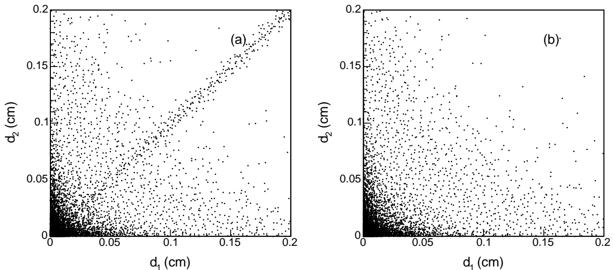
FIG. 4: Two-dimensional impact parameter distributions of muon pairs (a) before and (b) after cosmic removal.
