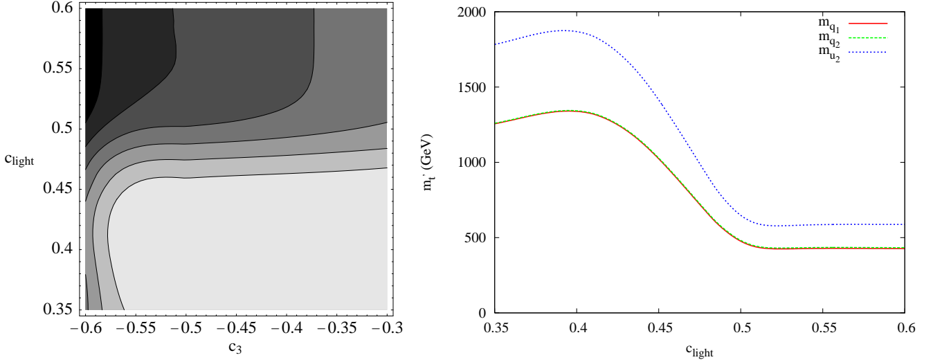
FIG. 5: Mass of the first level quarks of the third generation for the model of Section IV and a \tilde{k} that saturates the bound, assuming c_{RH} = -c_{light} (dotted curve in the right panel of Fig. 2). In the left panel we show the masses of the three degenerate quarks with charges 5/3 , 2/3 and -1/3 as a function of c_3 and c_{light} , for fixed c_1 = 0.2 . The different contours, from dark to light, correspond to m_1 = 500, 600, 750, 1000, 1250 and 1500 GeV, respectively. In the right panel we show the mass of the three lightest quark KK modes with charge 2/3 as a function of c_{light} for fixed c_1 = 0.2 and c_3 = -0.6 .
