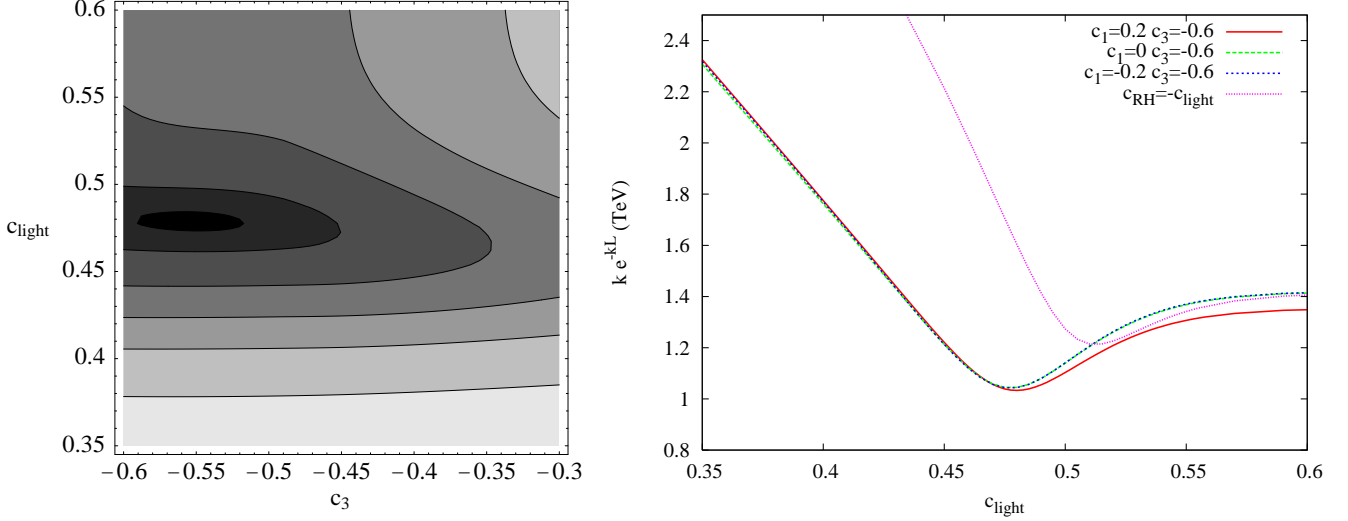
FIG. 2: Lower bound on \tilde{k} = k e^{-kL} as a function of c_3 and c_{\text{light}} for fixed c_1 = 0.2 and c_{\text{RH}} = -0.6 (left panel). The different contours, from dark to light, correspond to \tilde{k} = 1030, 1100, 1300, 1500, 1700 and 2000 GeV, respectively. The minimum is \tilde{k}_{\text{min}} = 1 TeV, corresponding to c_3 \approx -0.55 and c_{\text{light}} \approx 0.48 . In the right panel we show the lower bound on \tilde{k} as a function of c_{\text{light}} for fixed c_{\text{RH}} = c_3 = -0.6 and three values of c_1 . We also show the lower bound on \tilde{k} for c_1 = 0.2 and c_3 = -0.6 , assuming c_{\text{RH}} = -c_{\text{light}} . The mass of the first gauge KK modes is m_1^{\text{gauge}} \approx 2.5 \tilde{k} .
