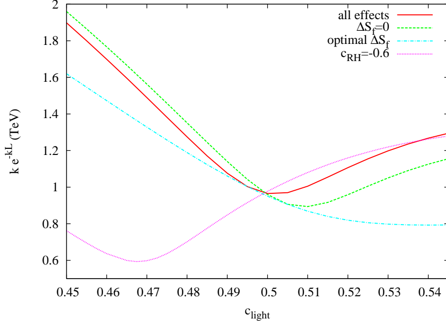
FIG. 4: Lower bound on \tilde{k} = k e^{-kL} as a function of c_{\text{light}} = -c_{\text{RH}} when the light generations arise from doublets of SU(2)_L or SU(2)_R , including all effects (solid line), setting the one-loop contributions to \Delta S_f to zero (dashed line), and choosing values of \Delta S_f that minimize the \chi^2 for each value of the parameters (dash-dotted line). We also show the lower bound on \tilde{k} when the right-handed light fermions are localized at c_{\text{RH}} = -0.6 (near the UV brane), as a function of the localization parameter for left-handed light fermions, c_{\text{light}} (dotted line). In all cases we have fixed c_1 = 0.2 and c_3 = -0.6 .
