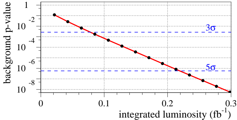
Figure 14: p -values as a function of integrated luminosity \mathcal{L} . The black dots on the line show hypothetical integral numbers of observed events, starting at N = 1 for \mathcal{L} = 0.02 fb ^{-1} .
