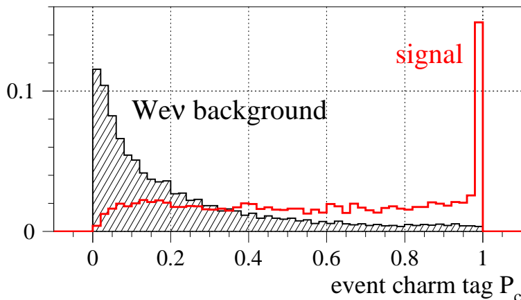
Figure 7: Event charm probability, P_c = F_1^{(e)} \times F_2^{(e)} , comparing signal and the W\bar{e}\nu background. Our requirement is P_c > 0.6 . These distributions are normalized to unit area.
