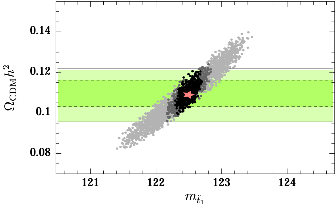
Figure 13: Computation of dark matter relic abundance \Omega_{\text{CDM}}h^2 taking into account estimated experimental errors for stop, chargino, neutralino and Higgs sector measurements at future colliders. The dots correspond to a scan over the 1\sigma ( \Delta\chi^2 \leq 1 ) region allowed by the experimental errors, as a function of the measured stop mass, for a mass measurement error of 1.2 GeV (light gray dots), 0.42 GeV (dark gray dots) and 0.24 GeV (black dots). The underlying scenario used as input is indicated by the red (light) star. The horizontal shaded bands show the 1\sigma and 2\sigma constraints on the relic density measured by WMAP.
