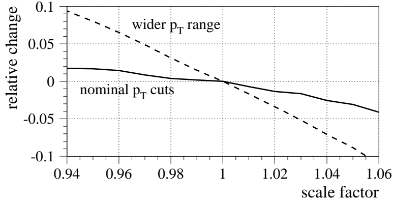
Figure 10: Relative variation of the ratio of efficiencies ( \epsilon_{\text{pk}}/\epsilon_{\text{th}} ) with an overall energy scale factor. The solid line shows a very small variation, given our nominal cuts on p_T , to be compared to a much larger variation if we had used looser p_T cuts meant to maximize the efficiency.
