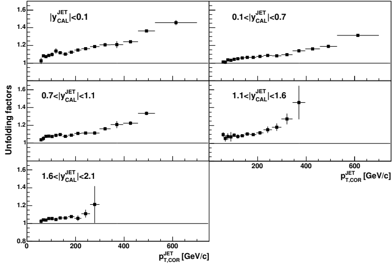
FIG. 6: Unfolding factors, U(p_{T,\text{cor}}^{\text{jet}}, y_{\text{cal}}^{\text{jet}}) , as extracted from PYTHIA TUNE A simulated event samples, as a function of p_{T,\text{cor}}^{\text{jet}} in the different |y_{\text{cal}}^{\text{jet}}| regions.
