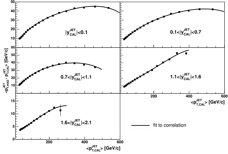
FIG. 5: Correlation \langle p_{T,\text{had}}^{\text{jet}} - p_{T,\text{cal}}^{\text{jet}} \rangle versus \langle p_{T,\text{cal}}^{\text{jet}} \rangle , as extracted from PYTHIA TUNE A simulated event samples, in the different |y_{\text{cal}}^{\text{jet}}| regions.
