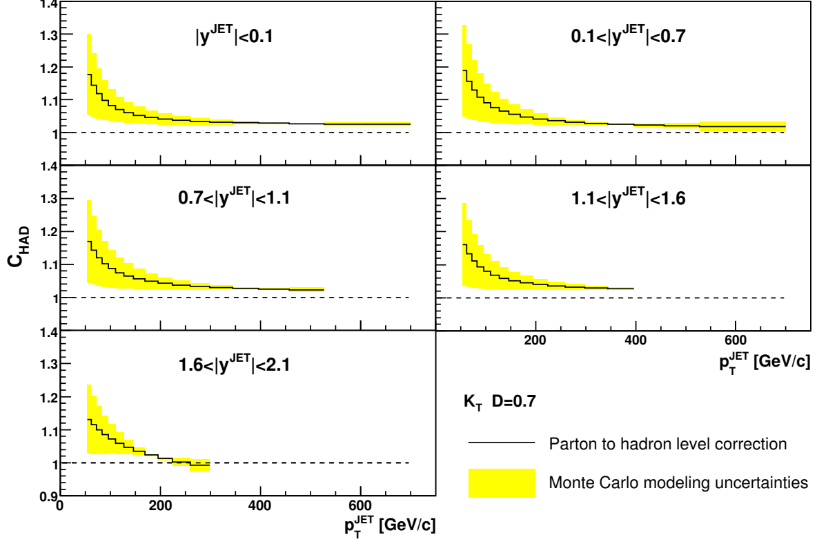
FIG. 8: Magnitude of the parton-to-hadron correction, C_{\text{HAD}}(p_{\text{T}}^{\text{jet}}, y^{\text{jet}}) , used to correct the NLO pQCD predictions (see Tables IV-V). The shaded bands indicate the quoted Monte Carlo modeling uncertainty.
