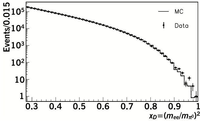
FIG. 2: Dalitz x_D \equiv (m_{e^+e^-}/m_{\pi^0})^2 for fully-reconstructed Dalitz decay candidates after normalization mode analysis cuts. Monte Carlo prediction using the world average form factor slope parameter is overlaid.
