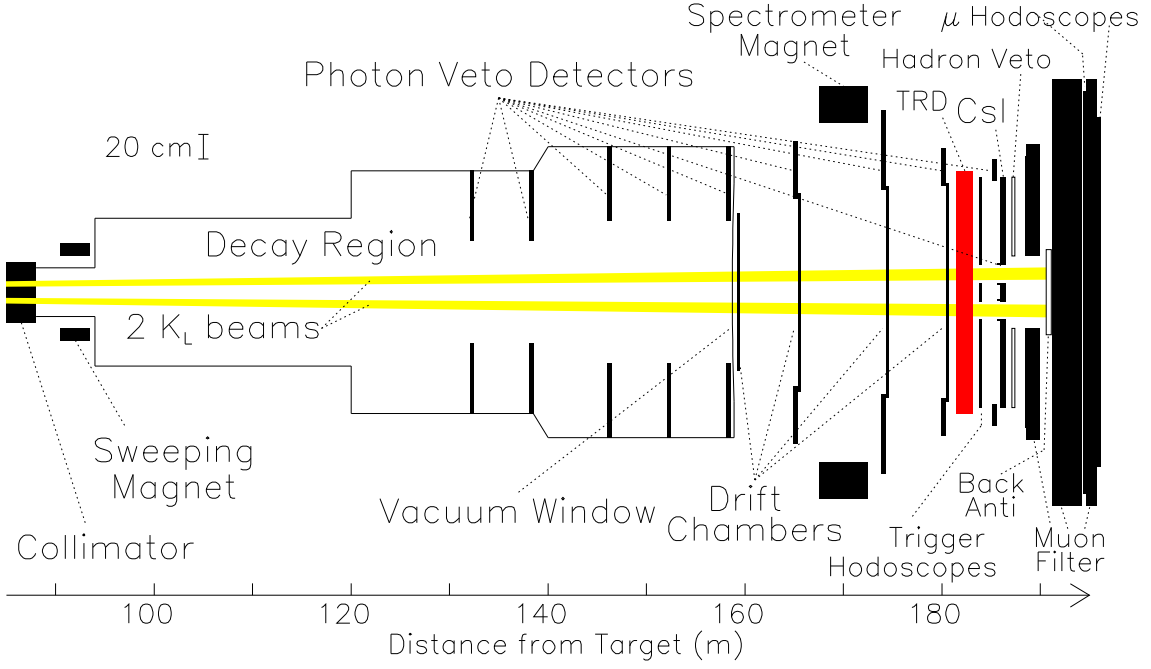
FIG. 1: The KTeV spectrometer in E799-II configuration.
