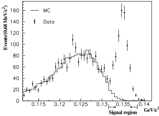
FIG. 3: Positron-electron invariant mass for \pi^0 \rightarrow e^+e^- signal candidates passing all other cuts. The points with error bars are data; the solid histogram is background MC.
