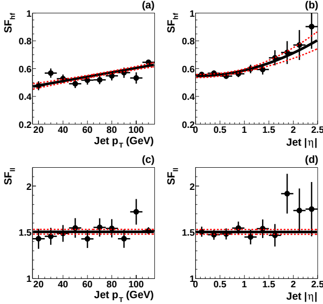
FIG. 10: Correction factors for the contribution of heavy flavor in the negative tag rate ( SF_{hf} ) as functions of (a) jet p_T and (b) jet |\eta| and contribution to the mistag rate from long lived particles ( SF_{ll} ) as functions of (c) jet p_T and (d) jet |\eta| . The resulting fits are shown as solid lines, and the \pm 1\sigma statistical uncertainties are shown as dotted lines.
