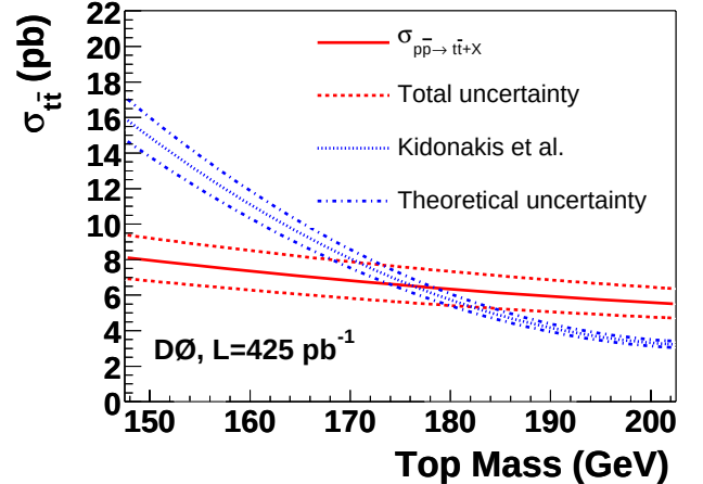
FIG. 13: Top quark mass dependence of the measured cross section compared to the theoretical prediction [6].
