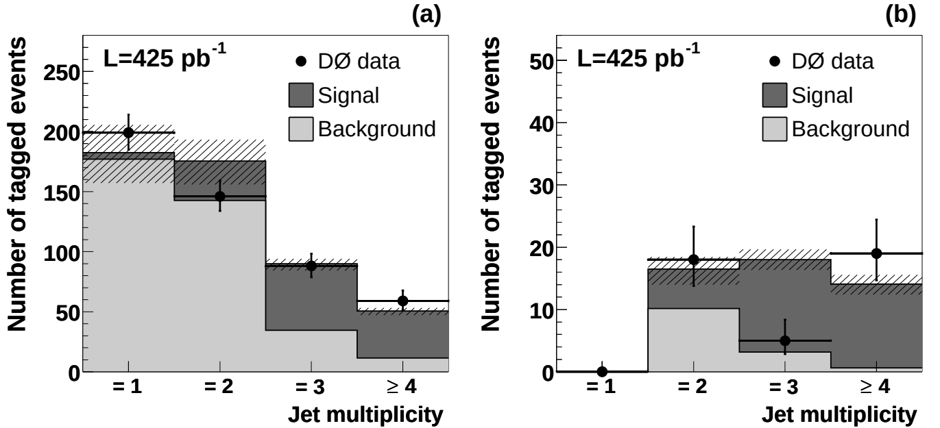
FIG. 12: Observed number of tagged events in data compared to the total SM prediction for (a) single tagged events and (b) double tagged events. The number of t\bar{t} events shown is calculated assuming a cross section of 6.6 pb. The total uncertainty is represented by the hatched band.
