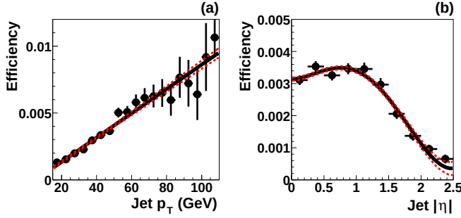
FIG. 9: Negative tagging efficiency vs. (a) jet p_T and (b) jet |\eta| . The resulting fit is shown as a solid line, and the \pm 1\sigma statistical uncertainty is shown as dotted lines.
