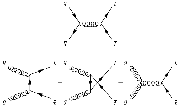
FIG. 1: Leading order Feynman diagrams for the production of t\bar{t} pairs at the Tevatron.
