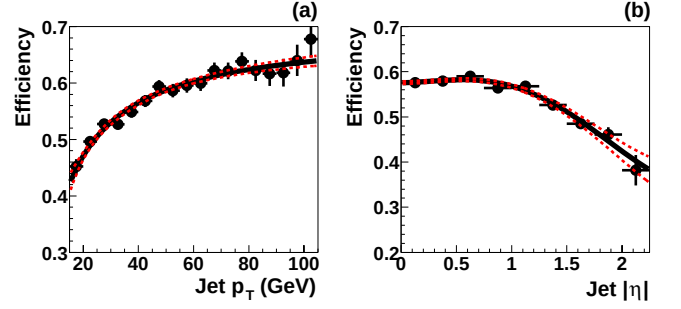
FIG. 7: Semileptonic b tagging efficiency vs. (a) jet p_T and (b) jet |\eta| measured in a b\bar{b} MC sample. The resulting fit is shown as a solid line, and the \pm 1\sigma statistical uncertainty is shown as dotted lines.
