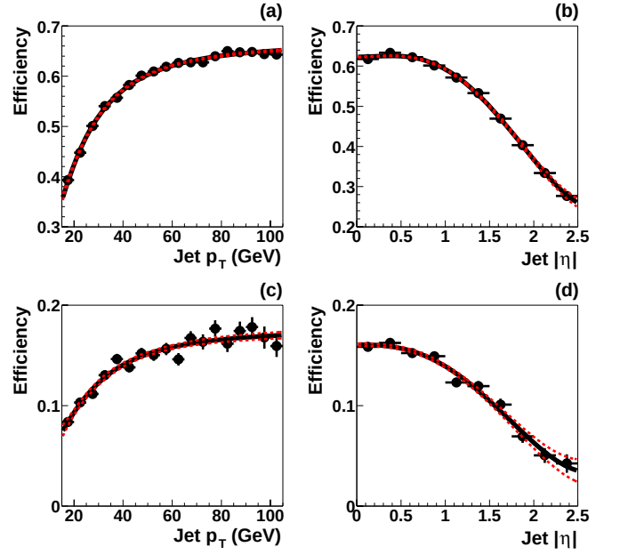
FIG. 8: Inclusive b tagging efficiency vs. (a) jet p_T and (b) jet |\eta| and inclusive c tagging efficiency vs. (c) jet p_T and (d) jet |\eta| . The resulting fit is shown as a solid line, and the \pm 1\sigma statistical uncertainty is shown as dotted lines.
