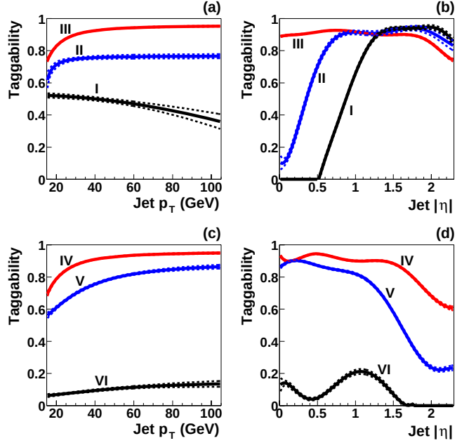
FIG. 3: Taggability vs. jet p_T and |\eta| for PV_z \times \eta < 0 [(a) and (b) respectively] and PV_z \times \eta > 0 [(c) and (d) respectively]. The central value is shown with a solid line, and the \pm 1\sigma statistical uncertainty is shown as dotted lines. The labels I–VI correspond to the regions of \text{sign}(PV_z \times \eta) \times |PV_z| defined in Fig. 2.
