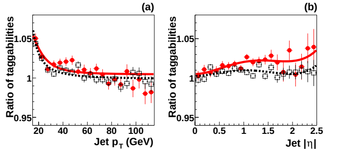
FIG. 4: Ratio of the b to light (full circles) and c to light (open squares) quark jet taggability, measured in a QCD MC sample as functions of (a) jet p_T and (b) jet |\eta| . The resulting fits used in the analysis are also shown.
