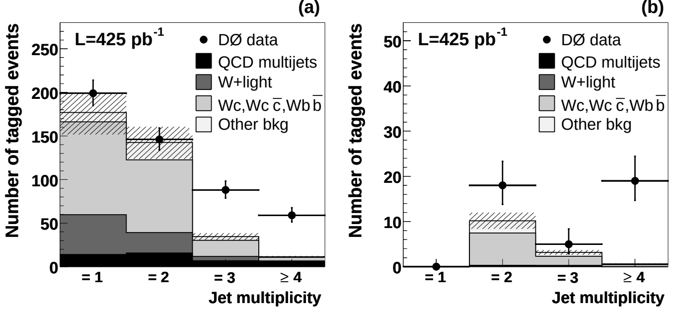
FIG. 11: Observed number of tagged events in data compared to the total SM background predictions (excluding t\bar{t} ) for (a) single tagged events and (b) double tagged events. The total uncertainty on the background prediction is represented by the hatched band. The excess of observed events in the third and fourth jet multiplicity bins is attributed to t\bar{t} production.
