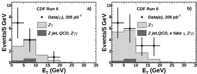
FIG. 3: The distributions in missing transverse energy \cancel{E}_T observed in the inclusive search for a) \mu\mu\gamma events and b) ee\gamma events. The histograms show the expected SM contributions.
