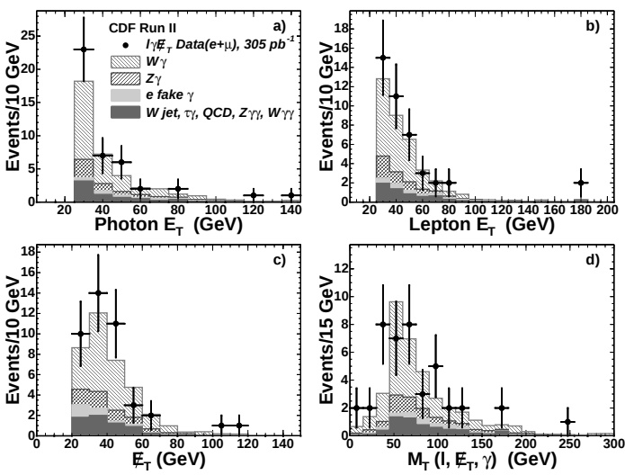
FIG. 1: The distributions for events in the \ell\gamma\cancel{E}_T sample (points) in a) the E_T of the photon; b) the E_T of the lepton; c) the missing transverse energy, \cancel{E}_T ; and d) the transverse mass of the \ell\gamma\cancel{E}_T system. The histograms show the expected SM contributions, including estimated backgrounds from misidentified photons and leptons.
