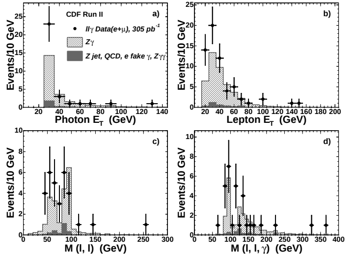
FIG. 2: The distributions for events in the \ell\ell\gamma sample (points) in a) the E_T of the photon; b) the E_T of the leptons (two entries per event); c) the 2-body mass of the dilepton system; and d) the 3-body mass m_{\ell\ell\gamma} . The histograms show the expected SM contributions.
