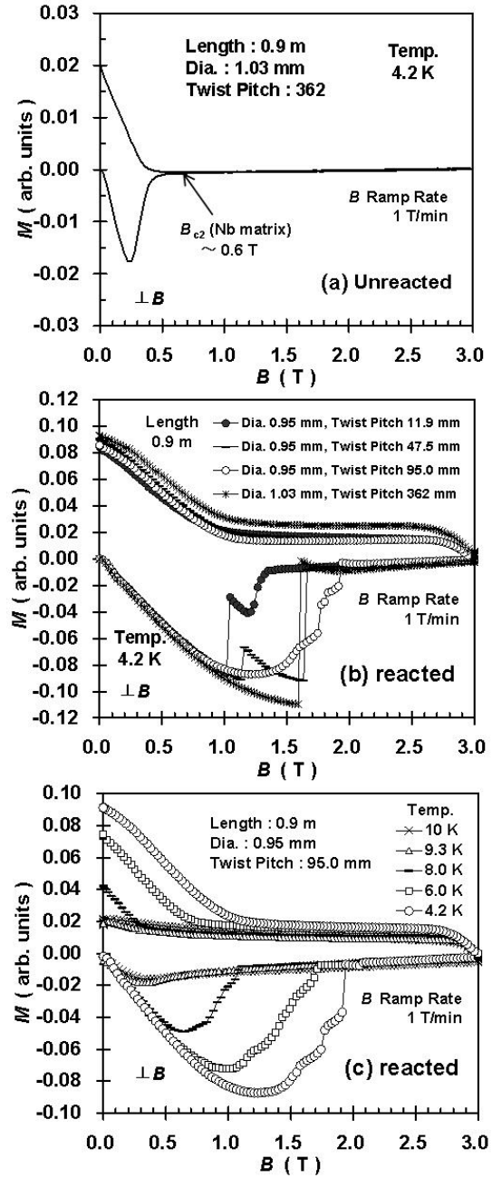
Fig. 6. Magnetization loops measured with the balanced coil magnetometer. Fig. 6a Loop for an unreacted F1 Nb 3 Al strand. Fig. 6b Twist pitch effect of the reacted samples. Fig. 6c. Temperature dependence of the reacted sample.
