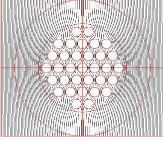
Fig. 5b. Flux line pattern in the Cu stabilized Nb 3 Al strand when the external field is above B_{c2} of Nb, namely above 0.6 Tesla and in a really stationary field. Nb is not superconducting. This is simulated with ANSYS [6].
