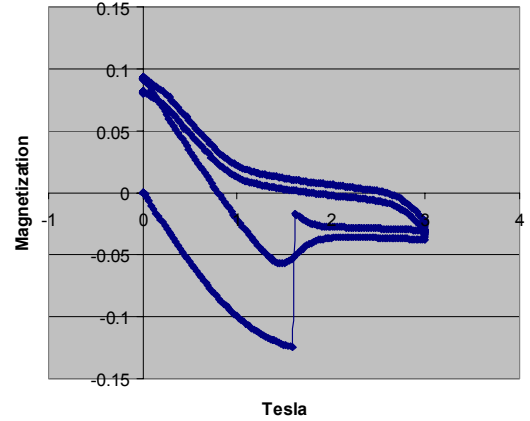
Fig. 4. Magnetization curve observed with a balanced coil magnetometer. Abnormally large magnetization loop and a big flux-jump like step are observed at 1.6 Tesla, which occurs at much higher field than the B_{c2} value (about 0.5 Tesla) of Nb. There is no abnormally big jump in the second loop.
