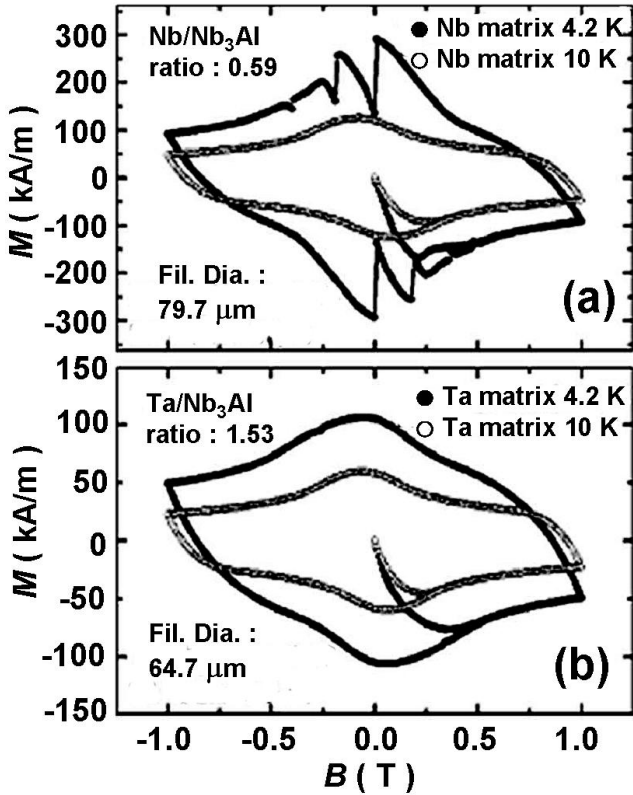
Fig. 3. Magnetization curves of (a) Nb matrix and (b) Ta matrix RHQT \text{Nb}_3\text{Al} strands at 4.2 K and 10 K measured at NIMS with a SQUID magnetometer [4].
