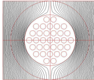
Fig. 5a. Flux line pattern in the Cu stabilized \text{Nb}_3\text{Al} strand, when the Nb is superconducting in a low external field. This is simulated with ANSYS [6].
