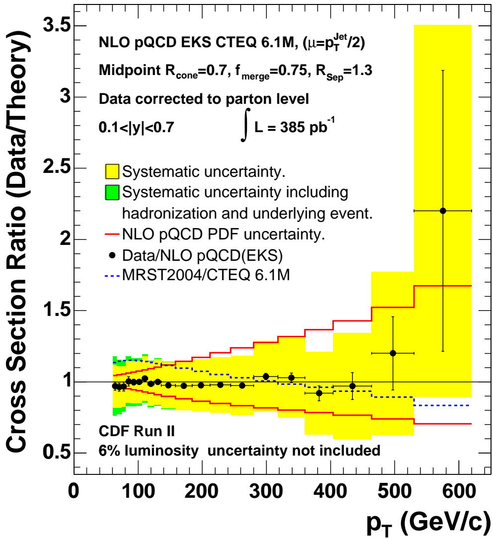
FIG. 2: The ratio of the data corrected to the parton level over the NLO pQCD prediction of the EKS calculation using CTEQ6.1M. Also shown are the experimental systematic errors and the theoretical errors from the PDF uncertainty. The ratio of MRST2004/CTEQ6.1M is shown as the dashed line. An additional 6% uncertainty on the determination of the luminosity is not shown.
