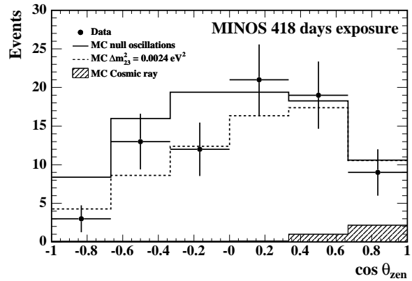
FIG. 10: The reconstructed \cos \theta_{\text{zen}} distribution for the 77 selected events with good timing compared to the MC expectation. The solid histogram shows the MC expectation for the case of no neutrino oscillations, the hatched histogram shows the cosmic-ray background and the points with error bars show the data. The dashed histogram shows the expectation for \nu_\mu \leftrightarrow \nu_\tau oscillations with \sin^2 2\theta_{23} = 1.0 and \Delta m_{23}^2 = 0.0024 \text{ eV}^2 .
