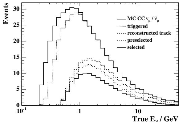
FIG. 7: The expected number of CC \nu_{\mu}/\bar{\nu}_{\mu} events that interact within the detector fiducial volume at the different stages in the selection (418 days exposure). In addition to the expected energy distribution before selection and the final selected distribution, the expected numbers of events are shown at several stages in the analysis: events which pass the trigger requirements; events for which there is a reconstructed track; and events which pass the preselection cuts.
