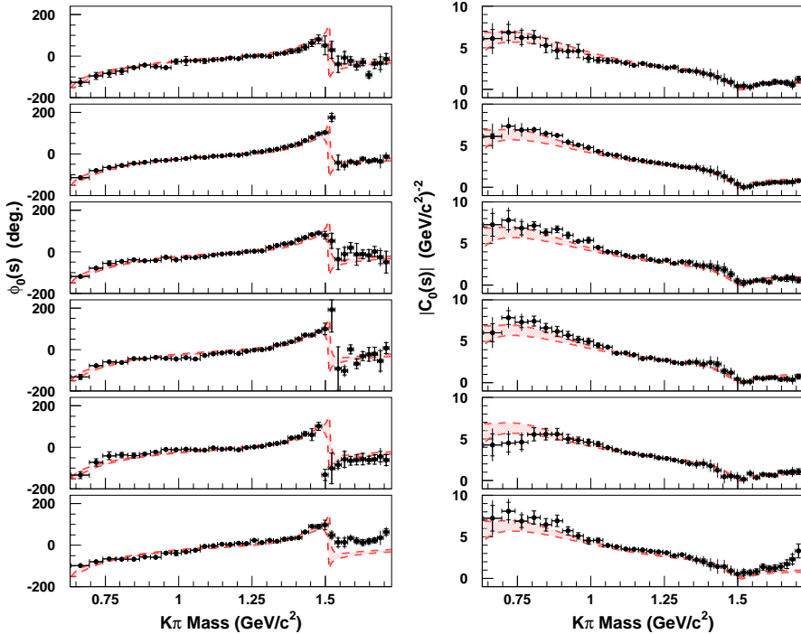
FIG. 8: Comparison between fitted S -wave amplitudes (solid circles with error bars representing statistical uncertainties) and generated amplitudes, represented as shaded regions between dashed curves computed as described in Sec. V. Generated curves follow the isobar fit model described in Sec. V. The figure shows results from the first six (of 100) samples used in the test.
