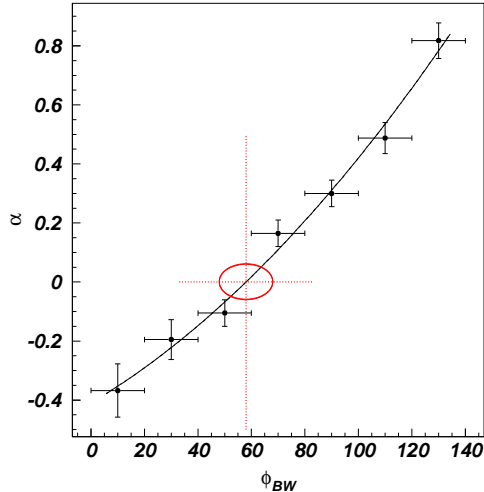
FIG. 2: The asymmetry \alpha plotted vs. BW phase \phi_{BW} for the K^*(892) . These quantities are described in the text. \alpha becomes zero at \phi_{BW} \sim 56 degrees.
