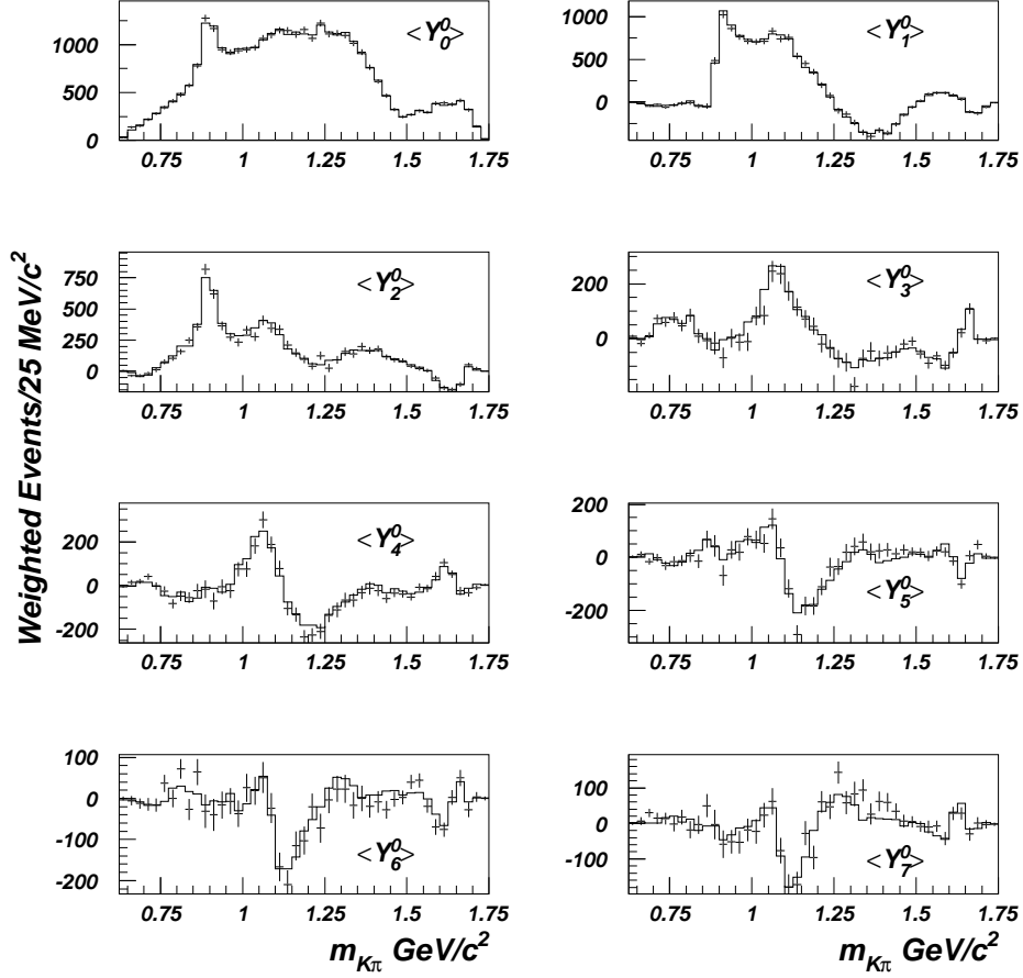
FIG. 5: Moments of the K^- \pi^+ helicity angle \theta for the MIPWA fit. In each figure, events are plotted in bins of K^- \pi^+ invariant mass with weights equal to P_L(\cos \theta) as indicated. Two combinations are plotted for each K^- \pi^+ \pi^+ candidate. Data are represented as points with error bars. Events are not weighted for their estimated efficiency. The MC events, treated the same way, are used to show the expectation for these moments from the fit, and are shown as solid histograms.
