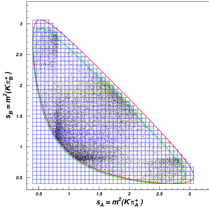
FIG. 1: Dalitz plot for D^+ \rightarrow K^- \pi_A^+ \pi_B^+ decays. The squared invariant mass s_B of one K^- \pi^+ combination is plotted against s_A , the squared invariant mass of the other combination. The plot is symmetrized, each event appearing twice. Lines in both directions indicate values equally spaced in squared effective mass at each of which the S -wave amplitude is determined by the MIPWA described in section III. Kinematic boundaries for the Dalitz plot are drawn for three-body mass values M = 1.810 and M = 1.890 \text{ GeV}/c^2 , between which data are selected for the fits.
