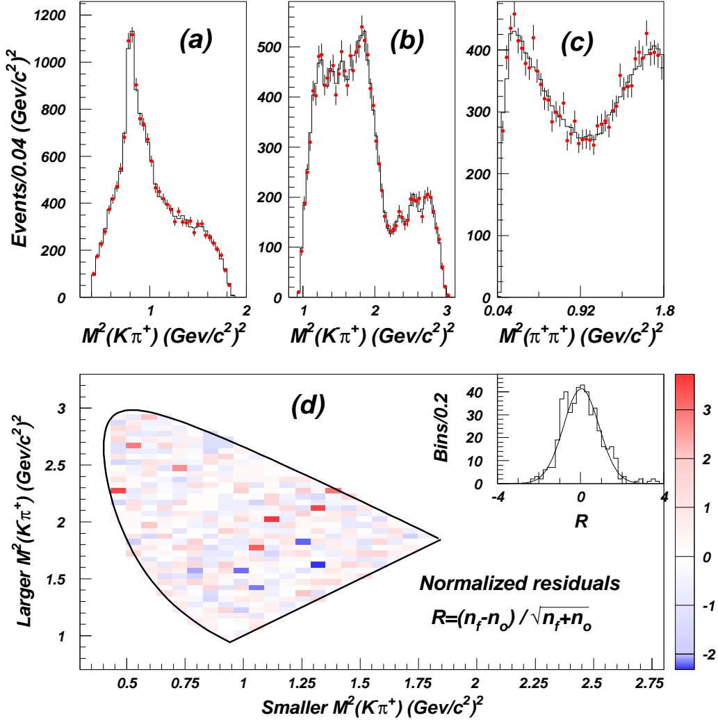
FIG. 4: Comparison between MIPWA fit and data for D^+ \rightarrow K^-\pi^+\pi^+ decays. For each event, the distributions of (a) the smaller K^-\pi^+ , (b) the larger K^-\pi^+ and (c) the \pi^+\pi^+ squared invariant masses are plotted as points with error bars. Results of the fit (solid histogram) are superimposed. (d) The Dalitz plot folded about the axis of symmetry resulting from the identity of the two \pi^+ mesons. The quantity plotted is the normalized residual (n_f - n_o)/\sqrt{n_f + n_o} defined in the text. The histogram is the distribution of normalized residual values and the curve is a Gaussian fit to this having mean -0.015 \pm 0.039 and standard deviation 0.93 \pm 0.04 .
