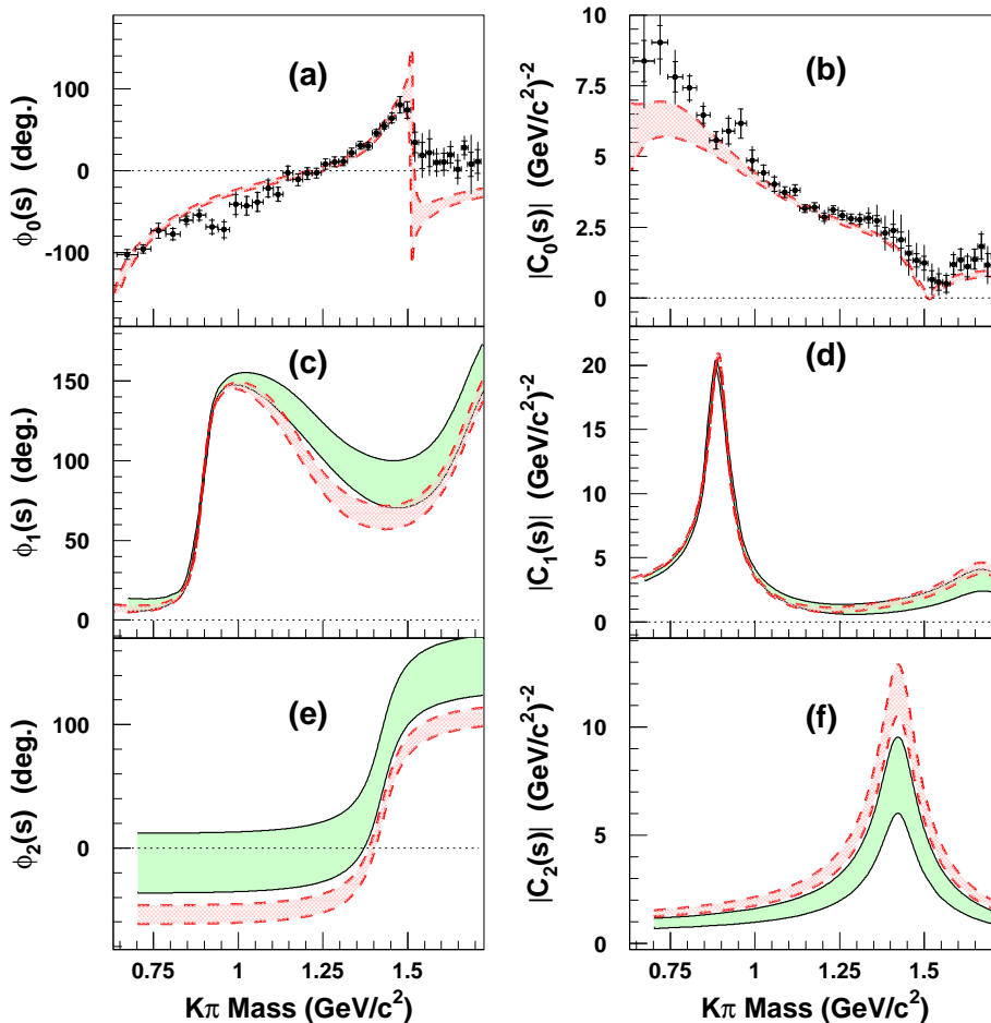
FIG. 3: (a) Phases \gamma_k = \phi_0(s_k) and (b) magnitudes c_k = |C_0(s_k)| of S -wave amplitudes for K^- \pi^+ systems from D^+ \rightarrow K^- \pi^+ \pi^+ decays with the amplitude and phase of the K^*(892) as reference. Solid circles, with error bars show the values obtained from the MIPWA fit described in the text. The effect of adding systematic uncertainties in quadrature is indicated by extensions on the error bars. The P -wave and D -wave phases are plotted in (c) and (e) and their magnitudes in (d) and (f), respectively. These curves are derived from Eqs. (7) and (8), respectively, evaluated with the parameters and error matrix resulting from the MIPWA. Curves appear as shaded areas representing one standard deviation limits for these quantities. In all plots, the dashed curves show one standard deviation limits for the predictions of the isobar model fit described in Sec. V. These curves are computed in the same way, using Eq. (17) in addition to (7) and (8) with parameters and error matrix from the isobar model fit.
