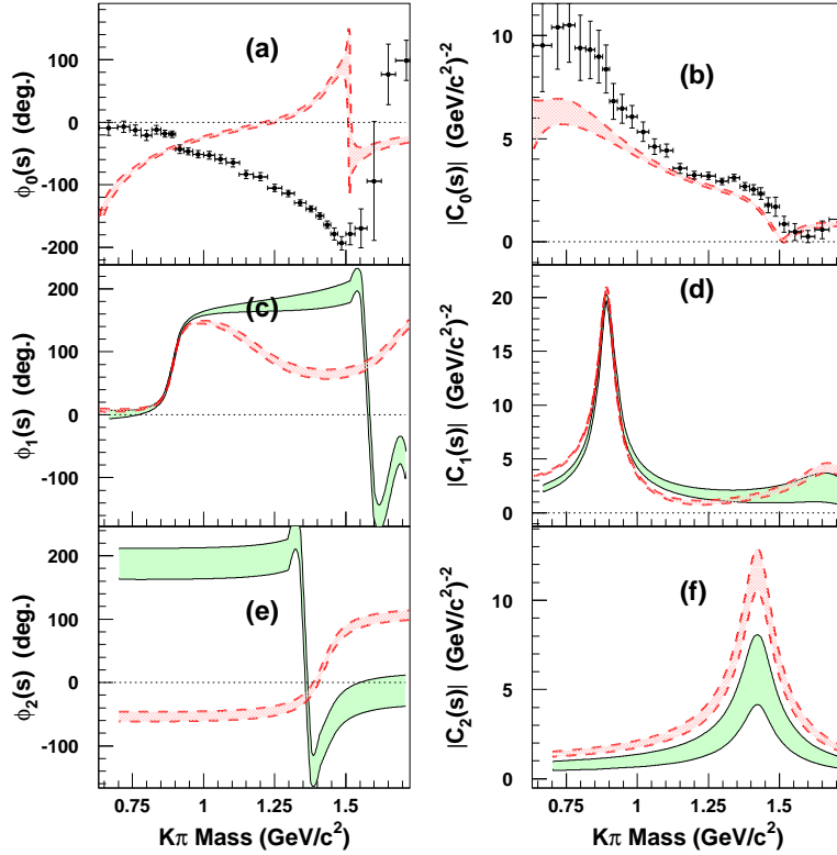
FIG. 9: A second solution for the S -wave amplitude from MIPWA fits to D^+ \rightarrow K^- \pi^+ \pi^+ decays with P - and D -wave parametrized by the \kappa model described in the text. Plots show the (a) phase and (b) magnitude for solution B for the S -wave obtained by using different starting values for the amplitudes. The dashed curves delineate the regions that lie within one standard deviation of the isobar model fit described in Sec. V. The P -wave is shown in (c) and (d) and the D -wave in (e) and (f).
