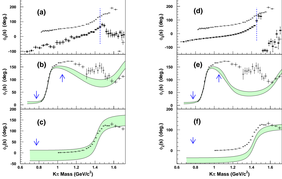
FIG. 6: Plots show comparisons between results obtained from the MIPWA, described in Sec. IV, for phases of the (a) S -wave, (b) P -wave and (c) D -wave K^- \pi^+ scattering amplitudes with measurements made by the LASS collaboration [16]. Solid circles in (a) are the phases \gamma_k obtained at each invariant mass s_k from the MIPWA. The vertical dashed line at the K\eta' threshold ( 1454 \text{ MeV}/c^2 ) indicates the upper limit of the range where K^- \pi^+ scattering is predominantly elastic in the S -wave. Solid curves in (b) and (c) enclose the zones within one standard deviation of the MIPWA P - and D -waves, computed as described in Sec. IV. Arrows indicate the position of the K\pi\pi threshold, at which K^- \pi^+ scattering in the P - and D -waves can become inelastic. In (b) a further arrow at 1050 \text{ MeV}/c^2 indicates the approximate invariant mass at which the P -wave data from Ref. [16] were observed to become inelastic. In (d)-(f) the results from the “elastic fit” are shown in place of those from the MIPWA. In all plots I = \frac{1}{2} measurements from the LASS experiment of phases for K^- \pi^+ scattering in these waves are shown as \times 's with error bars indicating statistical uncertainties.
