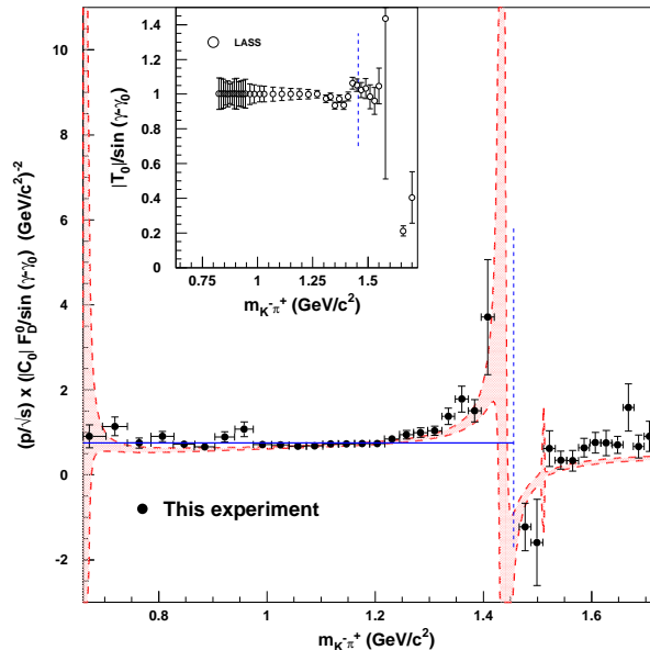
FIG. 7: The quantities p/\sqrt{(s_k)} \times |C_0(s_k)| \times \mathcal{F}_D^0/\sin(\gamma_k - \gamma_0) plotted as solid circles for each point obtained for the S -wave amplitude in the MIPWA fit described in Sec. IV. Three points between 1400 and 1450 \text{MeV}/c^2 are omitted from the plot as their values for \sin(\gamma_k - \gamma_0) are very small. Their values are either off-scale or their errors extremely large. The region between the dashed lines shows the one standard deviation limits of this quantity for the S -wave amplitude obtained from the isobar fit. The inset shows, as small open circles, the quantities |T_0(s)|/\sin(\gamma_B + \gamma_R) taken from the LASS experiment. The K\eta' threshold is indicated by dashed, vertical lines in both plots.
