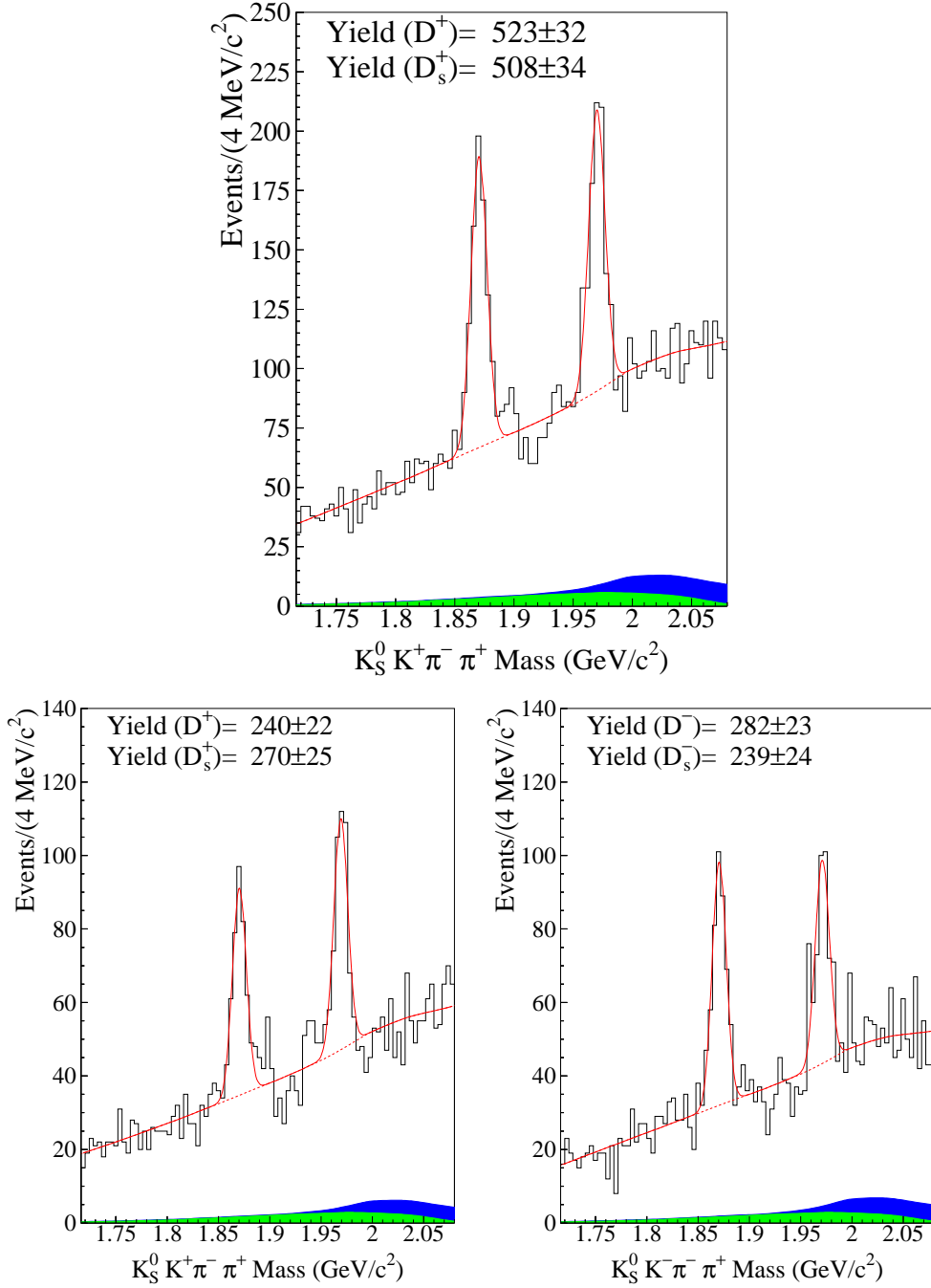
Fig. 4. Upper plot is an invariant mass plots for the state K_S^0 K^\pm \pi^+ \pi^- . Lower plots are invariant mass plots for D^+ \rightarrow K_S^0 K^+ \pi^+ \pi^- (left) and for D^- \rightarrow K_S^0 K^- \pi^+ \pi^- (right). All plots have an L/\sigma > 6 cut. The broad light shaded region is a reflection from \Lambda_c^+ \rightarrow p K_S^0 \pi^- \pi^+ , while the darker shaded region above the D^+ mass results from D^+ \rightarrow K_S^0 \pi^+ \pi^- \pi^+ where one pion is misidentified as a kaon.
