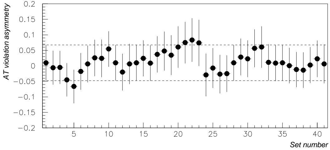
Fig. 3. T -violating asymmetry A_{Tviol} versus several sets of cuts. We varied the confidence level of the secondary vertex from 1% to 5% (5 points), Iso2 from 10^{-6} to 1 (7 points), L/\sigma_L from 5 to 15 (11 points), \Delta_K from 1 to 5 (9 points), p_{icon} from -6 to -2 (9 points). The dashed lines show the quoted A_{Tviol} asymmetry \pm 1\sigma .
