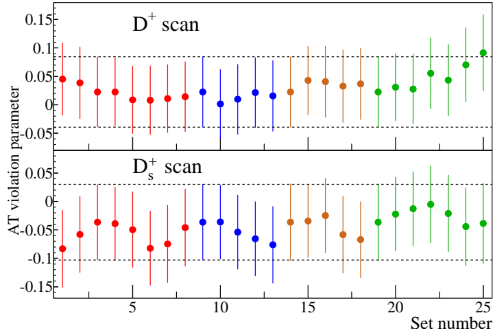
Fig. 6. T -violating asymmetry A_{Tviol} versus several sets of cuts. We varied the \sigma_L from 4 to 12 (8 points), Iso2 from 10^{-2} to 10^{-6} (5 points), confidence level of the secondary vertex from 1% to 5% (5 points), \Delta_K from 2 to 5 (7 points). The dashed lines show the quoted A_{Tviol} asymmetry \pm 1\sigma .
