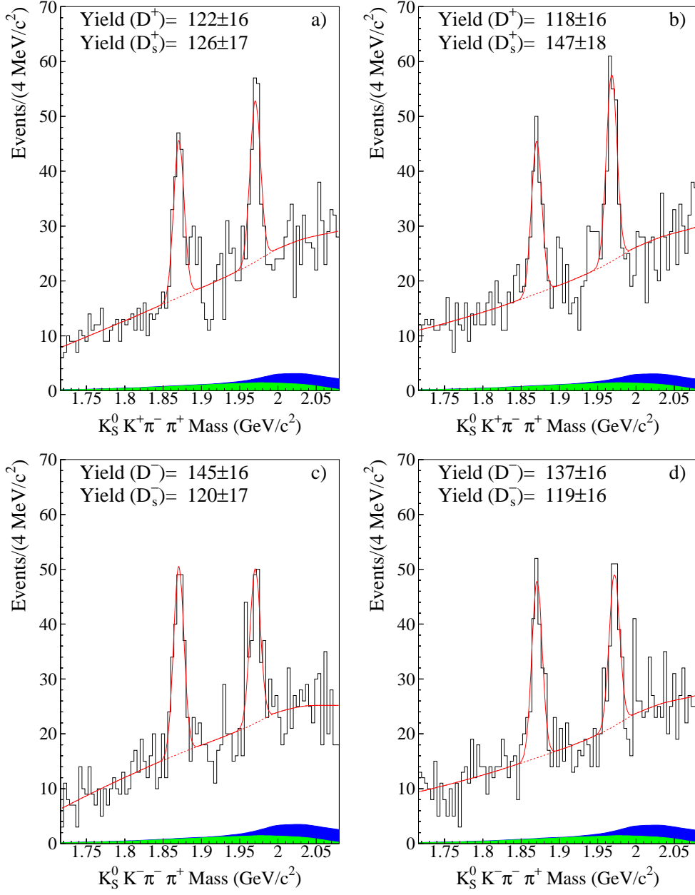
Fig. 5. Upper plots are invariant mass plots for D^+ \rightarrow K_S^0 K^+ \pi^+ \pi^- for C_T > 0 in Fig. 5a and for C_T < 0 in Fig. 5b. Lower plots are invariant mass plots for D^- \rightarrow K_S^0 K^- \pi^+ \pi^- for C_T > 0 in Fig. 5c and for C_T < 0 in Fig. 5d. All plots have an L/\sigma > 6 cut. The shaded regions shown in each plot are explained in the text and in Fig. 4.
