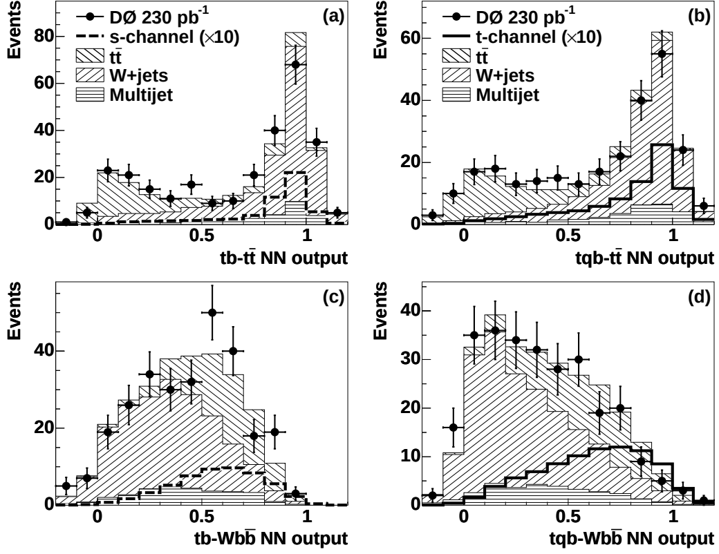
FIG. 3: Comparison of signal, background, and data for the neural network outputs, for the electron and muon channels combined, requiring at least one tag. This figure shows (a) the tb\text{-}\bar{t}\bar{t} filter, (b) the tqb\text{-}\bar{t}\bar{t} filter, (c) the tb\text{-}Wb\bar{b} filter, and (d) the tqb\text{-}Wb\bar{b} filter. Signals are multiplied by ten.
