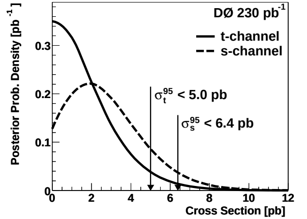
FIG. 4: The Bayesian posterior probability density as a function of the single top quark cross section for the s -channel and t -channel searches.
