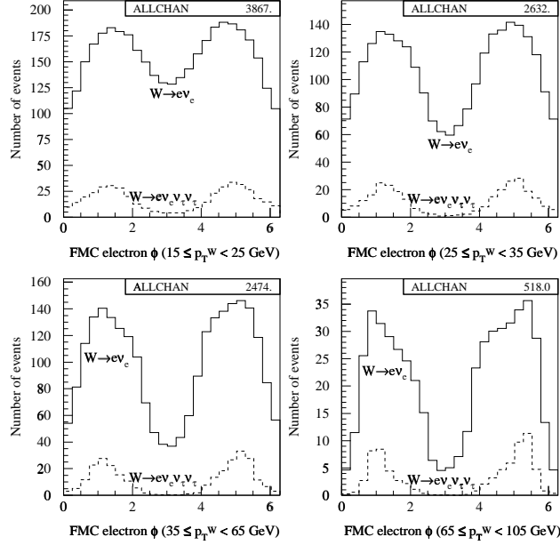
FIG. 11: Electron \phi distributions for the four p_T^W bins for electron W +jet FMC events (solid histogram) and for tau W +jet FMC background (multiplied by 5), where the tau decays to an electron (dashed histogram). The histograms are normalized to the FMC signal event yields.
