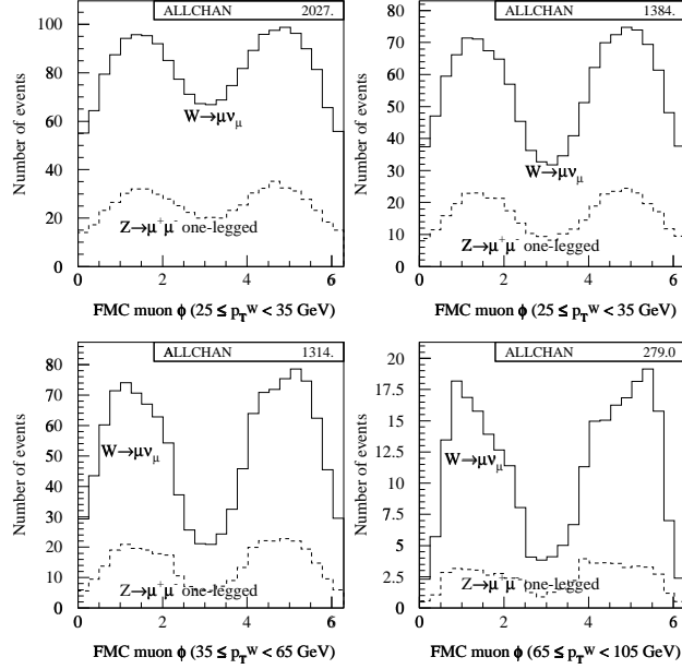
FIG. 10: Muon \phi distributions for the four p_T^W bins for muon W +jet FMC events (solid histogram) and for Z +jet FMC background (multiplied by 5), where one of the muons from the Z decay is undetected and the other one passes the detection and analysis requirements (dashed histogram). The histograms are normalized to the muon FMC signal event yields.
