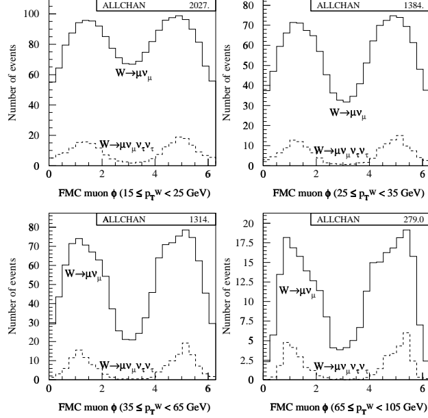
FIG. 12: Muon \phi distributions for the four p_T^W bins for muon W +jet FMC events (solid histogram) and for tau W +jet FMC background (multiplied by 5), where the tau decays to a muon (dashed histogram). The histograms are normalized to the FMC signal event yields.
