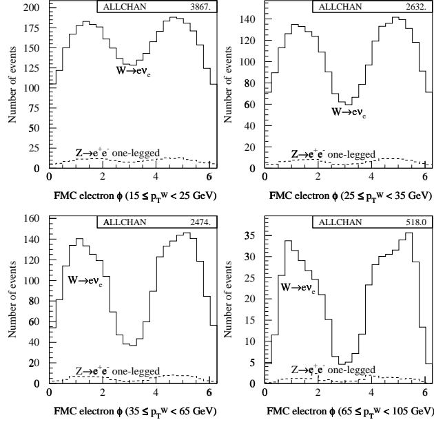
FIG. 9: Electron \phi distributions for the four p_T^W bins for electron W +jet FMC events (solid histogram) and for Z +jet FMC background (multiplied by 5), where one of the electrons from the Z decay is undetected and the other one passes the detection and analysis requirements (dashed histogram). The histograms are normalized to the electron FMC signal event yields.
