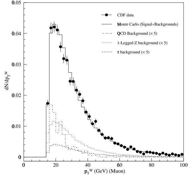
FIG. 18: The transverse momentum of the W for the muon W +jet data sample (points) along with the FMC signal simulation including backgrounds (solid histogram). The backgrounds are multiplied by 5, to be visible. The data and expected signal+background distributions are normalized to unity.
