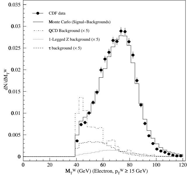
FIG. 19: The transverse mass of the W for the electron W +jet data sample (points) along with the FMC signal simulation including backgrounds (solid histogram). The backgrounds are multiplied by 5, to be visible. The data and expected signal+background distributions are normalized to unity.
