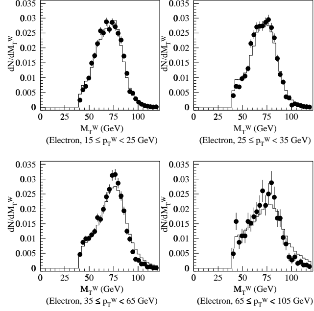
FIG. 20: The transverse mass of the W for the electron W +jet data sample (points) along with the FMC signal simulation including backgrounds (histogram), for the four p_T^W bins. The data and expected signal+background distributions are normalized to unity.
