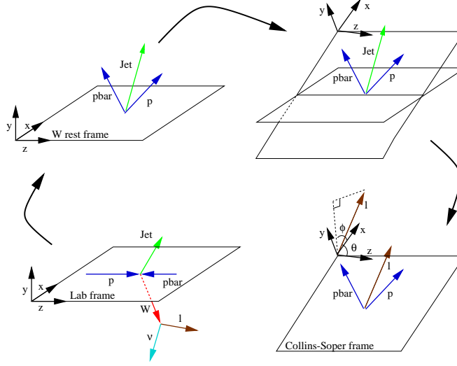
FIG. 1: Transforming from the laboratory frame to the Collins-Soper frame. We first boost to the W rest-frame, then rotate the x-z plane so that it coincides with the p-\bar{p} plane. Finally we rotate the frame around the y -axis so that the z -axis bisects the angle between \vec{p} and -\vec{p} . The positive y axis is selected to have the same direction as \vec{p}_{CS} \times \vec{p}_{CS} .
