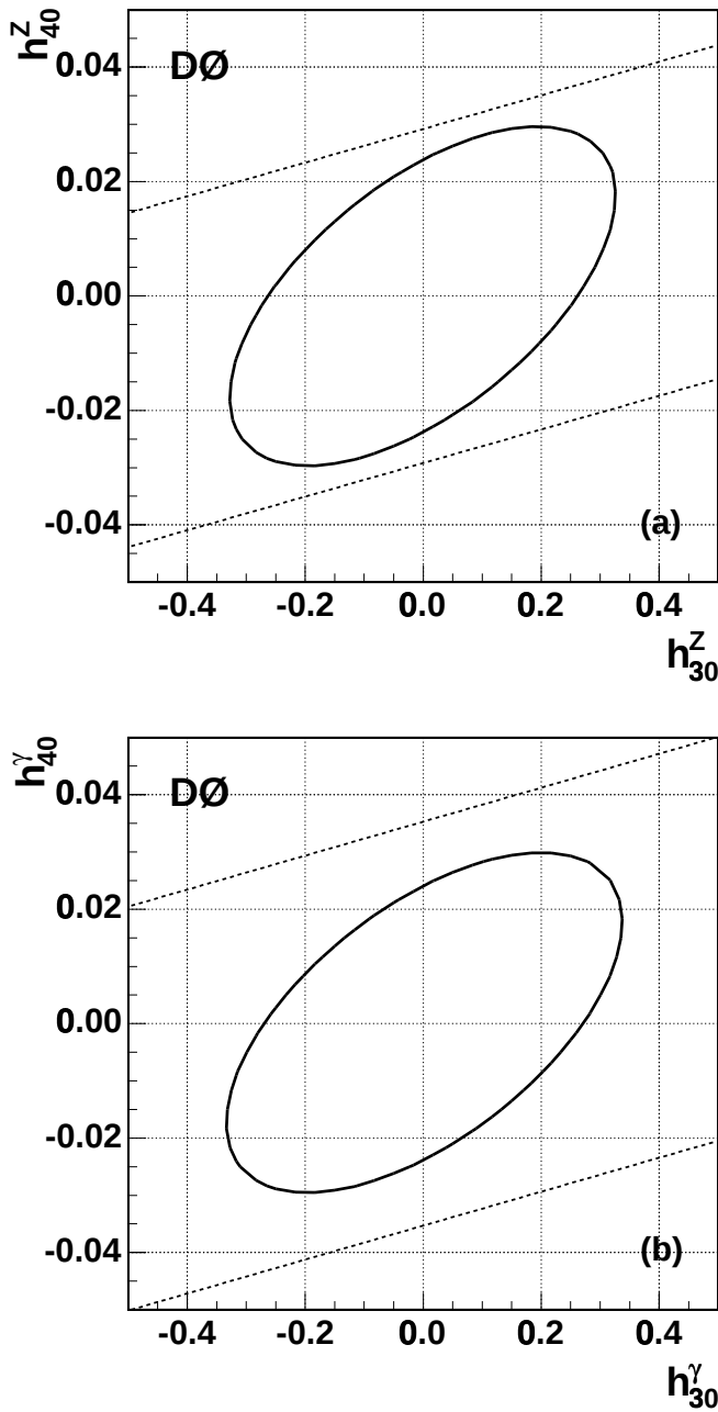
FIG. 3: The 95% C.L. two-dimensional exclusion limits for CP-conserving ZZ\gamma (a) and Z\gamma\gamma (b) couplings for \Lambda = 1 TeV. Dashed lines illustrate the unitarity constraints.
