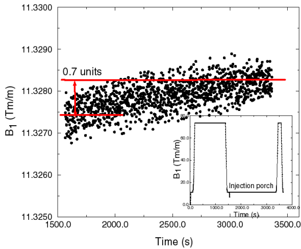
Figure 3: A main field for the Tevatron quadrupole N921F after 30 min injection porch. The insert shows the main field dependence versus time for this measurement. A decay of 0.7 units was observed
