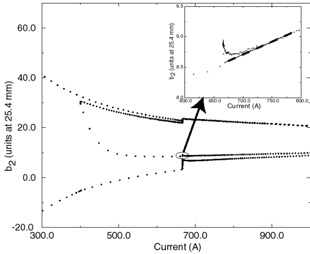
Figure 1: Typical b_2 hysteresis loop with short injection porch. The upper insert shows the snap-back after 6 s of injection porch and the line approximation of the loop in the snap-back's region
