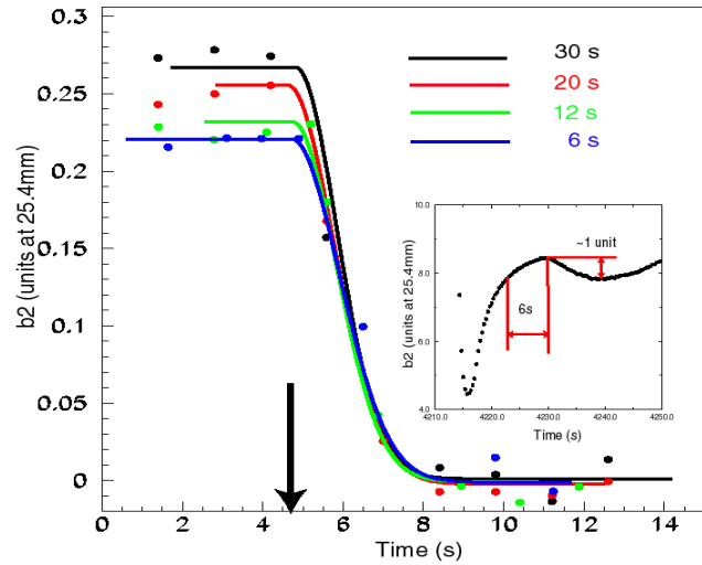
Figure 2: Snapback of the sextupole component in TC0604 for a plateau at injection of 6,12,20 and 30 s for 60 min flattop and 5 min back-porch. A fast decay of approximately 0.2 units is observed after first 6 s. The arrow shows the beginning of the snapback. The insert shows the decay and snapback for TC1130 in case of 6 s injection porch
