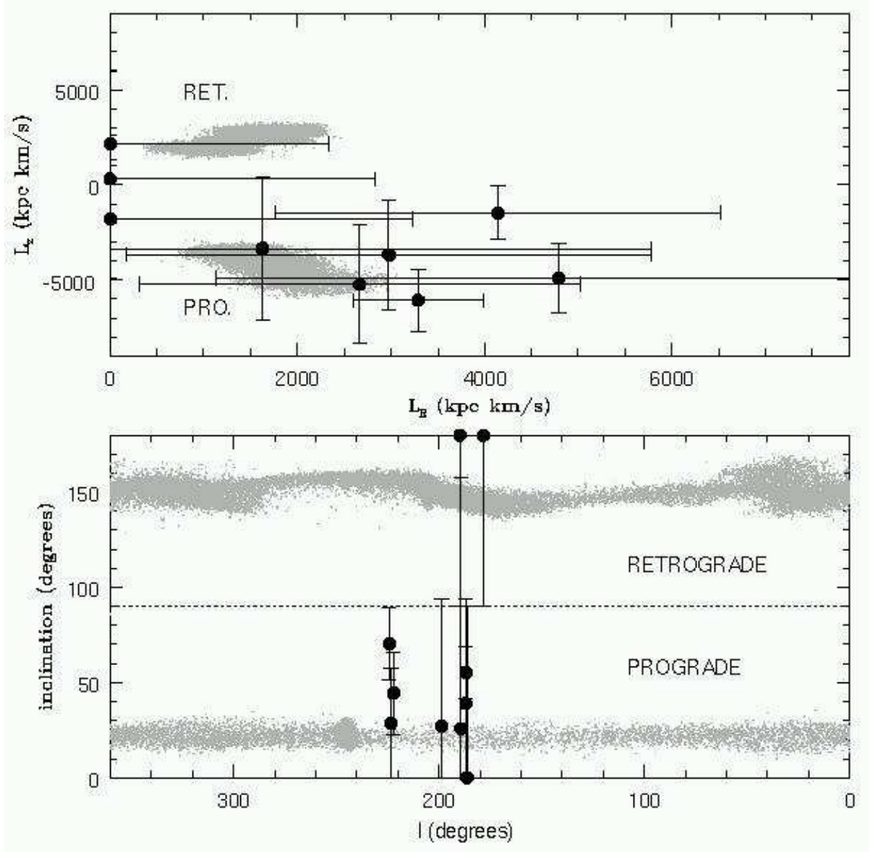
Fig. 5.— Upper panel: Prograde ( pro1 model) vs. retrograde ( ret1 model) values of the angular momentum components. Dots represent observational values after being corrected (see text). Lower panel: Orbital inclination as a function of Galactocentric longitude.
