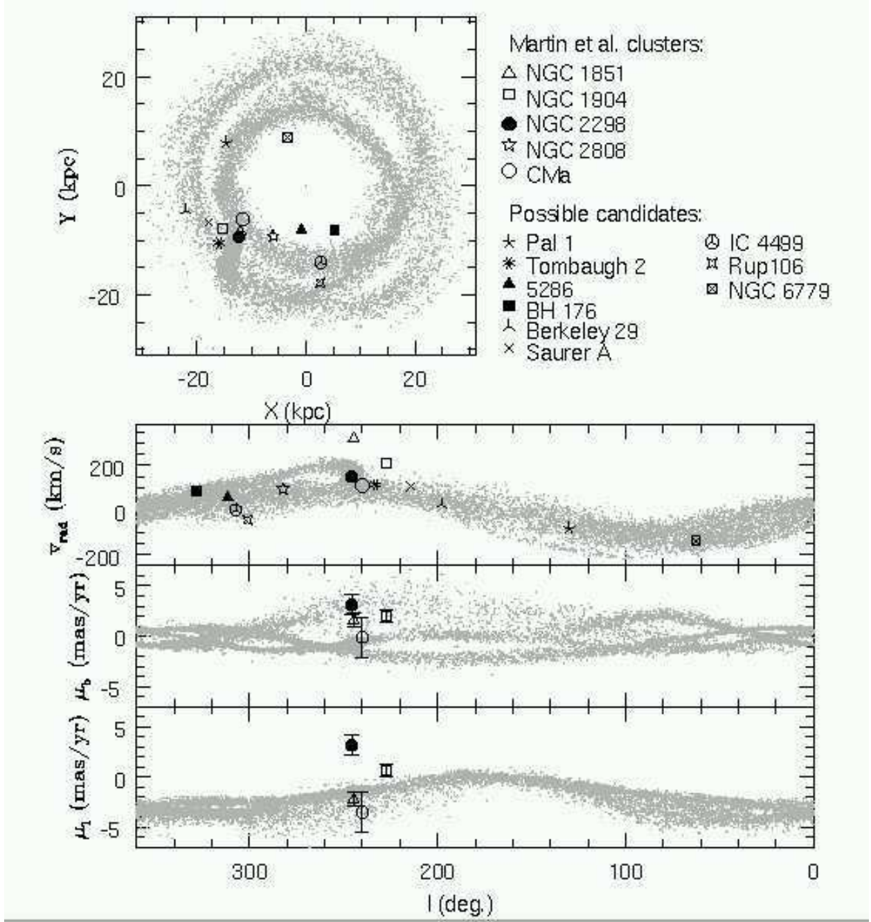
Fig. 11.— Upper panel: X-Y projection of the pro1 model debris against some globular and open clusters possibly associated with the Monoceros stream. Middle-upper panel: radial velocity curve. Lower-middle panel: Proper motions in the latitudinal component. Lower panel: Proper motions in the longitudinal component. The open circle denotes the position and radial velocity of the CMa dwarf (Martin et al. 2004b).
