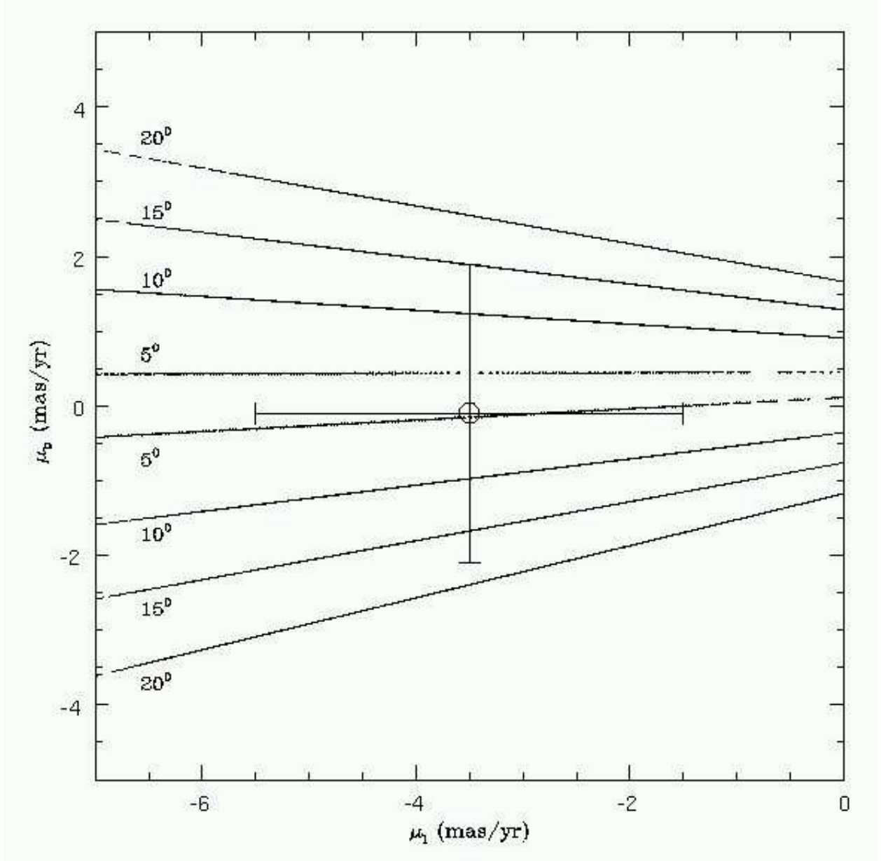
Fig. 9.— Orbital inclination of CMa as a function of \mu_l, \mu_b , fixing the radial velocity to 109 km/s and the heliocentric distance to r_s = 7.2 kpc.
