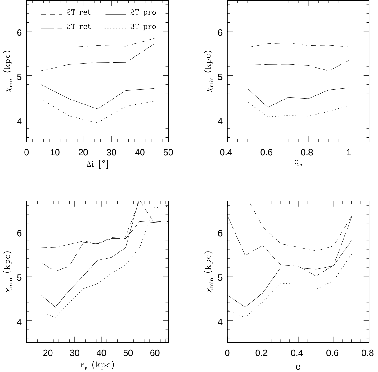
Fig. 1.— Minimum values of the fitting parameter \chi as a function of initial heliocentric distance (lower-left panel), eccentricity (lower-right panel), halo axis-ratio (upper-right panel) and orbital inclination (upper-left panel). For each parameter, we perform the fit assuming that the observed tidal stream can be reproduced by an orbit segment of extension \Delta T \simeq 2T_{\text{orb}} (solid lines) or 3T_{\text{orb}} (dotted lines).
