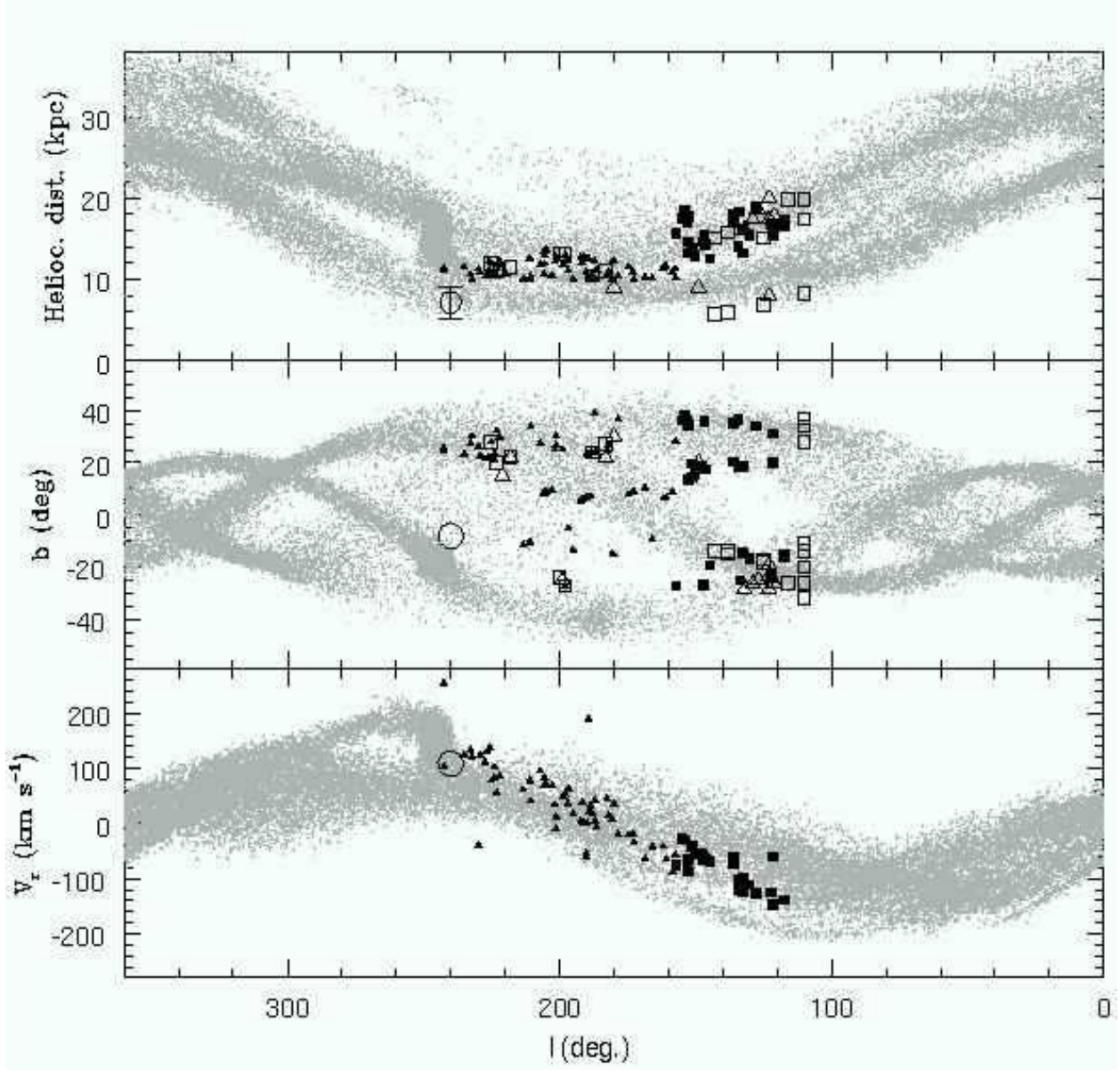
Fig. 8.— Comparison of our model for the Monoceros stream progenitor against CMA dwarf properties (open circle). Upper panel: heliocentric distances of stream particles from model pro1 (grey) against observations. Middle panel: Projection in Galactocentric coordinates. Lower panel: heliocentric radial velocities.
