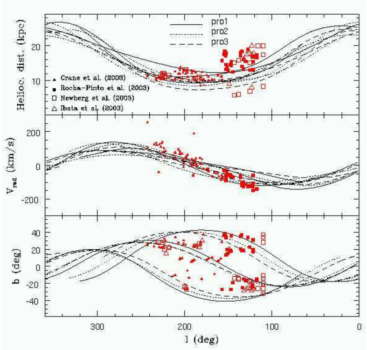
Fig. 2.— Best-fitting prograde solutions (see Table 3). Upper panel: Heliocentric distance as a function of Galactic longitude ( l ). Middle panel: Heliocentric radial velocity. Lower panel: Projected spatial position in the l-b plane. Open triangles and full squares represent detections of stars. Open squares denote colour-magnitude detections (with no radial velocity measurements available).
