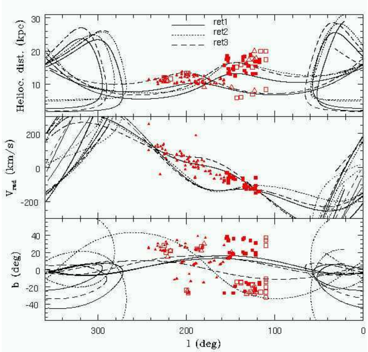
Fig. 3.— As Fig. 2 for our best-fitting retrograde solutions.
