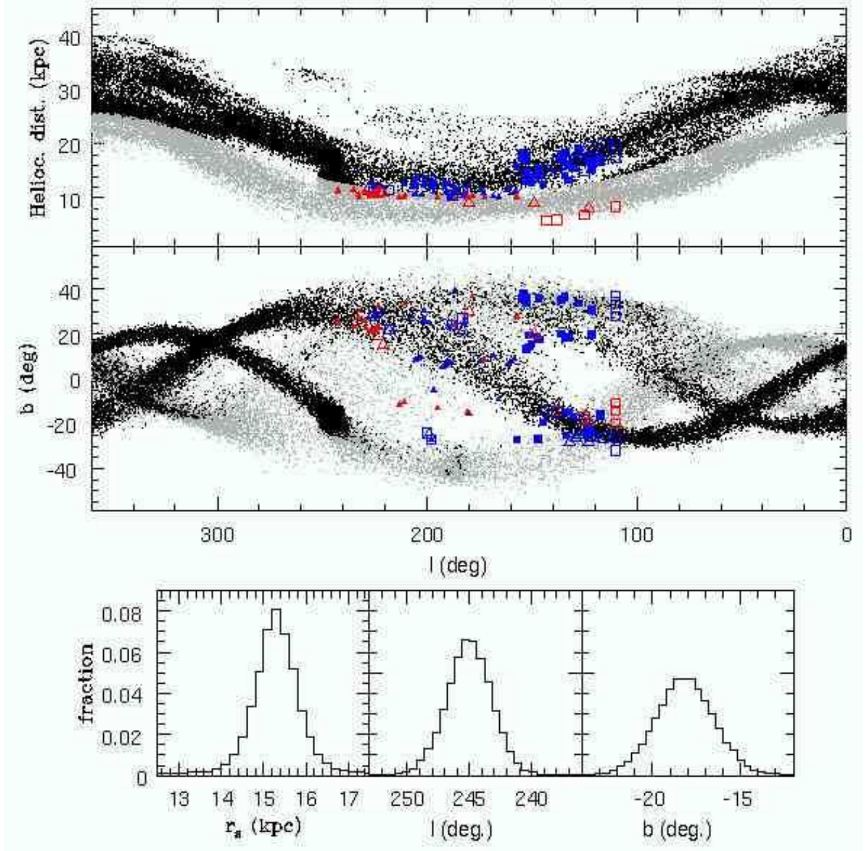
Fig. 7.— Model pro1 integrated 2.99 Gyr. Heliocentric distance (upper panel) and galactocentric latitude (middle panel) of debris as a function of galactic longitude. We use notation of Fig. 4 to distinguish different observational sources. Grey and black dots denote, respectively, particles at r \geq 18 kpc (“outer ring”) and r < 18 kpc (“inner ring”) from the Galaxy centre. Lower panels show the distribution of debris around the main system remnants. From left to right we plot the heliocentric distance, Galactocentric longitude and the Galactocentric latitude distributions, which are normalized to the total number of dwarf galaxy stars ( N_s = 10^5 ).
