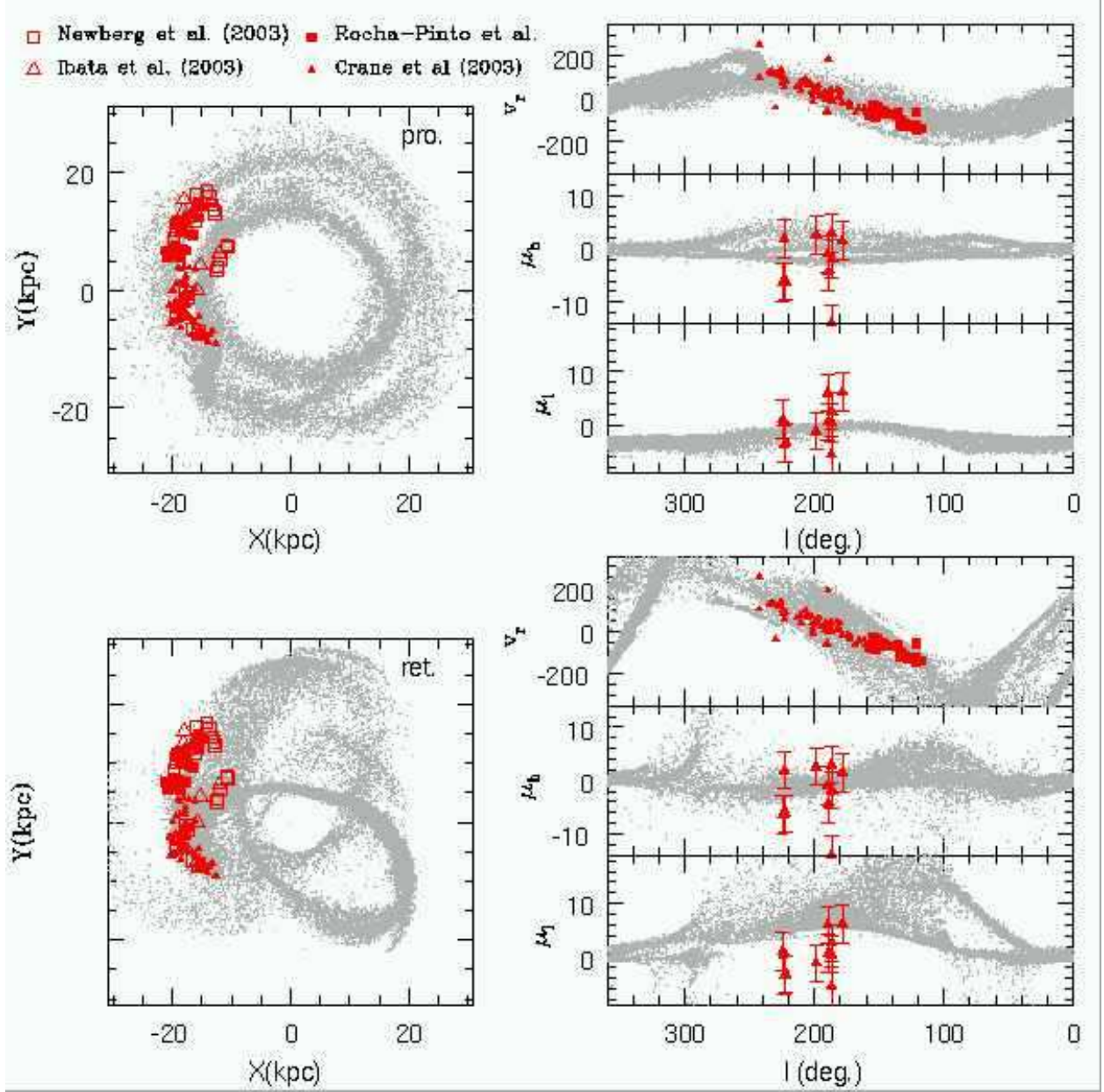
Fig. 4.— Prograde ( pro1 model) vs. retrograde ( ret1 model) orbits. Left column: X-Y Galaxy plane projections. The sun is placed at (X, Y, Z) = (-8, 0, 0) kpc. Right column: Heliocentric radial velocity curve (upper panel, given in km/s). Proper motions in the latitudinal (middle panel) and in the longitudinal (lower panel) components, both given in mas/yr.
