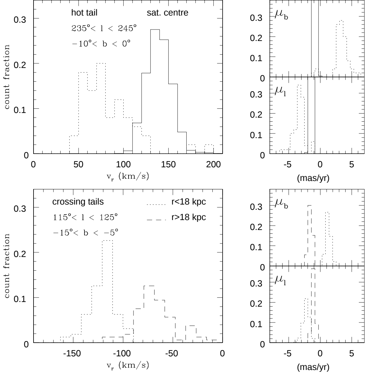
Fig. 10.— Left column: Distribution of radial velocities in the CMa region from model pro1 (upper panel) and in a region of tail overlap (lower panel). The velocity distribution of the satellite center includes particles within 243^\circ \leq l \leq 247^\circ and -17 \leq b \leq -13^\circ . The number of particles in each distribution was 8400 in the dwarf center and 50 in the surrounding tail. Dotted and dashed lines in the lower panel show the distributions from particles in the inner and outer “rings”, respectively. Right column: Distribution of proper motions in the regions indicated above.
