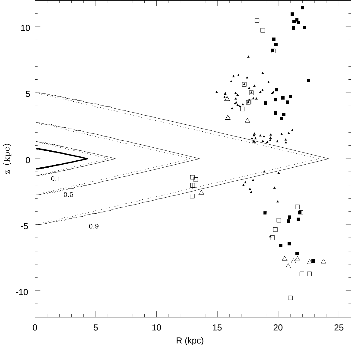
Fig. 12.— Iso-contours of the thick disk number of particles against stream detections. The Sun is located at R = z = 0 . The strong line represents the maximum like-hood directions of finding thick disk stars towards the Galactic anticenter ( l = 180^\circ ). Lines show the R, z values where the number of thick disk stars is 10%, 50% and 90% of the total number if looking at the Anti-center (full lines) and 70^\circ away (dotted lines).
