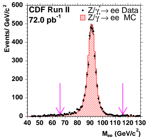
FIG. 1: Distributions of M_T for W \rightarrow \mu\nu (top) and M_{e^+e^-} for Z/\gamma^* \rightarrow e^+e^- (bottom). The arrows in the M_{e^+e^-} distribution define the mass window.
