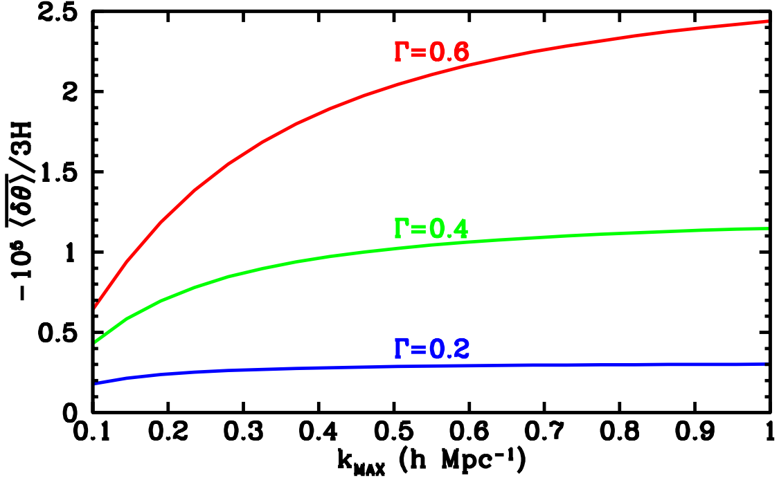
FIG. 1: The present mean value, \langle \delta\theta \rangle / 3H , in the matter-dominated Universe as a function of the ultraviolet cutoff k_{\text{MAX}} for various values of the shape factor \Gamma .
