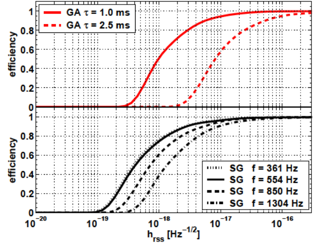
FIG. 13: Burst detection efficiency for triple coincidence as a function of h_{rss} , using the TFCLUSTERS event trigger generator, averaging over wave directions and polarizations, for six different waveforms: GA refers to the Gaussians defined in Eqn. 5.1 and SG to the sine-Gaussians defined in Eqn. 5.2.
