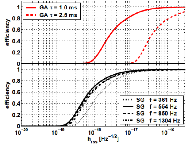
FIG. 14: Same as Fig. 13, for the SLOPE event trigger generator.
