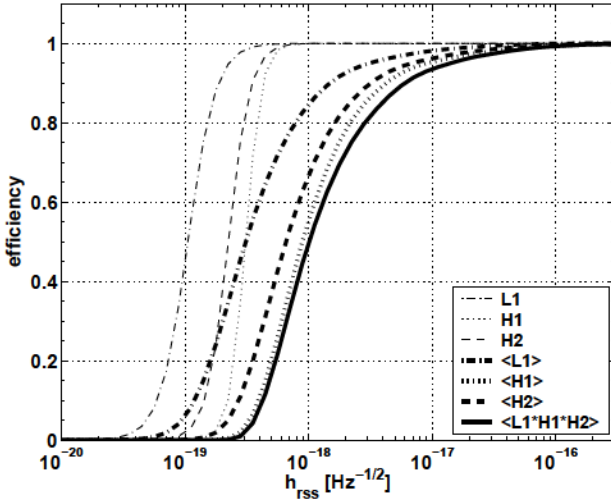
FIG. 12: Burst detection efficiency for Gaussian bursts with \tau = 1 ms, as a function of h_{rss} , for each of the three LIGO detectors, and for the triple coincidence, using the TFCLUSTERS event trigger generator. The lighter grey curves are the same as the curves in Fig. 10. The darker curves to the right of them are the result of averaging the efficiency curves over wave directions and polarizations (denoted by \langle \dots \rangle in the legend) as described in section V C.
