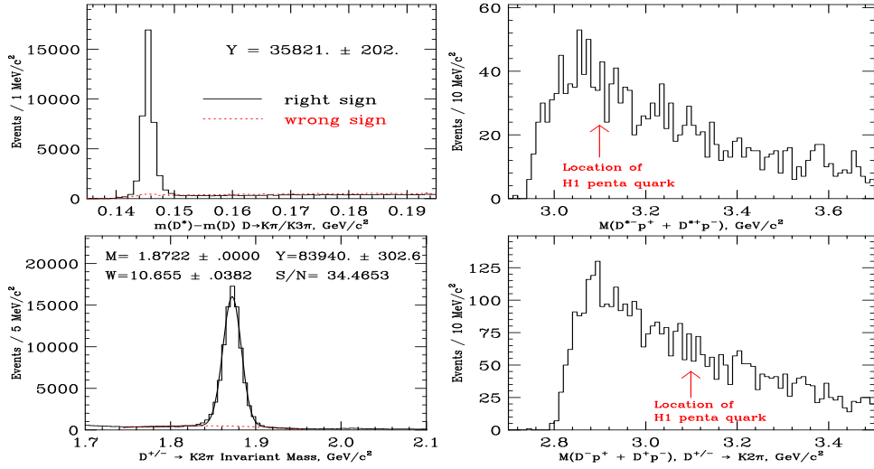
Fig. 3. We add a proton to the D^{*-} events and D^- events (left) to search for \Theta_c(3099) (right).
