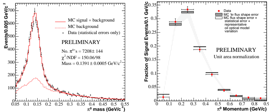
Fig. 1. \pi^0 reconstructed mass peak (left), and momentum spectrum (right). The mass peak signal is from NC resonant and coherent single \pi^0 events. Backgrounds to these events contain interactions which produce \pi^0 ; the peak near the \pi^0 mass in the background is expected. Errors shown are shape errors: dark bands are from flux errors, and the light bands are from the current understanding of the optical model.
