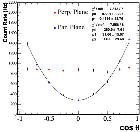
(a) Scattering Angular Distribution
