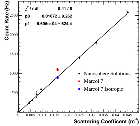
(b) Scattering Rate
