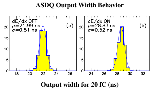
Figure 27. The distribution of output widths for ~6600 ASDQ channels for an injected charge of 20 fC and a) dE/dx off and b) dE/dx on. The vertical scale is channels / 1000. The variation as a function of channel number within the chip is much less than \sigma .
