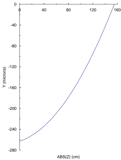
Fig 36. Graph of vertical displacement as a function of absolute vertical displacement.
