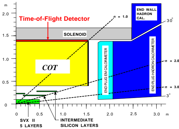
Figure 1. Side view of the central region of the CDF detector (quarter section), showing the location of the COT.
