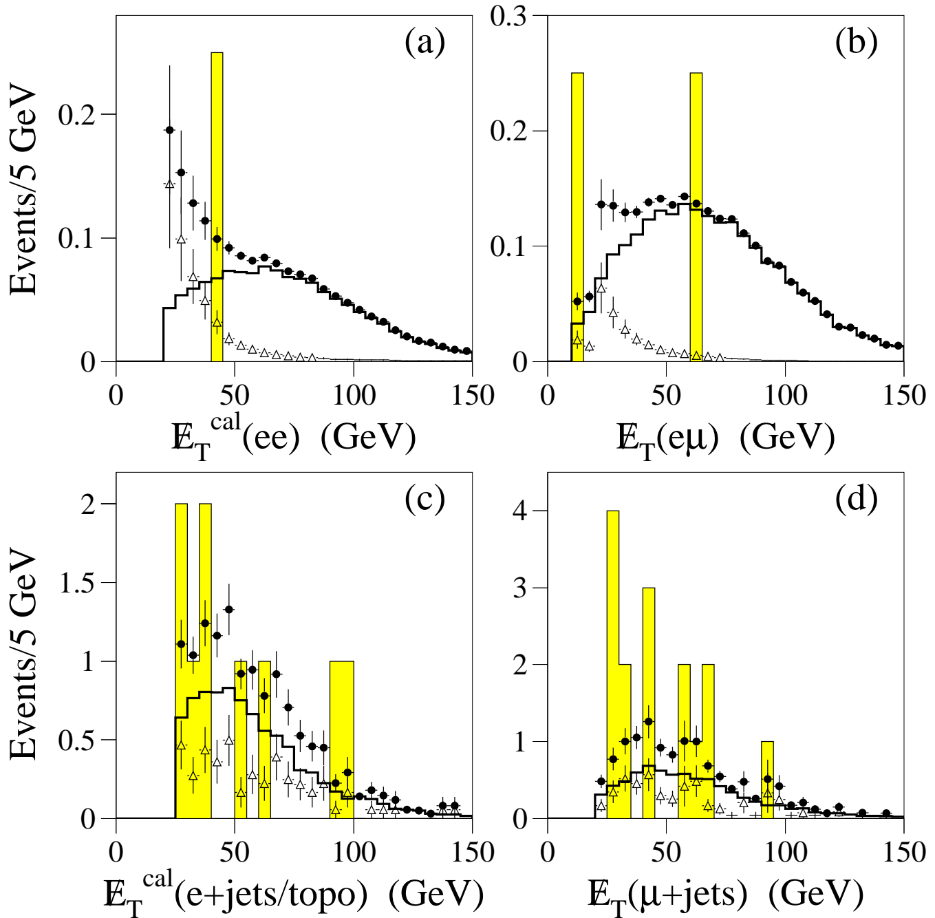
FIG. 34. \cancel{E}_T distributions for the ee (a) and e+\text{jets}/\text{topo} (c) channels, and \cancel{E}_T distributions for the e\mu (b) and \mu+\text{jets}/\text{topo} and \mu+\text{jets}/\mu (d) channels: t\bar{t} candidates (shaded histogram), t\bar{t} MC [HERWIG, m_t = 170 \text{ GeV}/c^2 ] (unshaded histogram), expected background (open triangles), and expected signal plus background (solid circles). The ee and e\mu candidate histograms [(a)–(b) shaded] have been multiplied by a factor of 0.25 for presentational clarity. The measured \cancel{E}_T for e\mu candidate 58796-7338(417) is 182.9 GeV and is therefore off scale in plot (b).
