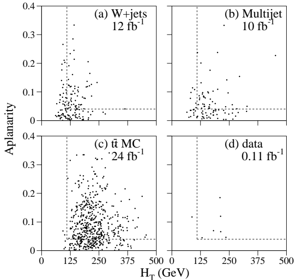
FIG. 28. Scatter plots of \mathcal{A} vs H_T for the \mu +jets/ \mu channel for (a) VECBOS W +jets MC background, (b) QCD multijet background, (c) HERWIG t\bar{t} MC ( m_t = 170 GeV/ c^2 ), and (d) data. The effective luminosity given for plot (b) is determined as the product of the luminosity of the selected multi-jet sample and the inverse of the muon misidentification rate.
