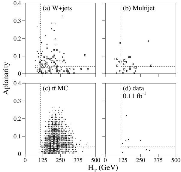
FIG. 27. Scatter plots of \mathcal{A} vs H_T for the e +jets/ \mu channel for (a) VECBOS W +jets MC background, (b) QCD multijet background, (c) HERWIG t\bar{t} MC events ( m_t = 170 GeV/ c^2 ), and (d) data.
