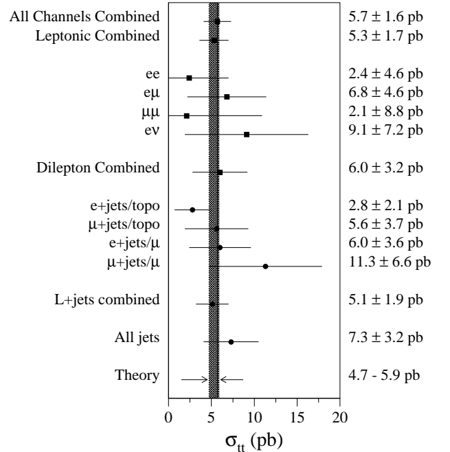
FIG. 29. D\theta measured t\bar{t} production cross section values for all channels, assuming a top quark mass of 172.1 GeV/ c^2 . The vertical line corresponds to the cross section for all channels combined and the shaded band shows the range of theoretical predictions [45–47,50].
