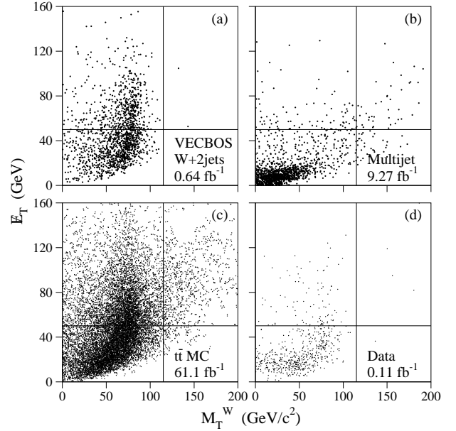
FIG. 13. Scatter plots of \cancel{E}_T vs M_T^W for the e\nu channel: (a) W +jets background, (b) background from multijet events with a misidentified electron, (c) t\bar{t} signal ( m_t = 170 \text{ GeV}/c^2 ), and (d) data. The signal region is shown in the upper right corner of each plot ( M_T^W \geq 115 \text{ GeV}/c^2 , \cancel{E}_T \geq 50 \text{ GeV} ).
