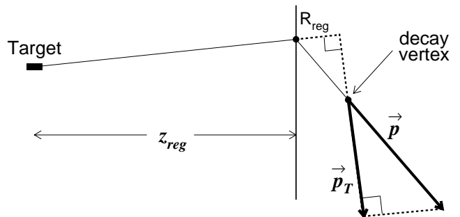
FIG. 11: Illustration of the transverse momentum, \vec{p}_T , for a kaon that scatters in the regenerator and then decays at the point labeled “decay vertex.” The line connecting the target to \mathbf{R}_{\text{reg}} represents the kaon trajectory upstream of the regenerator, \vec{p} is the measured momentum of the \pi^+ \pi^- system, and z_{\text{reg}} is the distance from the target to the downstream end of the regenerator.
