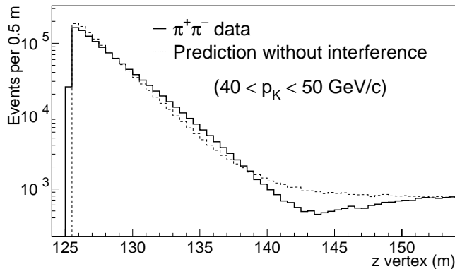
FIG. 24: z decay distribution of K \rightarrow \pi^+ \pi^- decays in the regenerator beam, for the restricted momentum range 40–50 GeV/c. The MC prediction (dashed) is without the interference term that is proportional to “ 2|\rho||\eta| ” in Eq. 14.
