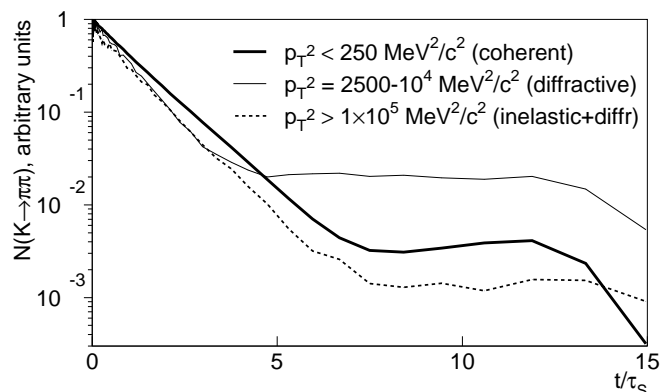
FIG. 17: Acceptance-corrected distribution of the number of regenerator beam K \rightarrow \pi^+\pi^- decays vs. the number of K_S lifetimes ( t/\tau_S ), for kaon momenta between 40 and 50 GeV/c. The proper time t = 0 corresponds to the downstream edge of the regenerator. The p_T^2 ranges are indicated on the plot for each curve. The thick curve is for coherent K \rightarrow \pi^+\pi^- decays. The thin solid curve corresponds to small p_T^2 and is mostly from diffractive scattering. The dashed curve is for large p_T^2 events, which are due to both inelastic and diffractive scattering. The fluctuations are due to statistics. All K \rightarrow \pi^+\pi^- cuts except p_T^2 have been applied. Backgrounds from collimator scattering and semileptonic decays have been subtracted.
