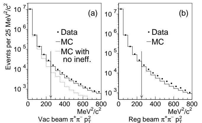
FIG. 12: \pi^+ \pi^- p_T^2 distributions after all other K \rightarrow \pi^+ \pi^- analysis cuts in (a) the vacuum beam and (b) the regenerator beam. The background-subtracted data are shown as dots, and the histogram shows the MC prediction. The selection cut is shown by the arrows. The dotted histogram in the vacuum beam shows the MC prediction without the effects of wire inefficiency, delayed hits, and accidentals (Sec. II E 2).
