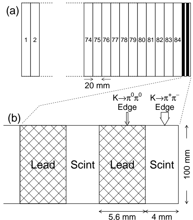
FIG. 7: (a) Diagram of the regenerator and (b) magnified view of the downstream end of the regenerator. PMTs are not shown. The dimension of each element is given in the figure. The kaon beam enters from the left. Vertical arrows above the lead and scintillator show the effective edge locations for K \rightarrow \pi^0 \pi^0 and K \rightarrow \pi^+ \pi^- decays; the width of each arrow indicates the uncertainty.
