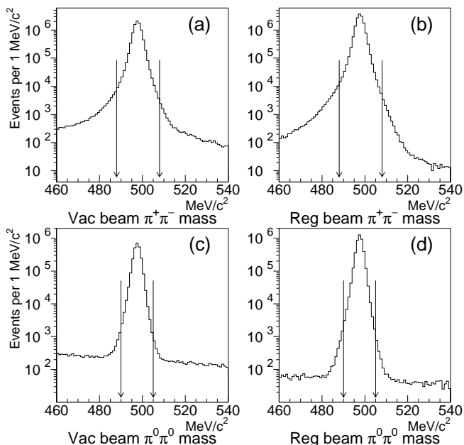
FIG. 10: Invariant mass distributions for (a) vacuum-beam \pi^+ \pi^- , (b) regenerator-beam \pi^+ \pi^- , (c) vacuum-beam \pi^0 \pi^0 , (d) regenerator-beam \pi^0 \pi^0 . All other analysis cuts are applied. The vertical arrows indicate the accepted mass range.
