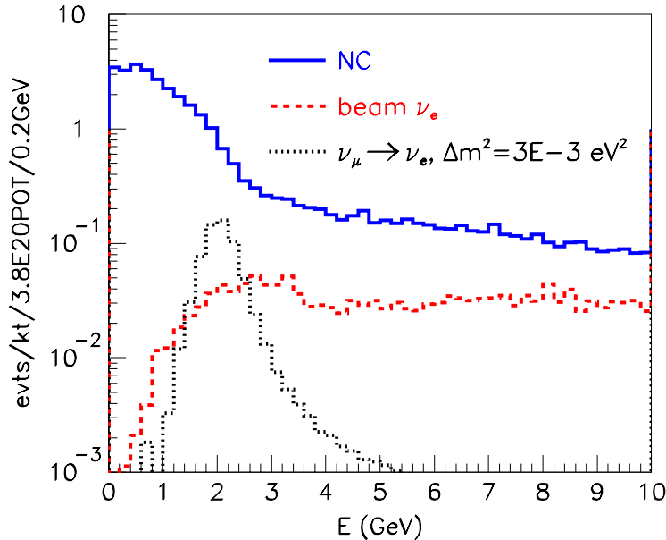
Figure 3: Visible energy distribution for a 15mrad off-axis beam: for a signal at \delta m_{32}^2 = 3 \times 10^{-3} \text{eV}^2 , the intrinsic \nu_e , and the neutral current background, assuming no particle identification, and perfect energy resolution.
