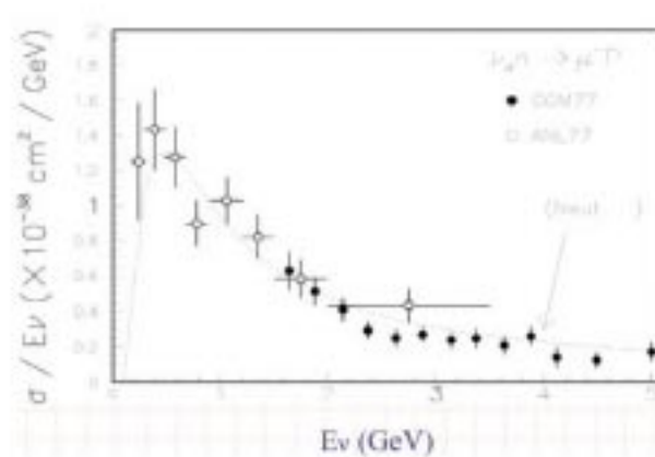
Figure 42: Neutrino quasi-elastic cross section data on neutrons.
