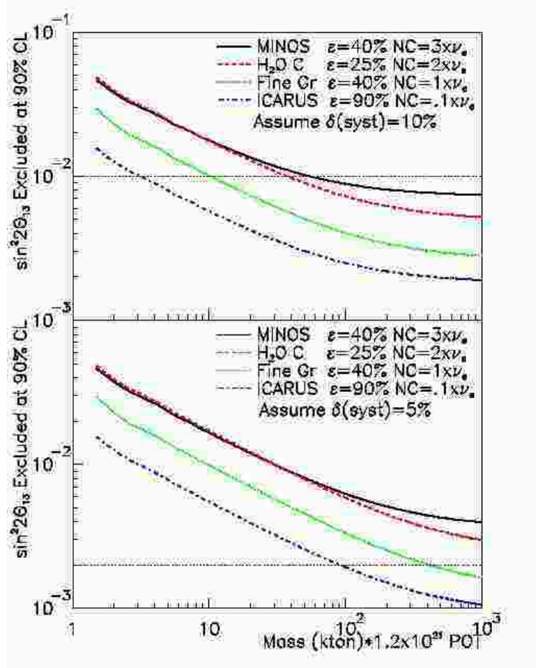
Figure 7: 90% confidence level limit one could achieve in the absence of a signal as a function of detector mass, for different detector assumptions. The top plot assumes a background uncertainty of 10% and the bottom plot assumes a background uncertainty of 5%, where the bottom plot is relevant in the event of a proton driver upgrade, where the proton intensity would be increased by a factor of 5 above nominal.
