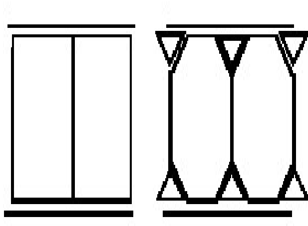
Figure 38: Examples of thin walled extrusions, shaped to form drift tubes.
