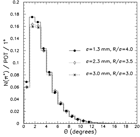
Figure 50: Angular distributions for pions coming off a graphite target. \theta is an angle between the target axis and pion direction.
