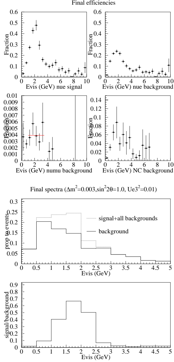
Figure 22: Left: The final fractions of events accepted as signal events after cuts the log likelihood differences. Right: The final spectra of signal and background assuming \nu_\mu \leftrightarrow \nu_e with \Delta m^2 = 0.003 \text{ eV}^2 , \sin^2 2\theta = 1.0 and U_{e3}^2 = 0.01 .
