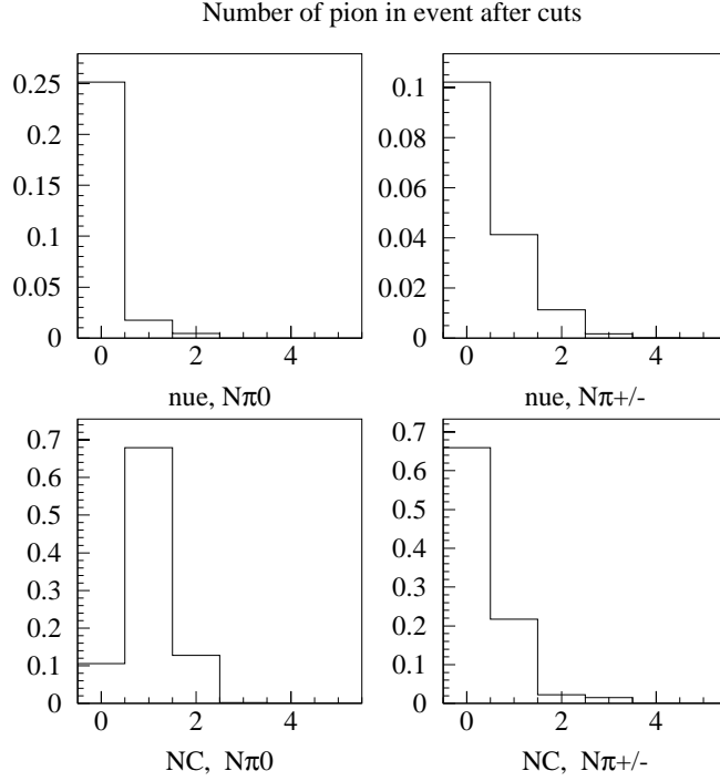
Figure 17: The number of neutral (left panels) and charged (right panels) pions in single ring \epsilon -like signal events (top panels) and neutral current-background events (bottom panels). The neutral-current backgrounds are dominated by events with a single energetic \pi^0 .
