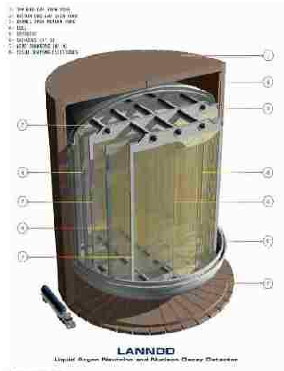
Figure 11: Concept of a 70-kton Liquid Argon Neutrino and Nucleon Decay Detector (LANDD) [37, 38].
