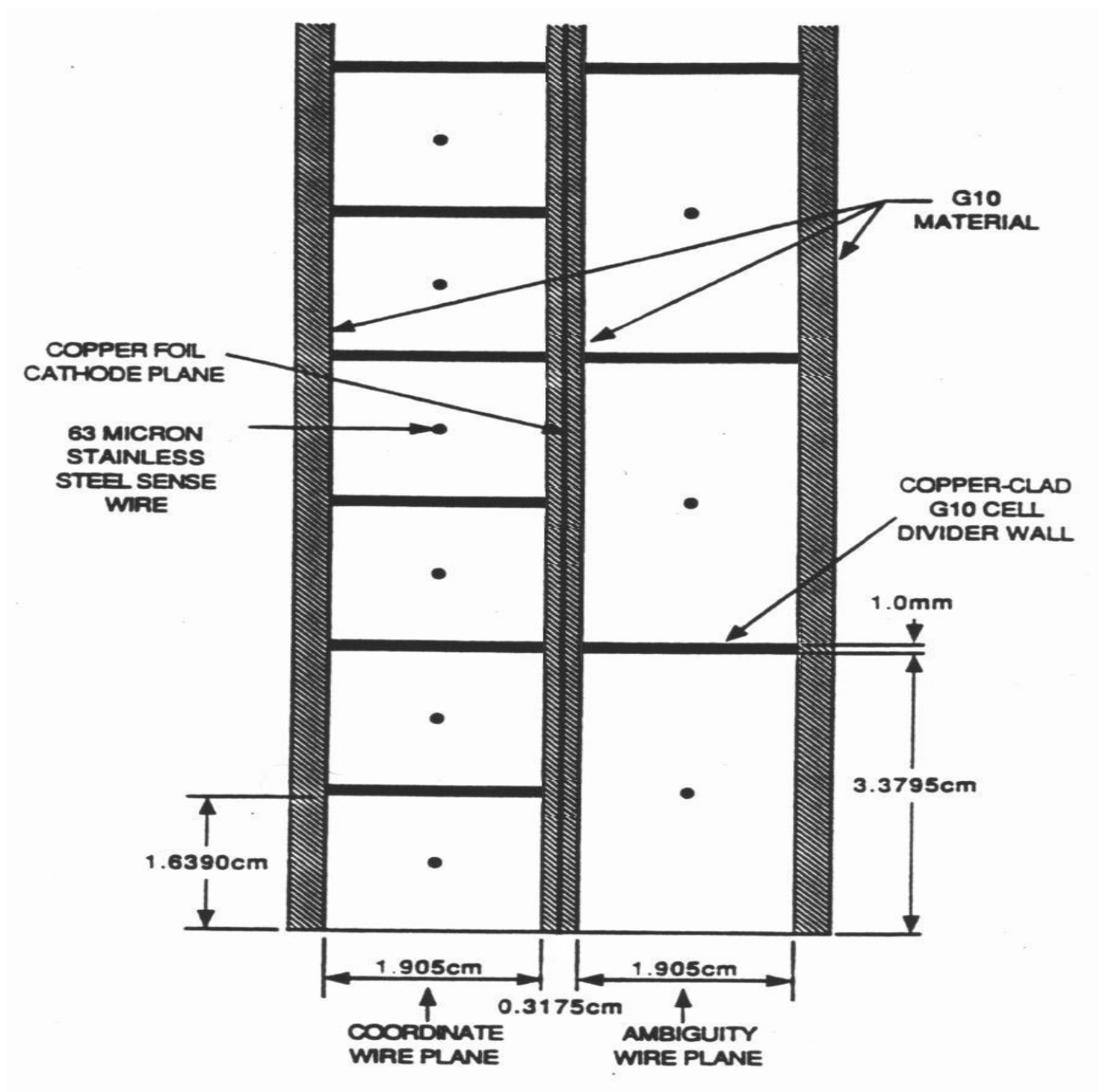
Figure 3: Schematic side view of the front plane chamber cell geometry at the inner radius. The cell sizes increased with increasing radius to define an approximately constant p_T^\mu threshold
