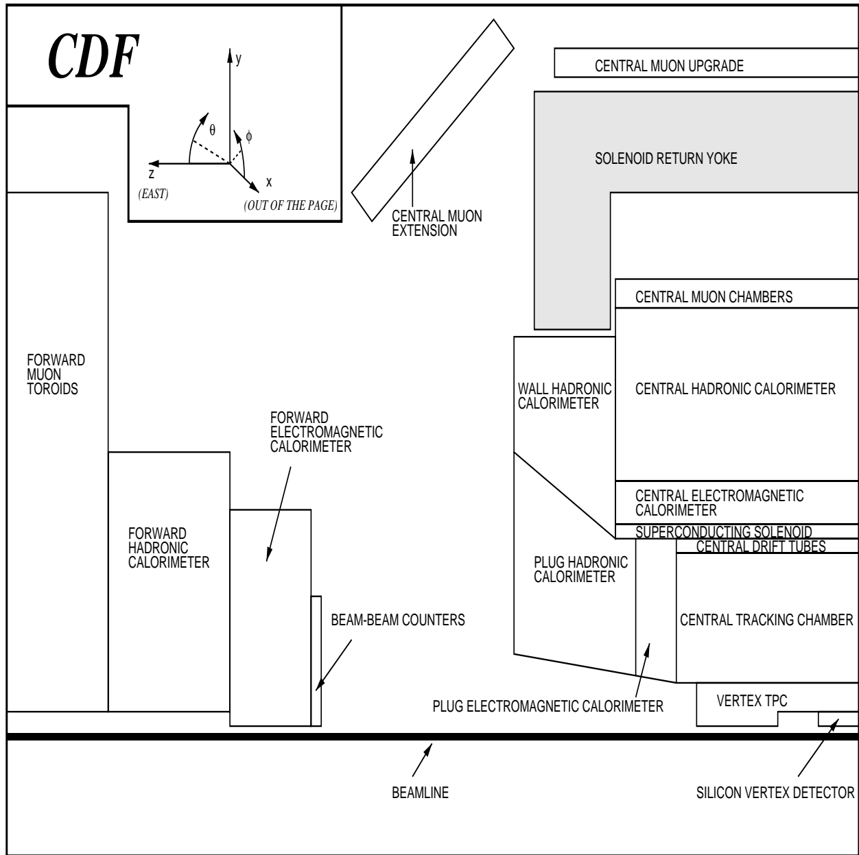
Figure 1: Side view of one quarter of the CDF detector. The interaction region is at the far right on the beamline. The forward muon toroids, chambers, and counters are shown schematically on the far left.
