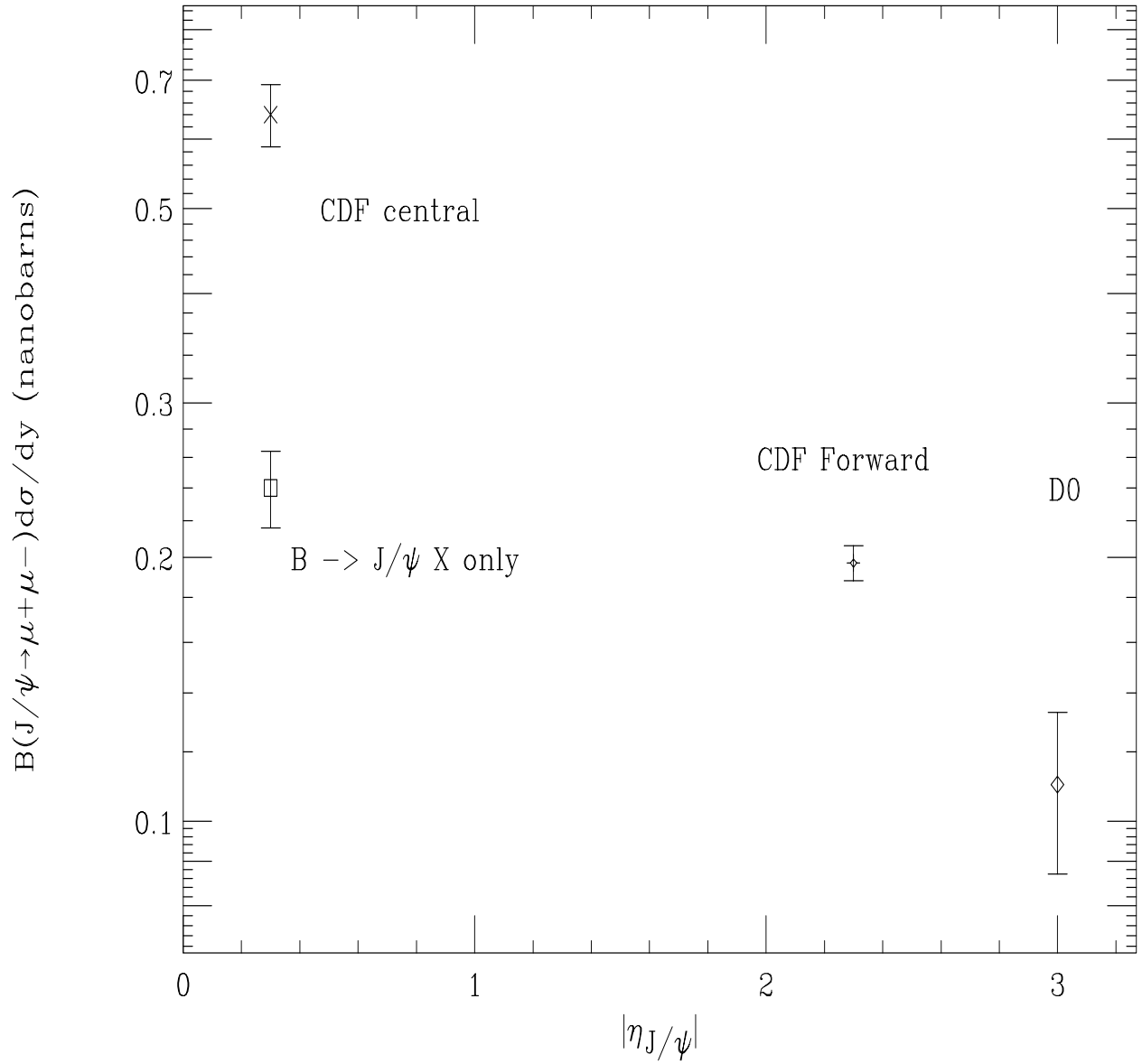
Figure 11: Integrated CDF and D0 cross sections vs |\eta| for p_T^{J/\psi} > 10 \text{ GeV}/c . The uncertainties shown are statistical only.
