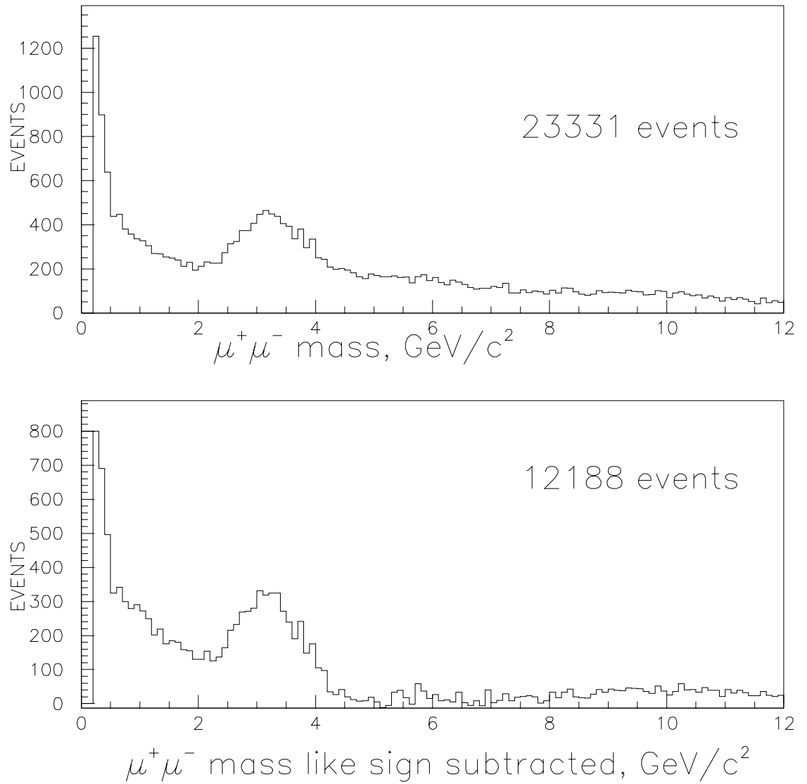
Figure 4: Opposite sign pair mass distributions from the reconstructed data file, before (top), and after (bottom) like sign subtraction.
