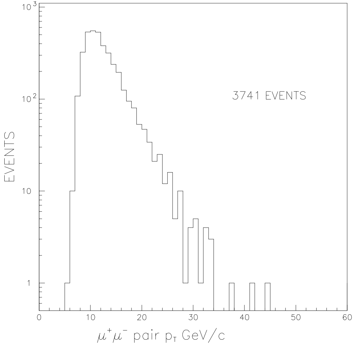
Figure 5: Opposite sign p_T^{\mu^+\mu^-} distribution
