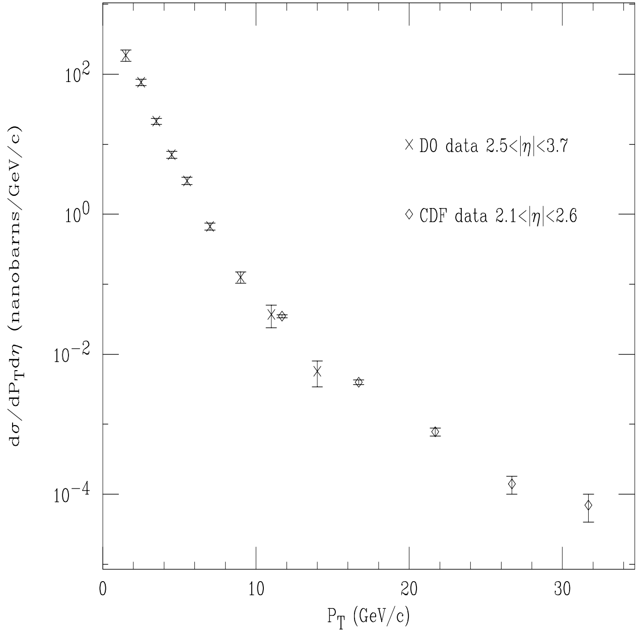
Figure 10: CDF and D0 forward cross sections vs p_T^{J/\psi} . The average pseudorapidity for CDF \langle |\eta| \rangle = 2.3 , while for D0 \langle |\eta| \rangle = 3 . The uncertainties shown are statistical only.
