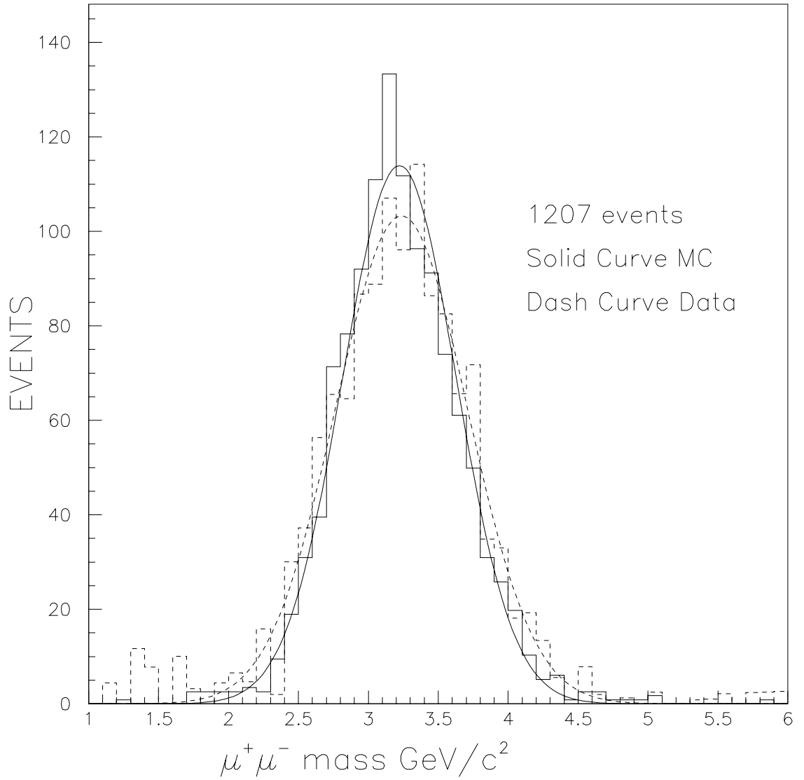
Figure 9: Background subtracted data compared to the J/\psi Monte Carlo. The MC peak is at 3.22 \pm 0.01 \text{GeV}/c^2 , with \sigma = 0.41 \pm .01 \text{GeV}/c^2 . The Gaussian fit to the data is the same as Figure 8: peak at 3.23 \pm 0.02 \text{GeV}/c^2 and \sigma = 0.47 \pm 0.02 \text{GeV}/c^2
