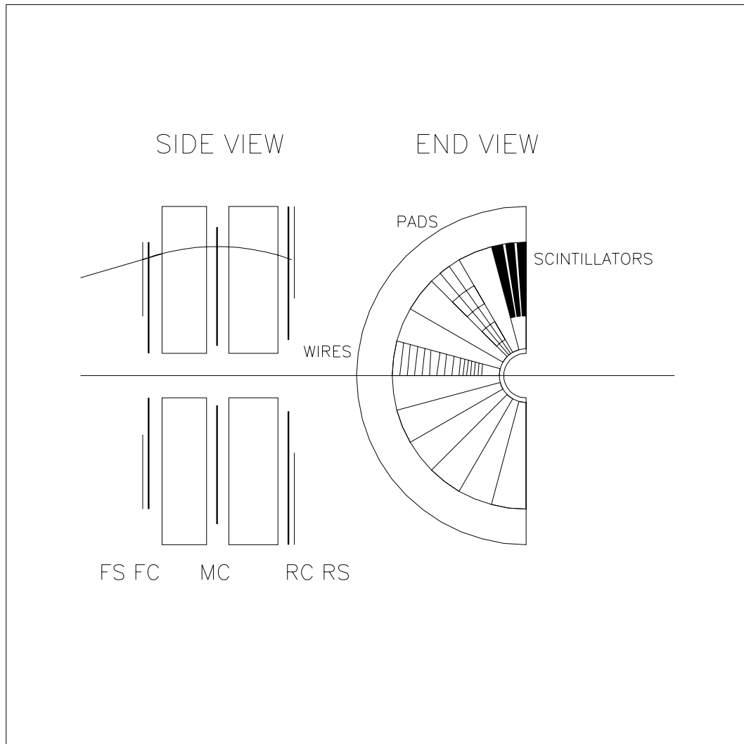
Figure 2: Side view of one pair of toroids, showing a muon trajectory, and an end view of half of the front plane. The labels FS, FC, MC, RC, and RS in the side view refer to front scintillators, front chambers, middle chambers, rear chambers, and rear scintillators respectively. The open boxes are the magnetized iron toroids. Going clockwise from horizontal in the end view, the first chamber shows the drift wires, next is the pattern of 15 cathode pads, and the top chamber shows the 5^\circ segmented scintillators. Each 15^\circ chamber was fully instrumented.
