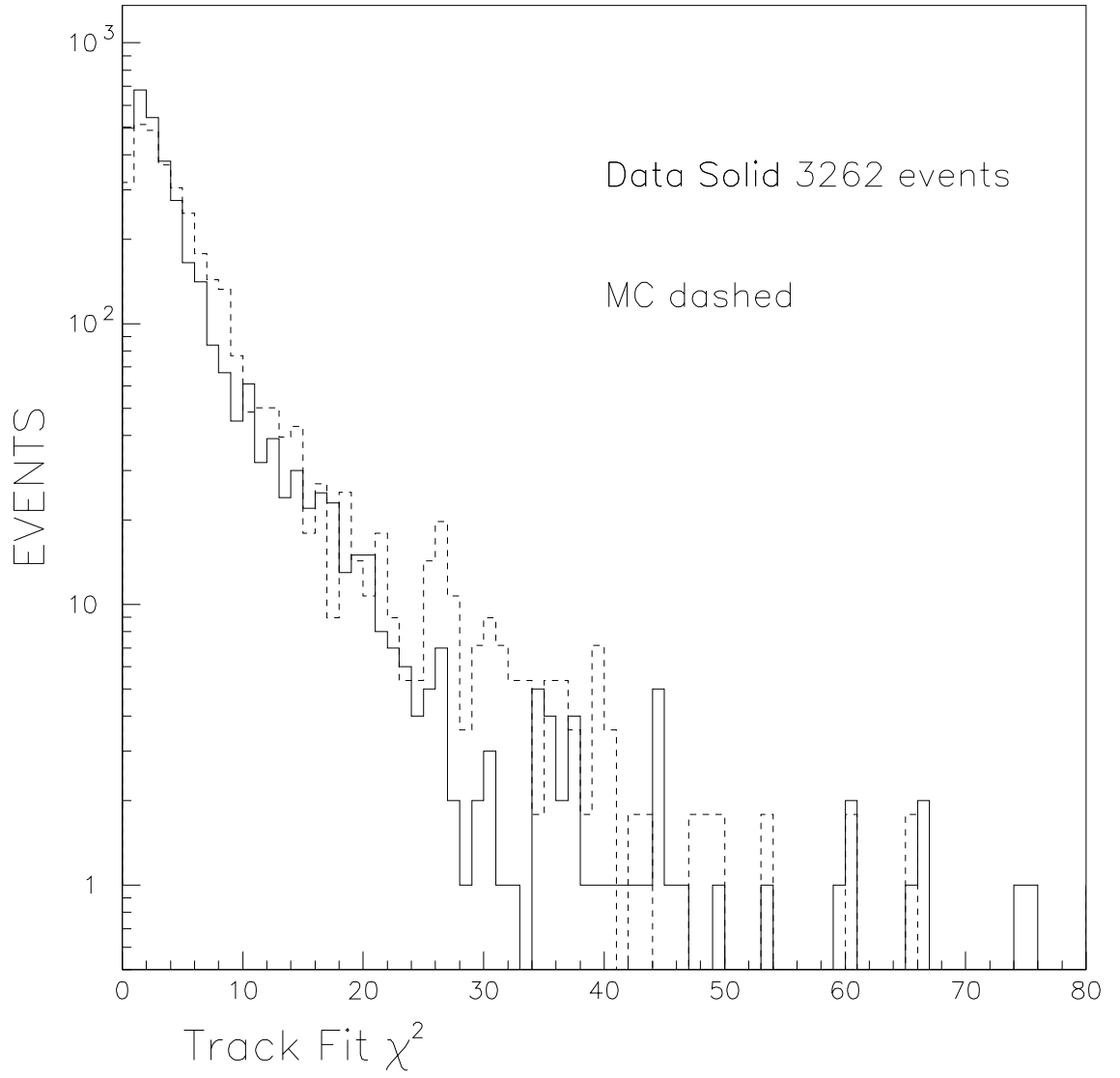
Figure 6: \chi^2 distribution for the single muon track fit compared to Monte Carlo.
