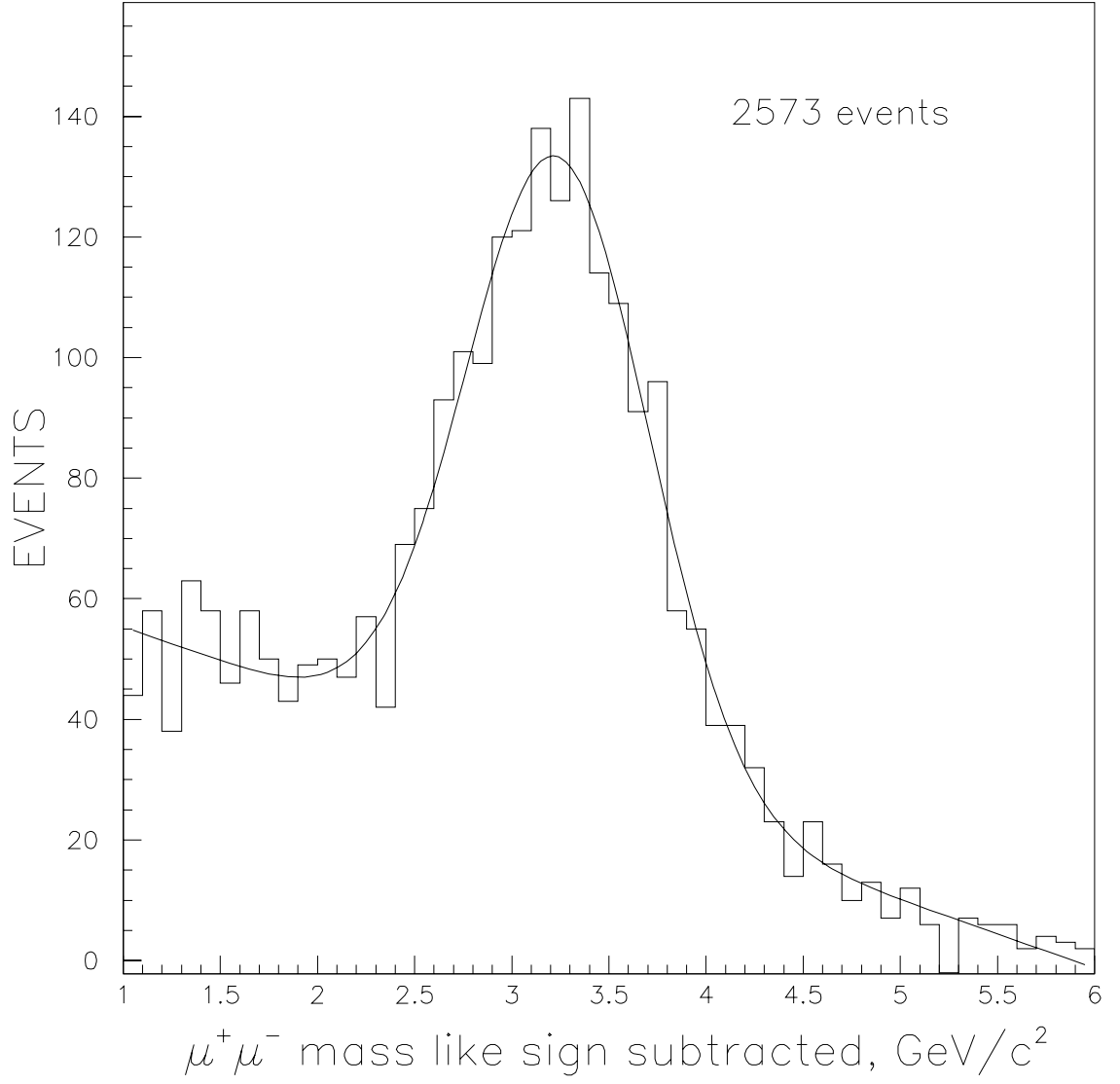
Figure 8: Final data sample after like sign subtraction. The Gaussian peak is at 3.23 \pm 0.02 \text{GeV}/c^2 , with \sigma = 0.47 \pm 0.02 \text{GeV}/c^2 . The overall fit \chi^2 = 50 for 45 degrees of freedom.
