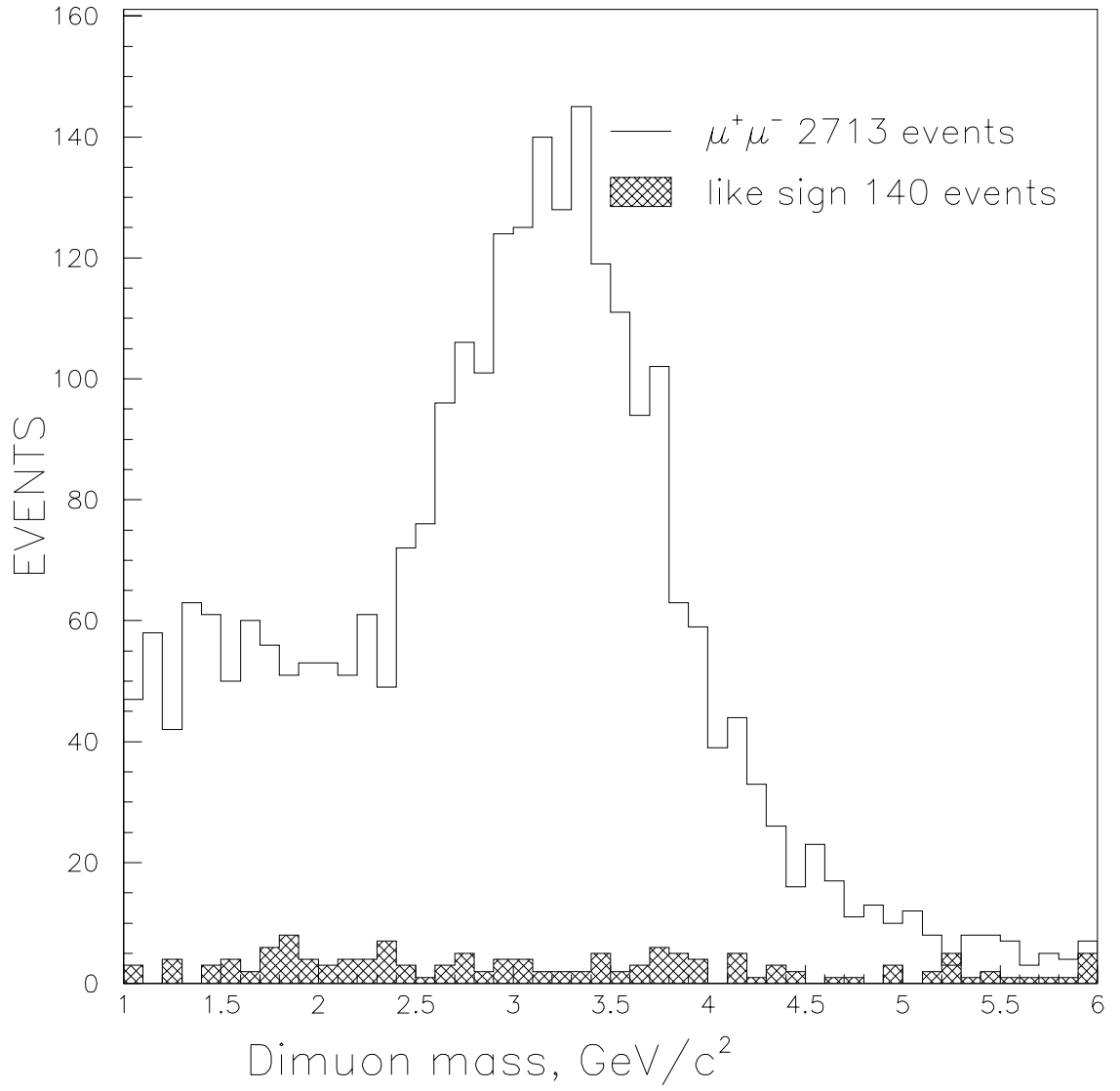
Figure 7: Data mass plot after all cuts. The like sign data are plotted separately.
