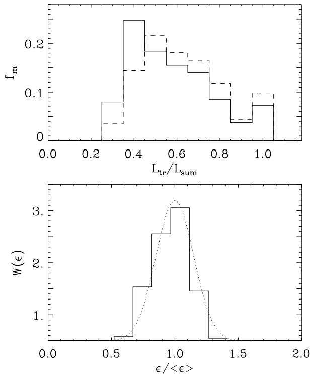
Figure 7. Top, the mass distribution versus L_{tr}/L_{sum} are plotted for N_{thr} = 5 and b_{thr} = 1.25 (solid line) and b_{thr} = 1 (dashed line). Bottom, the distribution function W(\epsilon) versus \epsilon/\langle\epsilon\rangle for b_{thr} = 1.25 and N_{thr} = 10 . The Gaussian functions with parameters listed in Table 3 are plotted by dotted lines.
