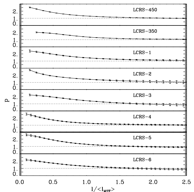
Figure 3. Functions p_{\text{MST}} (2.2) for the PDF MSTs plotted in the previous figures.
