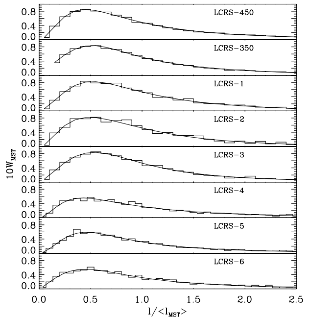
Figure 2. The PDF MSTs averaged over six slices for two full samples (LCRS-450 and LCRS-350) and for the six separate slices of LCRS-350. The best fits (2.4) are plotted by the solid line.
