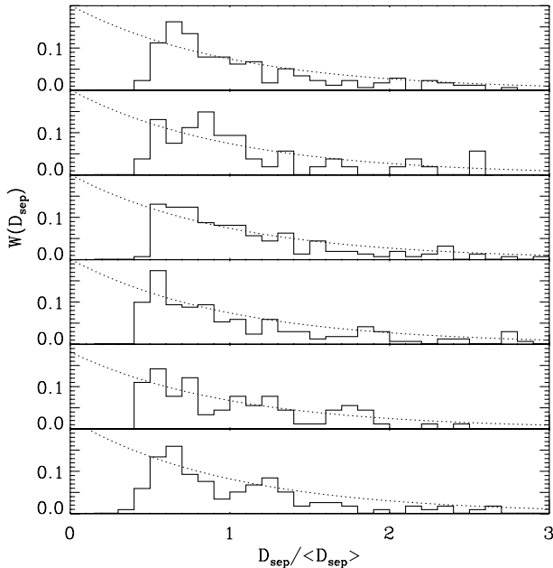
Figure 10. The distribution of the separation of richer clusters along the radial (three top panels) and transverse (three bottom panels) directions. Exponential fits are plotted by the dotted lines.
