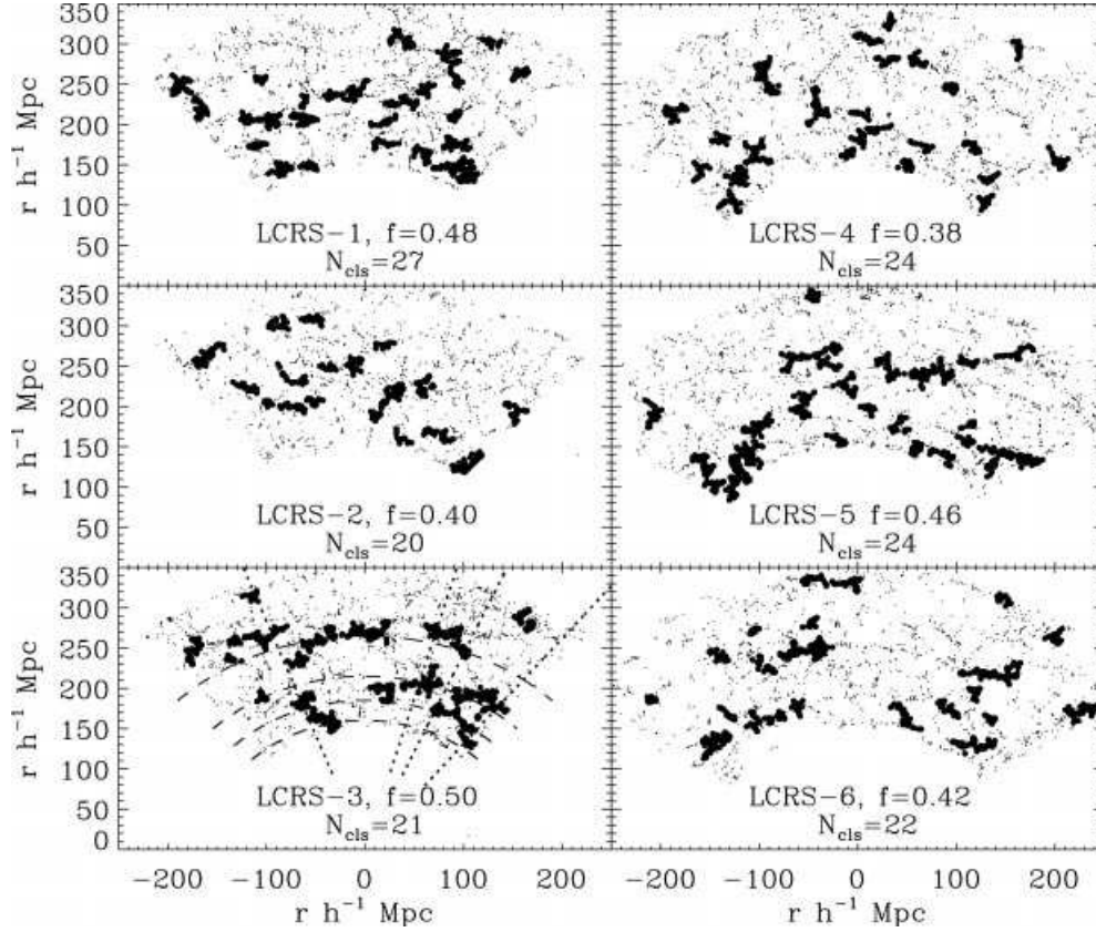
Figure 8. Spatial distribution of the richer clusters ( b_{\text{thr}} = 1.25 ) for the LCRS-350 corrected for the selection effect. N_{\text{cls}} and f_{\text{cl}} are numbers of and fractions of galaxies in richer clusters. The galaxy number densities along the dotted and dashed lines (LCRS-3) are shown in Fig. 9.
