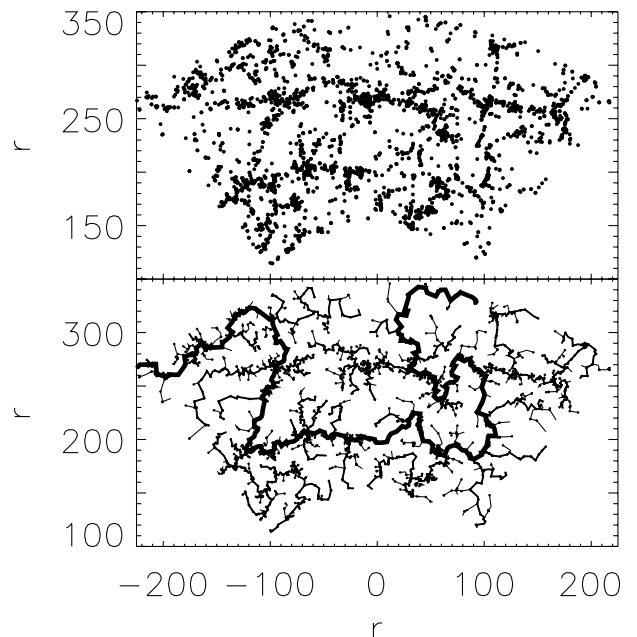
Figure 1. Top, the distribution of galaxies in the LCRS-3 slice in the distance interval 150 \leq D \leq 350 h^{-1} Mpc. Note the relative lack of apparent radial selection effects owing to the moderate flatness of the LCRS selection function over this interval. Bottom, the minimal spanning tree for the above galaxy distribution. The trunk and longer branches of MST are plotted by the thicker lines.
