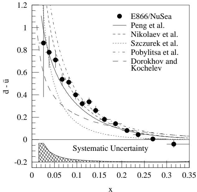
FIG. 15. Comparison of the measured \bar{d}(x) - \bar{u}(x) at Q^2 = 54 \text{ GeV}^2/c^2 to predictions of several models of the nucleon sea. The solid and short-dash curves show pion-cloud calculations by Peng et al. and Nikolaev et al. , respectively. The dotted curve shows the chiral perturbation theory calculation of Szczurek et al. , while the dot-dash curve shows the chiral quark-soliton calculation of Poblitsa et al. The long-dash curve shows the instanton model prediction of Dorokhov and Kochelev.
