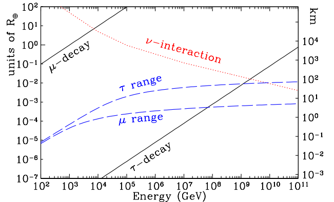
FIG. 1. Some important length scales, in units of Earth radii and km, versus the energy in GeV for the neutrino or charged lepton. Solid lines : the \mu and \tau decay lengths, i.e., the distances over which a fraction e^{-1} of the the initial fluxes would survive (ignoring energy loss). Dashed lines : the \mu and \tau ranges, i.e., the distances in standard rock ( 22 \text{ g mol}^{-1} ) at a density 8 \text{ g cm}^{-3} over which they would be fully stopped by their electromagnetic interactions (ignoring decays). Dotted line : the neutrino interaction length (the same for all flavors), i.e., the distance at a density 8 \text{ g cm}^{-3} over which a fraction e^{-1} of the initial flux would survive. With the exception of the Glashow resonance for \bar{\nu}_e at 6.3 PeV, this figure is the same for antiparticles. While the density varies significantly with nadir angle, 8 \text{ g cm}^{-3} is representative.
