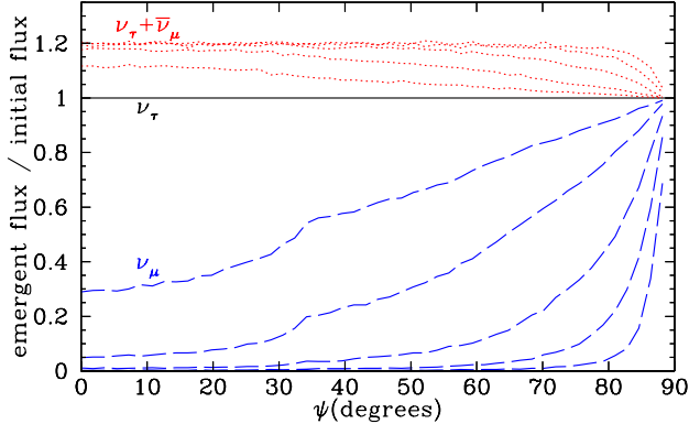
FIG. 2. The surviving fluxes associated with the initial \nu_\tau and \nu_\mu fluxes versus nadir angle, for a variety of energies. The results were calculated with our Monte Carlo code, and the slight jaggedness in the curves is due to statistical fluctuations. The initial \nu_\mu flux is depleted ( \nu_e would be the same), and the flux associated with the initial \nu_\tau is increased due to the secondary \bar{\nu}_\mu (and the equal \bar{\nu}_e component, not shown). The initial energies are 10^5 , 10^6 , 10^7 , 10^8 , and 10^9 GeV, going from top to bottom for the \nu_\mu fluxes and bottom to top for the \nu_\tau + \bar{\nu}_\mu fluxes. The emergent \nu_\tau flux is unity for all energies. We use the density profile given in the Preliminary Reference Earth Model described in, e.g., Ref. [8]. Note the mantle-core transition at \psi \simeq 33^\circ , corresponding to a radial distance of 3480 km.
