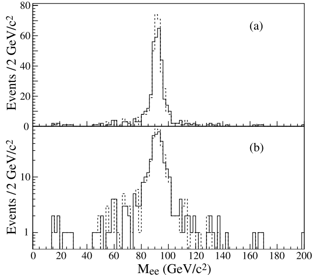
FIG. 1: Z(\rightarrow ee) + 2j data before (solid) and after (dashed) reverteching: (a) has a linear scale and illustrates the improvement in the Z -boson mass resolution after the reverteching; (b) has a logarithmic scale and shows the suppression of the background from vertex misidentification in the tails of the Z -boson peak.
