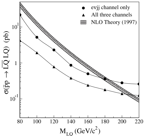
FIG. 18: The 95% C.L. upper limits on the cross sections for scalar leptoquark pair production from the e\nu jj channel, and for all three channels combined, for \beta = \frac{1}{2} , compared to the NLO prediction, as a function of leptoquark mass.
