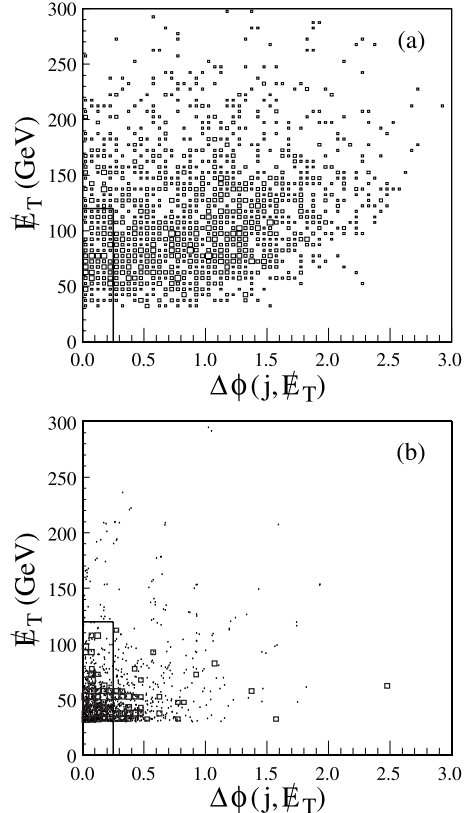
FIG. 13: Effect of the requirement of acolinearity in \cancel{E}_T on (a) a 180 \text{ GeV}/c^2 MC leptoquark signal and (b) the multijet background. In (b), the dots show the distribution before imposition of the M_T^{e\nu} requirement; the open squares show the distribution after applying the M_T^{e\nu} requirement. The acolinearity requirement is indicated by the solid lines.
