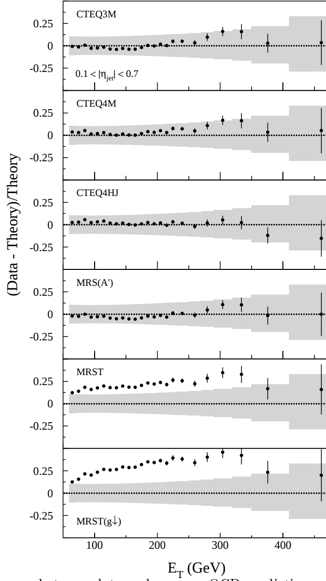
FIG. 54. The difference between data and JETRAD QCD predictions normalized to predictions for 0.1 < |\eta| < 0.7 . The error bars show the statistical uncertainties. The shaded region represents the \pm 1\sigma systematic uncertainties about the prediction.
