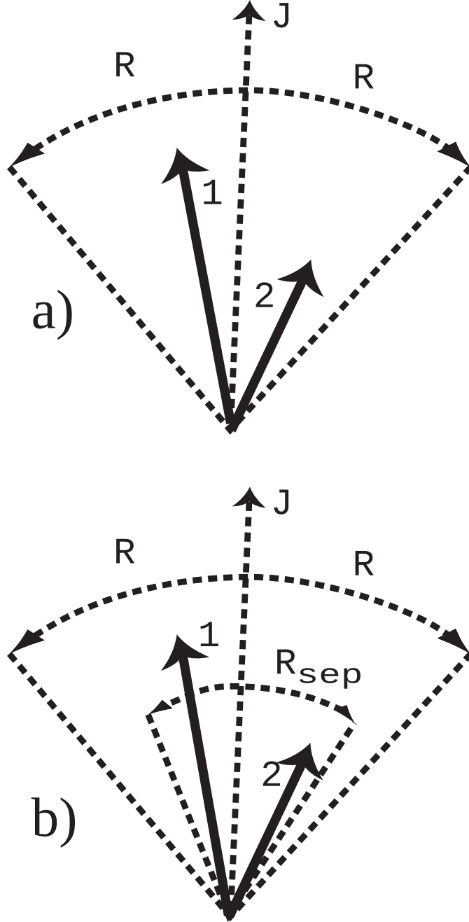
FIG. 4. Illustration and description of the jet definitions at NLO parton level as used by the DØ experiment. a) The jet definition in NLO according to Snowmass. Parton -1- and -2- are combined into jet -J-, if the parton distance to the jet axis is less than R . The jet axis is defined by partons 1 and 2, according to the Snowmass definition. b) The jet definition in NLO according to the modified Snowmass with R_{\text{sep}} . Use the standard Snowmass clustering, but in addition require the distance between the two partons to be less than R_{\text{sep}} .
