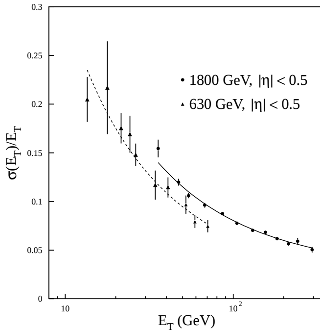
FIG. 34. The single jet resolutions at \sqrt{s} = 630 GeV (triangles) and 1800 GeV (circles). The resolutions at the two center-of-mass energies have been fitted separately to Eq. 10.2. The fit to the \sqrt{s} = 1800 GeV data is the solid line, and the fit to the \sqrt{s} = 630 GeV data is the dashed line.
