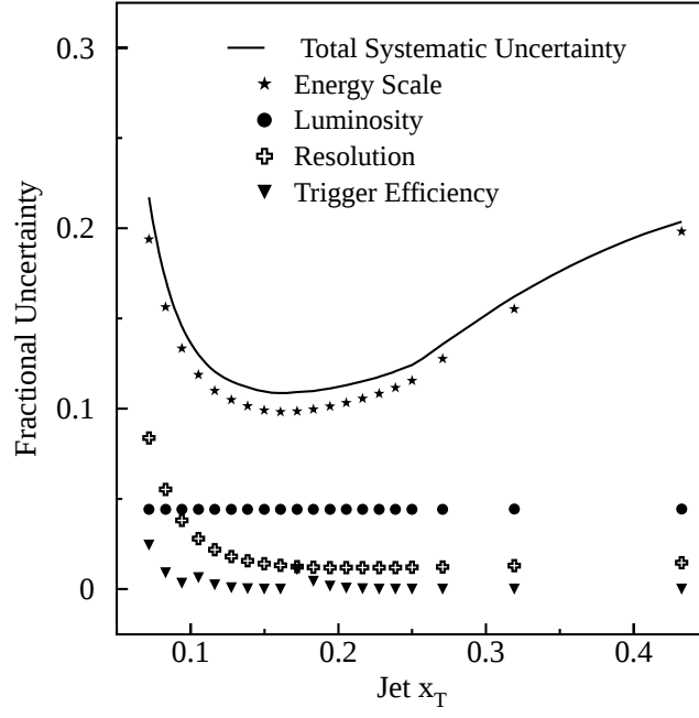
FIG. 59. Contributions to the |\eta| < 0.5 at \sqrt{s} = 630 GeV cross section uncertainty plotted by component.
