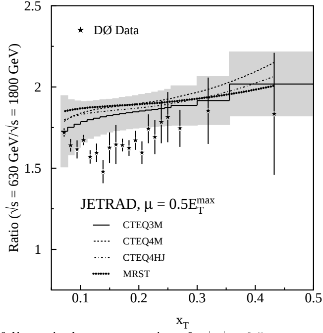
FIG. 66. The ratio of dimensionless cross sections for |\eta| < 0.5 compared with JETRAD predictions with \mu = 0.5E_T^{\max} and the CTEQ3M, CTEQ4M, CTEQ4HJ, and MRST PDFs. The shaded band represents the \pm 1\sigma systematic uncertainty band about the prediction.
