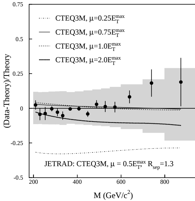
FIG. 94. The difference between the data and the prediction (JETRAD) divided by the prediction for |\eta^{\text{jet}}| < 1.0 . The solid circles represent the comparison to the calculation using CTEQ3M with \mu = 0.5E_T^{\text{max}} . The shaded region represents the \pm 1\sigma systematic uncertainties about the prediction. The effects of changing the renormalization scale are also shown (each curve shows the difference between the alternative prediction and the prediction using CTEQ3M with \mu = 0.5E_T^{\text{max}} ).
