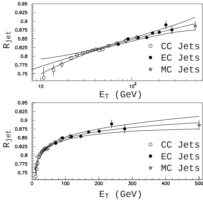
FIG. 24. R_{\text{jet}} versus energy for the \mathcal{R} = 0.7 cone jet algorithm. The solid lines are the fit and the associated uncertainty band.
