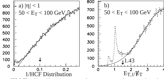
FIG. 16. a) The 1/\text{HCF} distribution. The arrow shows the location of the cut for \sqrt{s} = 1800 GeV. b) The distribution of E_T^{\text{jet1}}/\cancel{E}_T . The arrow at E_T^{\text{jet1}}/\cancel{E}_T = 1.43 corresponds to the \cancel{E}_T/E_T^{\text{jet1}} cut of 0.7. The peak at 1.0 is due to contamination from cosmic rays and the Main Ring. The dashed histograms show the distributions for the full data samples.
