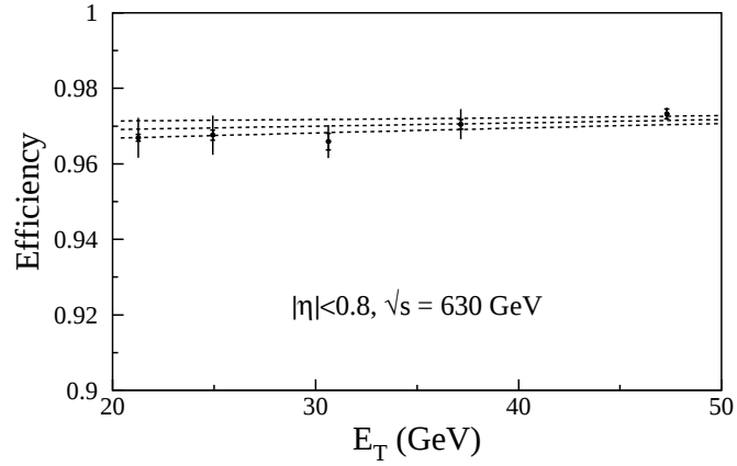
FIG. 19. The efficiency of the standard jet quality cuts for |\eta| < 0.8 at \sqrt{s} = 630 \text{ GeV} (Eqs. 8.6, 8.7, and 8.8). The three curves show the fit to the efficiencies and the uncertainty in the fit.
