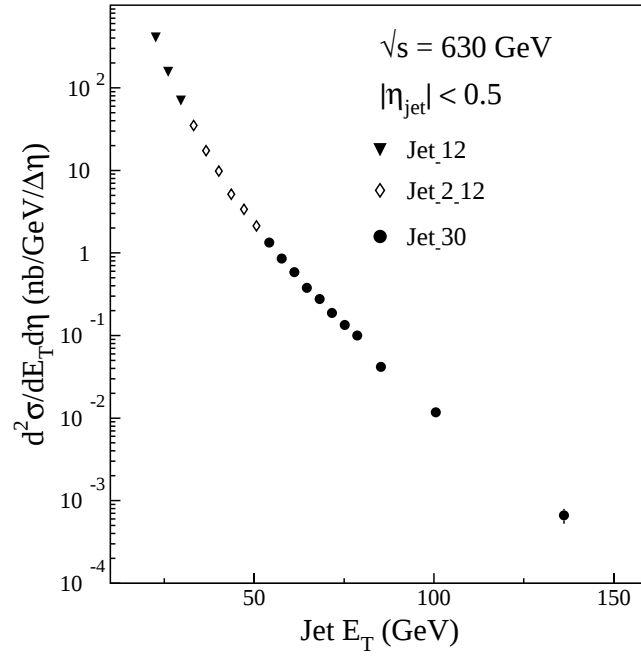
FIG. 56. The observed inclusive jet cross section for \sqrt{s} = 630 GeV. Symbols indicate the three jet triggers (shaded triangles: Jet_12; hollow diamonds: Jet_2_12; shaded circles: Jet_30).
