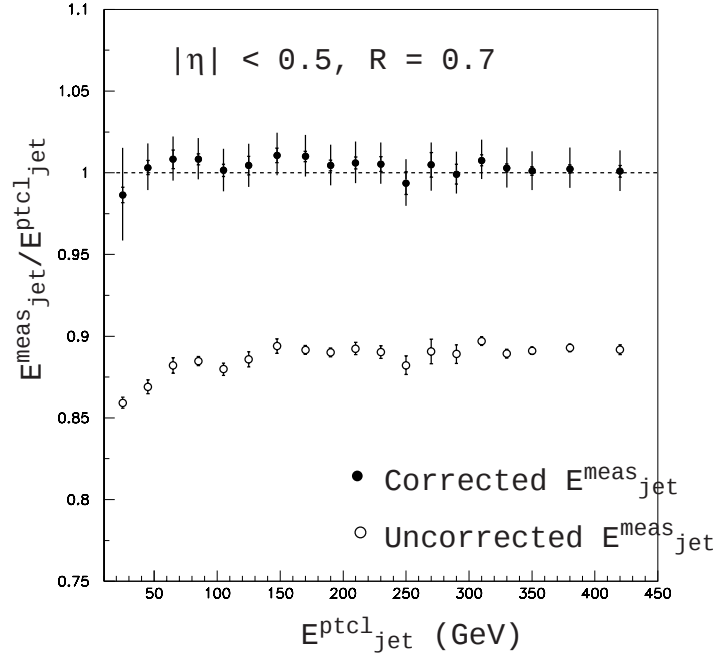
FIG. 26. Monte Carlo verification test. Corrected E_{\text{jet}}^{\text{meas}} / E_{\text{jet}}^{\text{ptcl}} ratio is consistent with 1.0 within errors. The inner error bars depict the statistical error due to the size of the Monte Carlo sample, and the outer error bars represent the systematic uncertainty on the energy scale.
