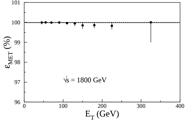
FIG. 18. The efficiency of the E_T cut used in the dijet analyses at \sqrt{s} = 1800 \text{ GeV} (Eq. 8.4).
