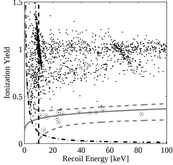
FIG. 1. Ionization yield ( Y ) vs. recoil energy for veto-anticoincident single scatters contained in the inner electrodes of the 3 uncontaminated Ge detectors. Solid curve: expected position of nuclear recoils. Dashed curves: nominal 90% nuclear-recoil acceptance region. Dashed line: 10 keV analysis threshold. Dashed-dotted curve: threshold for separation of ionization signal from amplifier noise. Circled points: nuclear recoils. The presence of 3 events just above the acceptance region is compatible with 90% acceptance.
