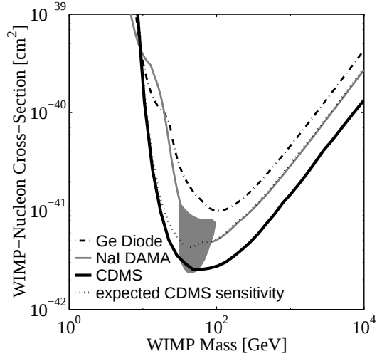
FIG. 4. Spin-independent \sigma vs. M . The regions above the curves are excluded at 90% CL. Solid dark curve: limit from this analysis. Dotted curve: CDMS expected sensitivity (median simulated limit) given the observed neutron background. Because the number of multiple scatters observed is larger than expected, the limit from this analysis is lower than the median simulated limit. Solid light curve: DAMA limit using pulse-shape analysis [27]. Shaded region: DAMA 3\sigma allowed region as described in text [25]. Dashed-dotted curve: Ge diode limit, dominated by [28]. All curves are normalized following [11], using the Helm spin-independent form-factor, A^2 scaling, WIMP characteristic velocity v_0 = 220 \text{ km s}^{-1} , mean Earth velocity v_E = 232 \text{ km s}^{-1} , and \rho = 0.3 \text{ GeV c}^{-2} \text{ cm}^{-3} .
