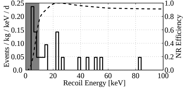
FIG. 2. Solid: histogram of nuclear recoils observed in the inner electrodes of the 3 uncontaminated Ge detectors (left-hand scale). Shaded: 10 keV analysis threshold. Dashed: peak-normalized nuclear-recoil efficiency (right-hand scale).
