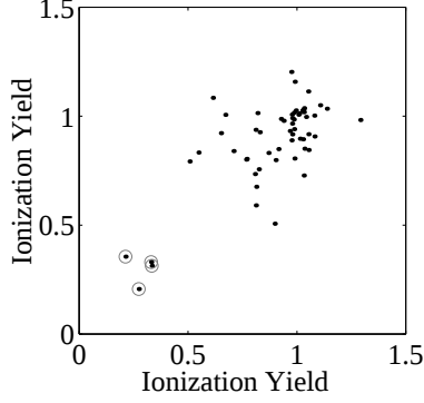
FIG. 3. Scatter plot of ionization yields for multiple scatters in the 3 uncontaminated Ge detectors with at least 1 inner-electrode scatter and both scatters between 10 and 100 keV. Circled events are tagged as nuclear recoils in both detectors. Bulk recoils and surface events lie at Y \simeq 1 and Y \sim 0.75 , respectively.
