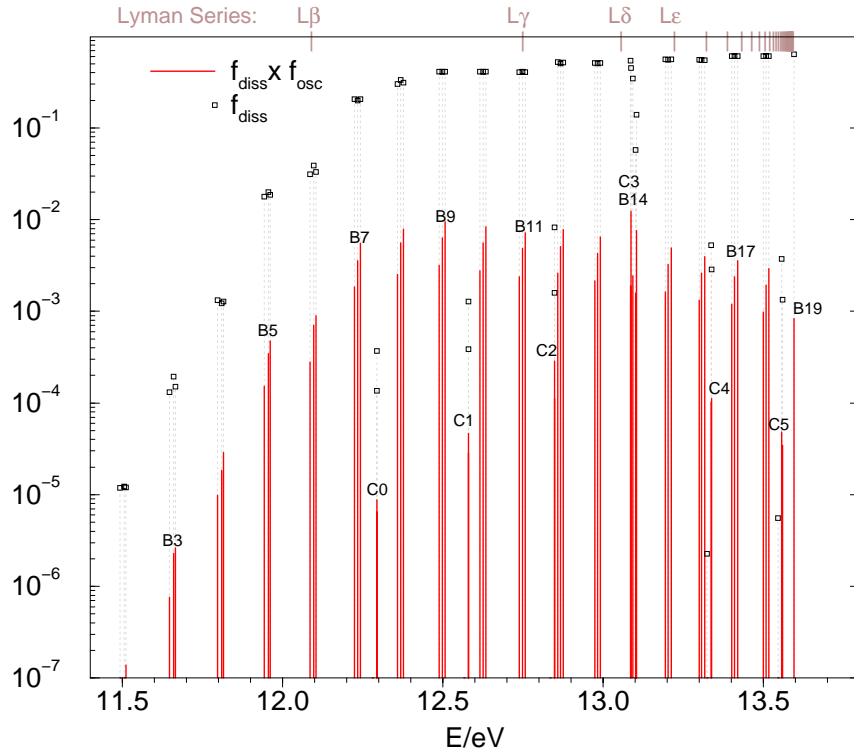
Fig. A16.— The relevant Lyman Werner bands for intergalactic H 2 photo-dissociation. The solid columns indicate the value of f_{diss} \times f_{osc} and the dotted ones show the dissociation fractions. Lines of the Lyman (Werner) system are labeled by B v' (C v' ) where v' is the vibrational quantum number of the excited state. The location of the atomic hydrogen Lyman series are indicated on the top of the graph.
