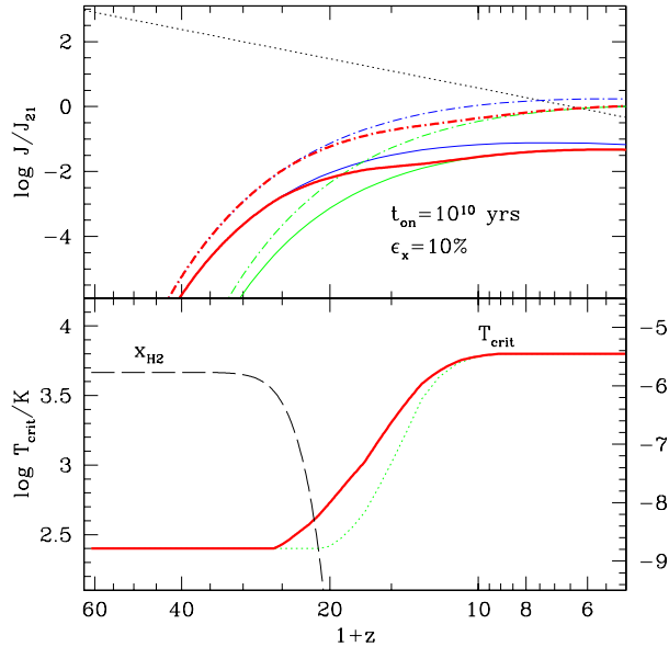
Fig. 10.— Same as Figure 7, but assuming t_{\text{on}} = 10^{10} \text{ yrs} .
