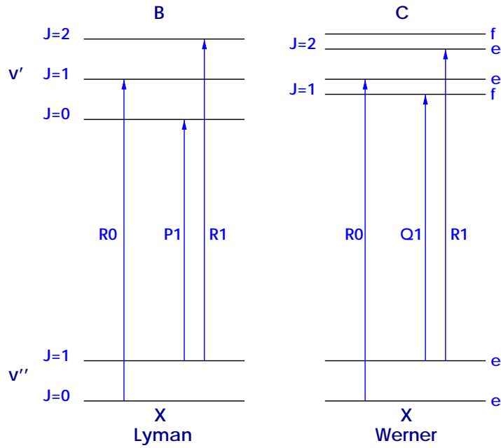
Fig. A15.— Illustration of all possible absorption lines from the lowest energy states of ortho and para H 2 .
