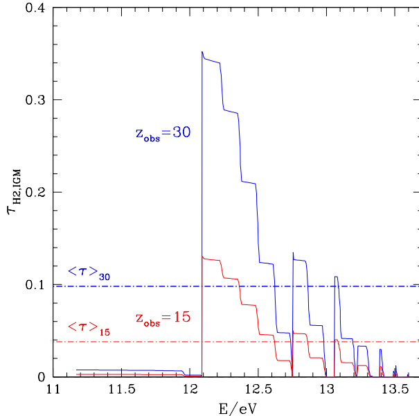
Fig. 2.— The total \text{H}_2 optical depth of the IGM for an observer at redshift z = 30 and z = 15 . We assume a constant fixed x_{\text{H}_2} = 2 \times 10^{-6} , and sum the optical depth of the Lyman-Werner lines of \text{H}_2 . At each observed frequency, we only include sources between z_{\text{obs}} and the nearest atomic Lyman resonance. The dashed lines show the effective optical depths averaged in the 11.18–13.6 eV range.
