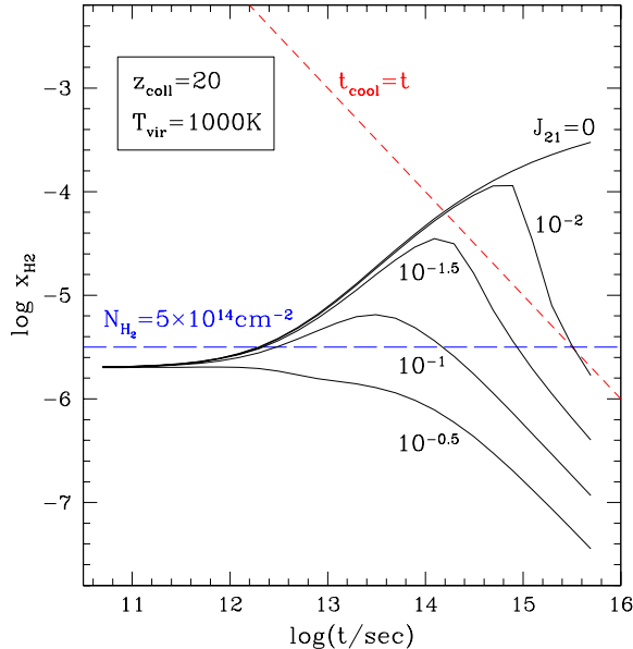
Fig. 5.— Evolution of the \text{H}_2 abundance in the core of the singular isothermal sphere shown in Figure 4; in the presence of various UV background fluxes (solid lines). Also shown is the \text{H}_2 abundance at which the cooling time equals the time elapsed since the collapse of the cloud (short dashed line); and the \text{H}_2 abundance at which the LW lines would become self-shielding (at an integrated \text{H}_2 column density of 5 \times 10^{14} \text{ cm}^{-2} , long dashed line). For J > 10^{-1.5} the cloud becomes self-shielding, but still cannot cool fast enough.
