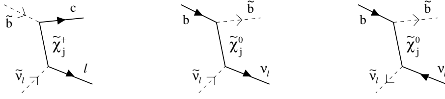
Figure 1. Semileptonic sbottom decay (left) and the decays b \rightarrow \tilde{b}\nu_l\tilde{\nu}_l^* (center) and b \rightarrow \tilde{b}\bar{\nu}_l\tilde{\nu}_l (right). l represents e or \mu .
