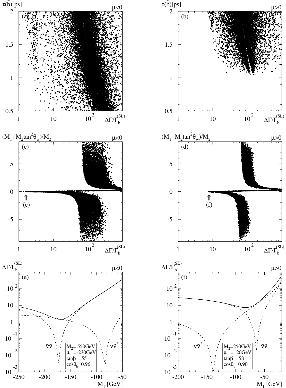
Figure 2. The contribution of b \rightarrow \tilde{b} + \mathbb{E} \rightarrow cl\mathbb{E} to the semileptonic b decay in 20000 MSSM scenarios, all fulfilling the relaxed sbottom lifetime requirement of \tau_{\tilde{b}} < 2 \text{ ps} (left: \mu < 0 , right: \mu > 0 ). The SUSY bottom decay width is plotted versus the sbottom lifetime (a,b) and versus the relevant combination of gaugino masses (c,d). For two particular parameter points the variation of the different decay channels with M_1 is shown (e,f).
