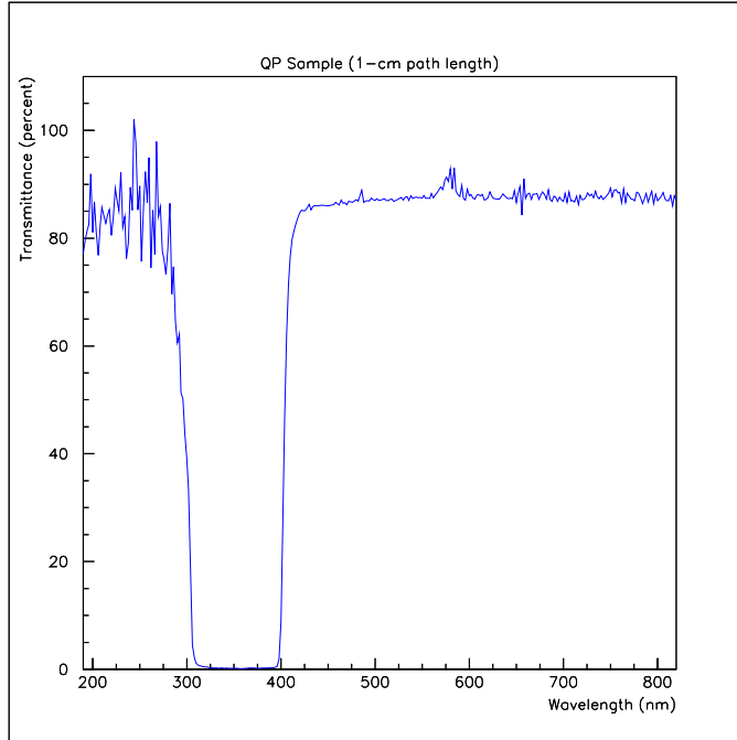
Fig. 4. Transmittance data of extruded plastic scintillator.
