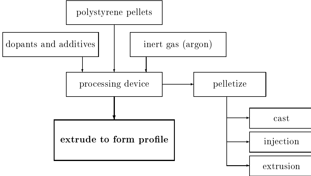
Fig. 8. Continuous in-line coloring and extrusion process (Method 2).
