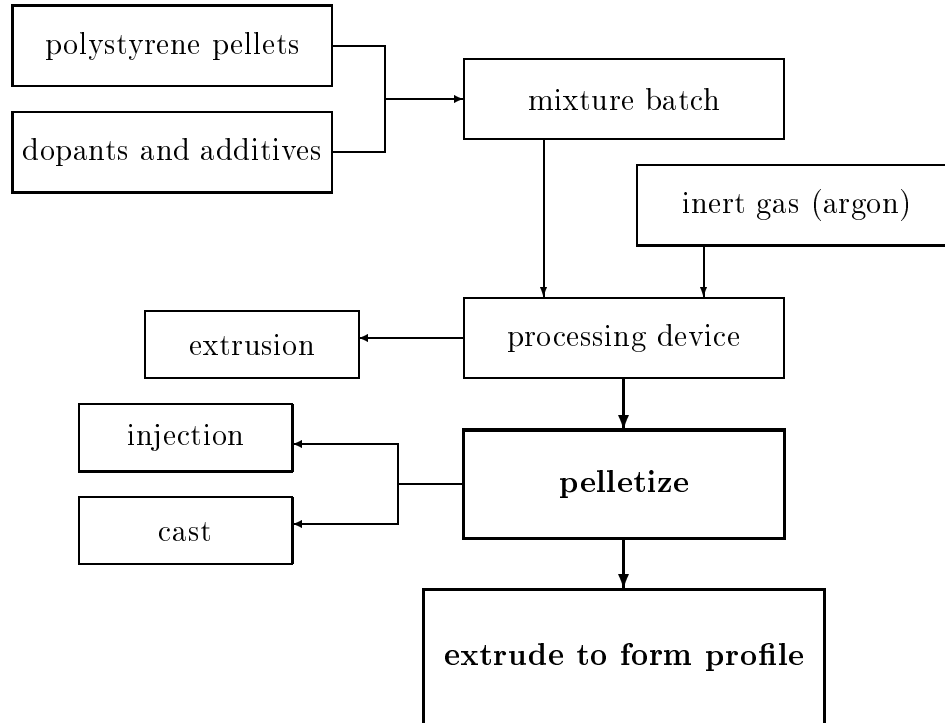
Fig. 5. Two-step process: batch coloring and extrusion (Method 1).
