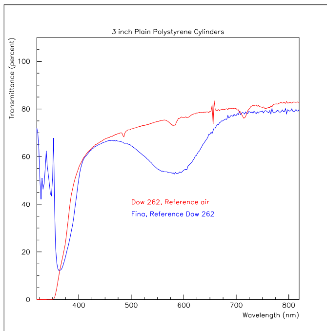
Fig. 3. Transmittance data of commercial polystyrene pellets.
