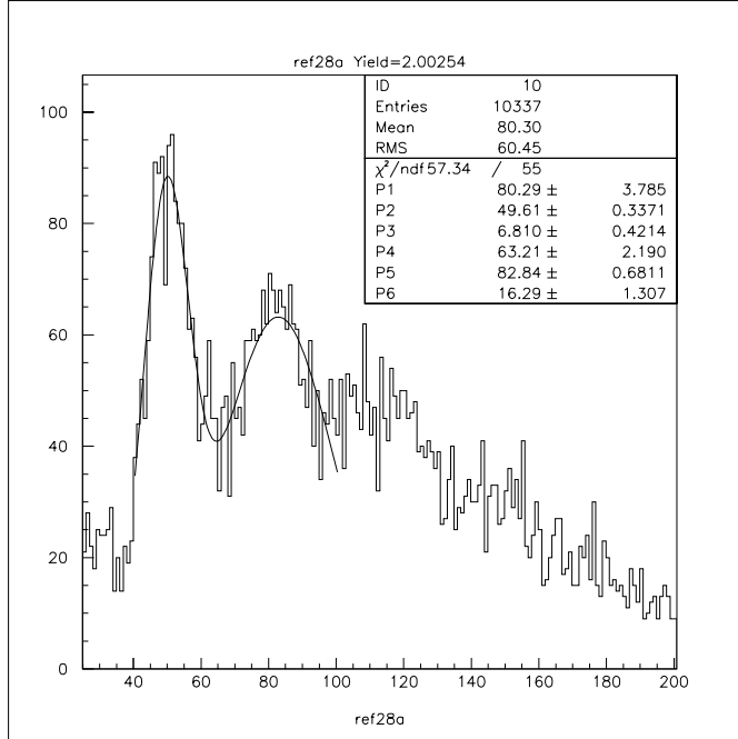
Fig. 9. Light yield distribution of extruded blue plastic scintillator with green WLS fiber.
