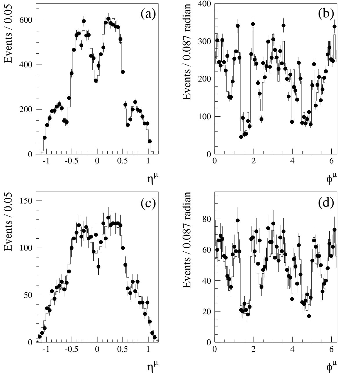
Figure 3.7: The \eta and \phi distributions of muons are shown in (a) and (b) for W decays, and (c) and (d) for Z decays. Points (histograms) show the data (the simulation) with statistical uncertainties.
