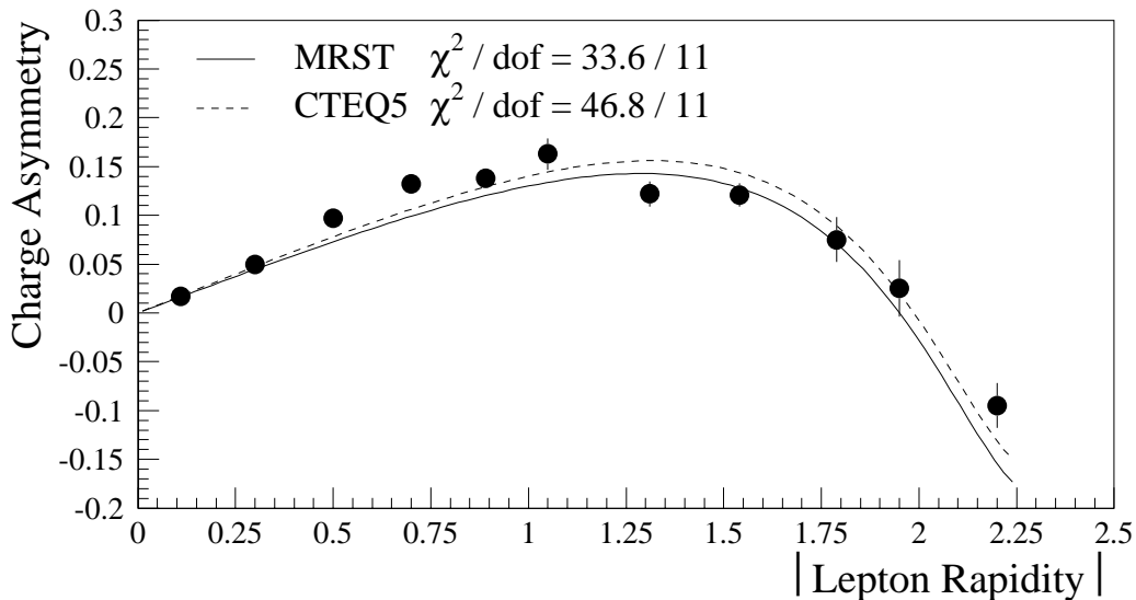
Figure 6.1: The CDF W lepton charge asymmetry measurement compared to predictions using the DYRAD calculations with MRST (solid) and CTEQ-5 (dashed) PDFs.
