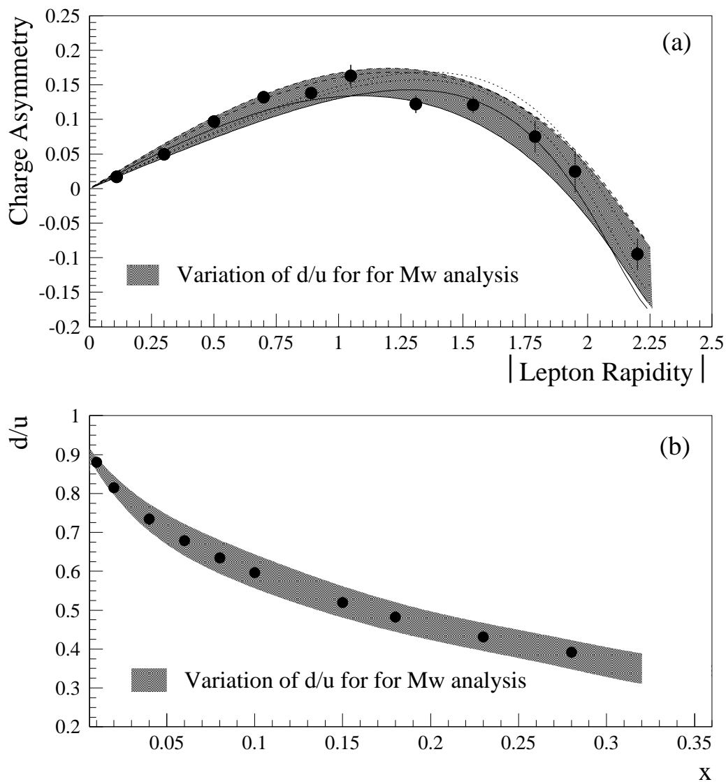
Figure 6.2: (a) The CDF measurement of the W lepton charge asymmetry compared with the six reference PDFs. The upper and lower dotted curves are MRS-R2 and MRS-R2 modified, the upper and lower dashed curves are MRS-R1 modified and MRS-R1, and the upper and lower solid curves in |\eta| < 1 are MRS-T and MRS-T modified, respectively. (b) The NMC d/u data evolved to Q^2 = M_W^2 . The gray bands represent the range spanned by the six reference PDFs.
