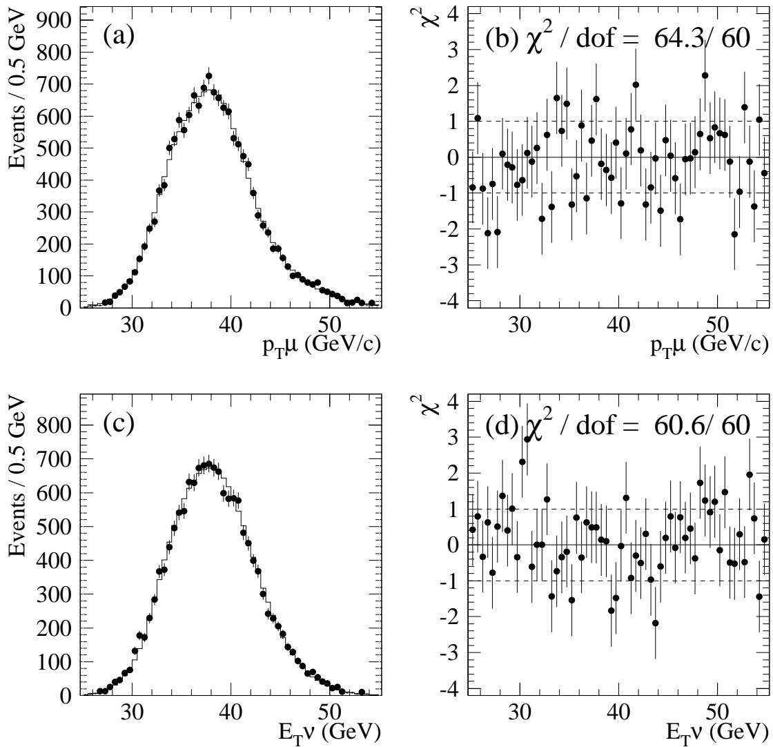
Figure 8.7: (a) p_T distribution of muons and (c) E_T distribution of neutrinos in the W \rightarrow \mu\nu channel. The points are the data and the histograms the best fit simulation. (b) and (d) The difference between the data and simulation normalized by the statistical uncertainty.
