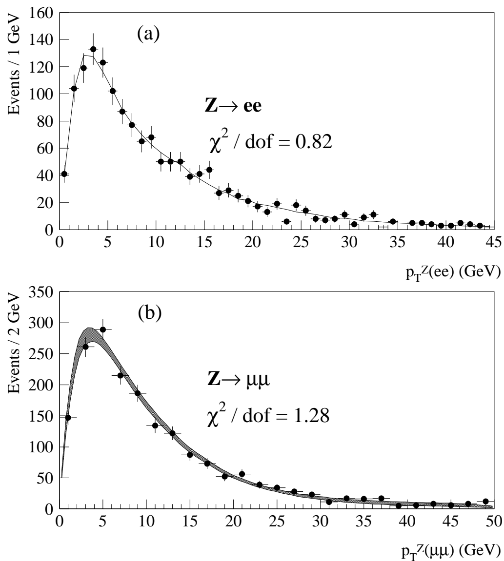
Figure 6.3: The observed Z p_T distributions (points) for the (a) Z \rightarrow e^+e^- and (b) Z \rightarrow \mu^+\mu^- sample are compared with the Monte Carlo simulation (solid line or shaded band) which uses the best fit parameters for the input p_T^Z distribution.
