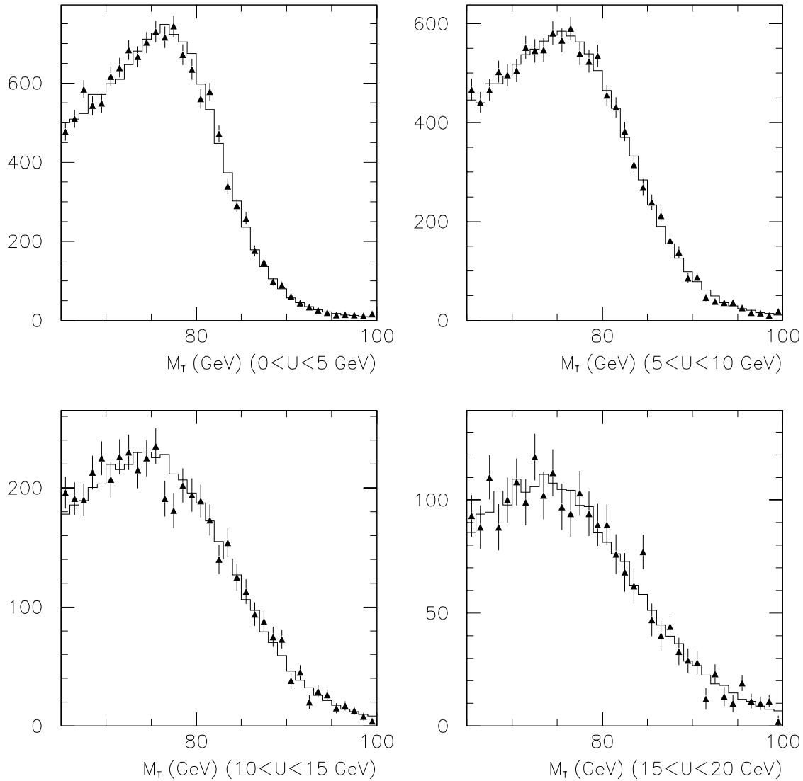
Figure 8.8: Transverse mass distributions in bins of |\mathbf{u}| for the W \rightarrow e\nu data (triangles) and the best fit simulation (histograms). The four |\mathbf{u}| bins are, 0 < |\mathbf{u}| < 5 GeV (Top Left), 5 < |\mathbf{u}| < 10 GeV (Top Right), 10 < |\mathbf{u}| < 15 GeV (Bottom Left), and 15 < |\mathbf{u}| < 20 GeV (Bottom Right)
