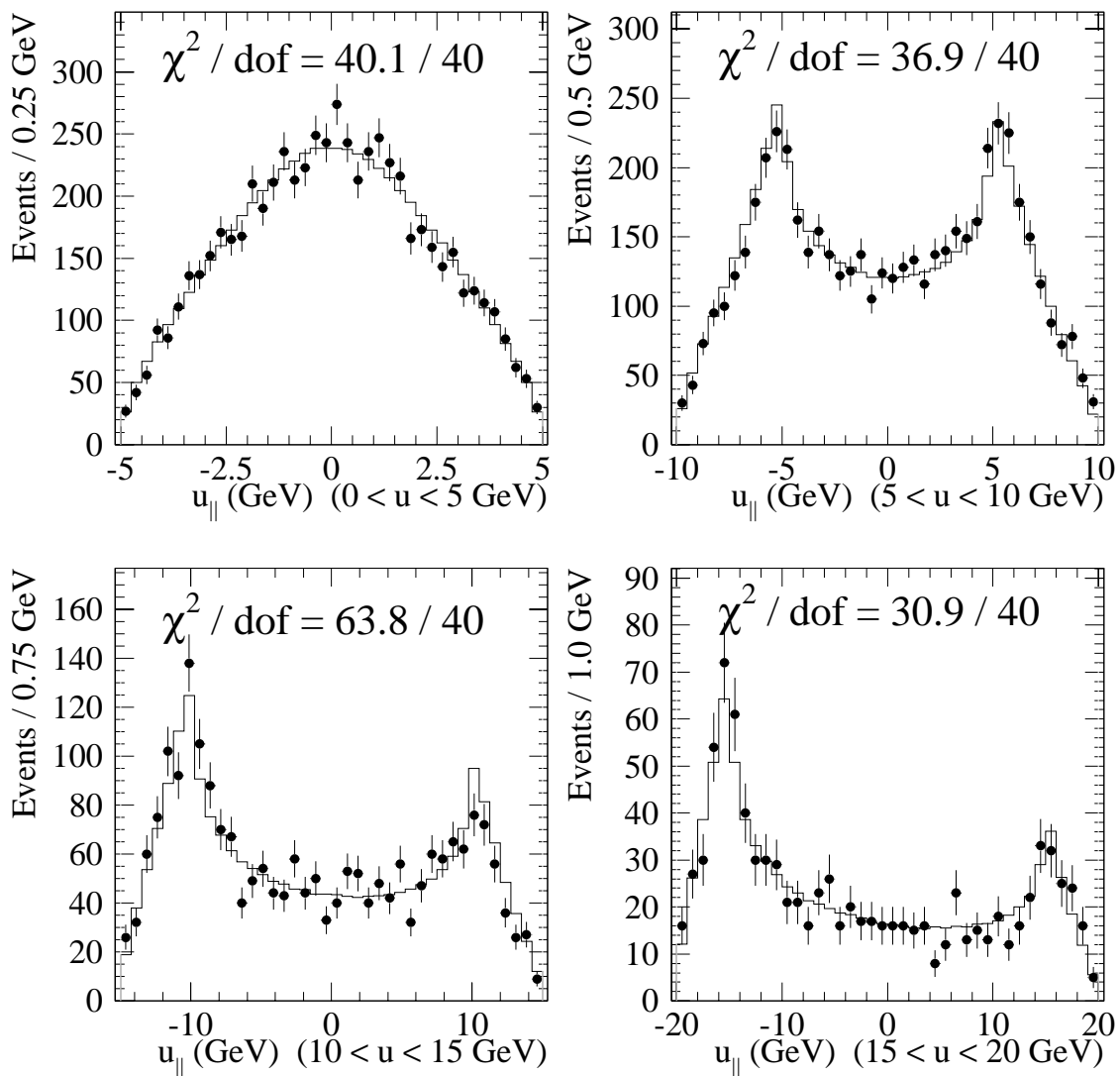
Figure 7.14: The u_{||} distributions for the W \rightarrow \mu\nu sample in four bins of |u| . The points are the data, and the histograms the simulation.
