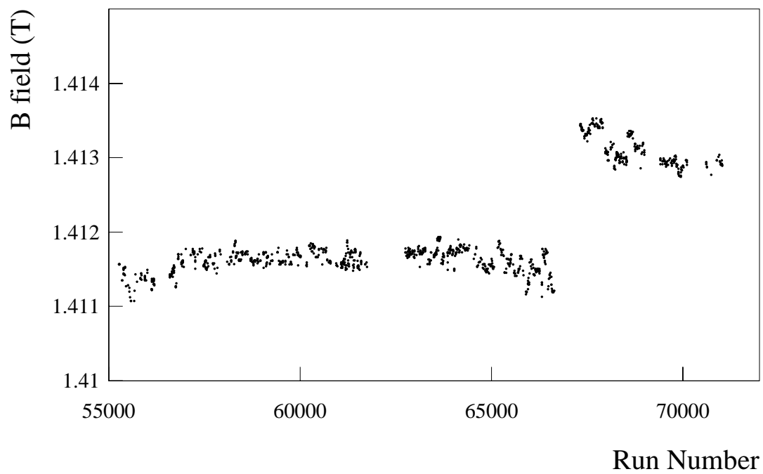
Figure 3.1: Variation of the average magnetic field as a function of run number. The left side of the plot corresponds to January 1994 and the right side of the plot to July 1995.
