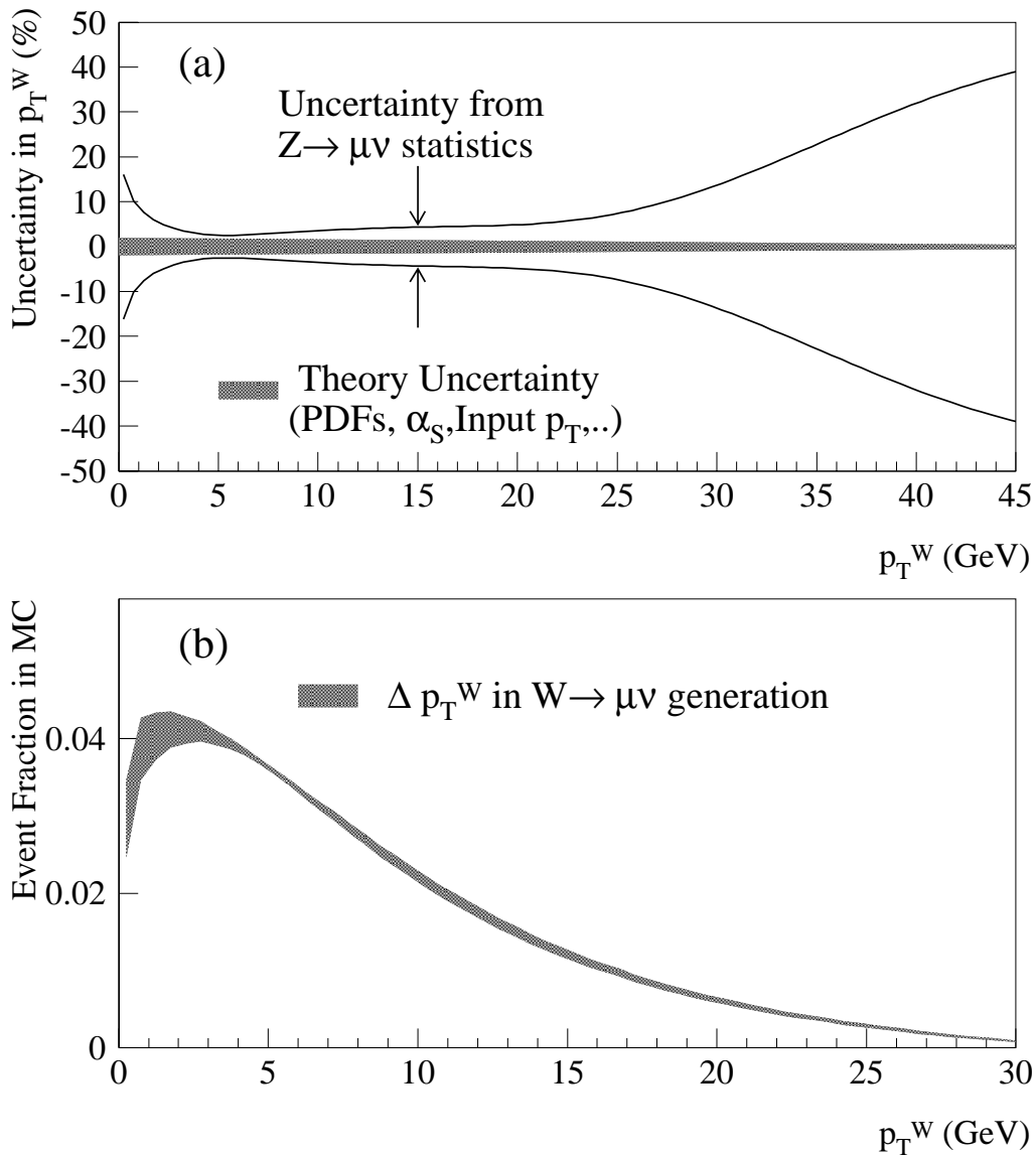
Figure 6.5: (a) The fractional uncertainties on p_T^W as a function of p_T^W . The solid lines show the uncertainty due to the Z statistics and the shaded band the uncertainty due to the theoretical calculations. (b) The p_T^W distribution extracted from the p_T^Z distribution and the theoretical calculations of p_T^W/p_T^Z for the W \rightarrow \mu\nu mass measurement. The band represents the uncertainties.
