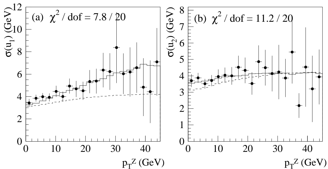
Figure 7.7: \sigma(u_1) and \sigma(u_2) as a function of p_T^Z for the Z \rightarrow \mu^+ \mu^- sample. The points are the data, and the solid histograms are the simulation using the recoil model parameters. The dashed histograms show \sigma_{mbs}(\Sigma E_T) , the resolutions of the underlying energy.
