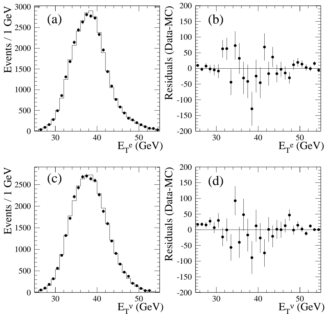
Figure 8.6: E_T distributions of (a) electrons and (c) neutrinos in the W \rightarrow e\nu channel. The points are the data and the histograms the best fit simulation. The differences between the data and simulation are shown in (b) and (d).
