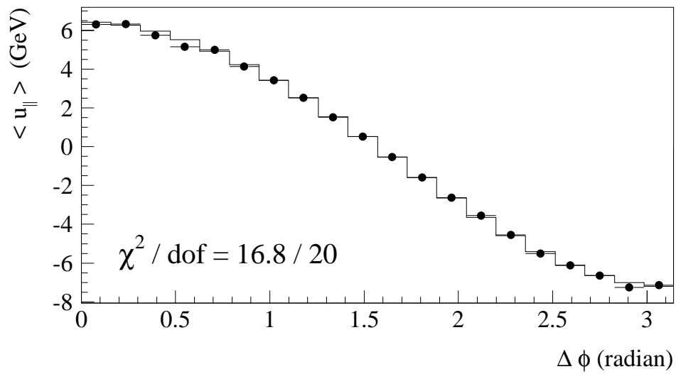
Figure 7.16: \langle u_{\parallel} \rangle as a function of azimuthal angle between the lepton and \mathbf{u} for the W \rightarrow \mu\nu sample. The points are the data and the histogram is the simulation.
