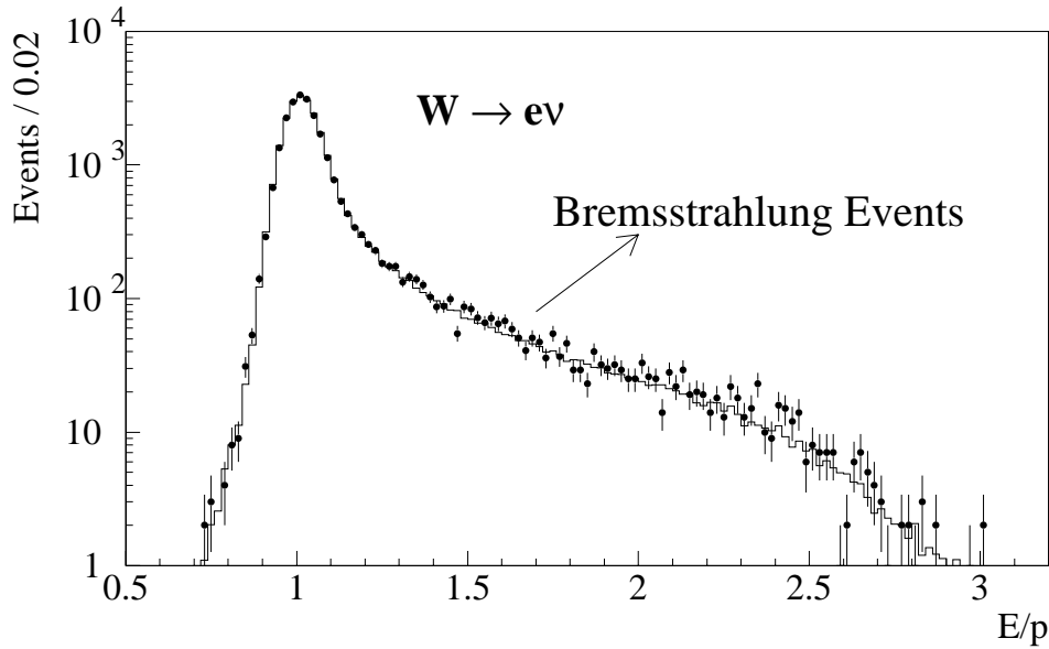
Figure 3.4: E/p distribution of electrons in the W \rightarrow e\nu sample. The histogram indicates the simulation.
