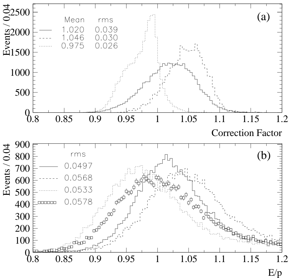
Figure 4.1: (a) Spatial and temporal energy correction factors on the W electrons. The dotted curve shows the spatial corrections only, the dashed curve the temporal corrections only, and the solid curve the product of the two. (b) The E/p distributions of the W electrons after the respective corrections. The squares show the data before any corrections are applied. The improvement in the resolution after correction is apparent.
