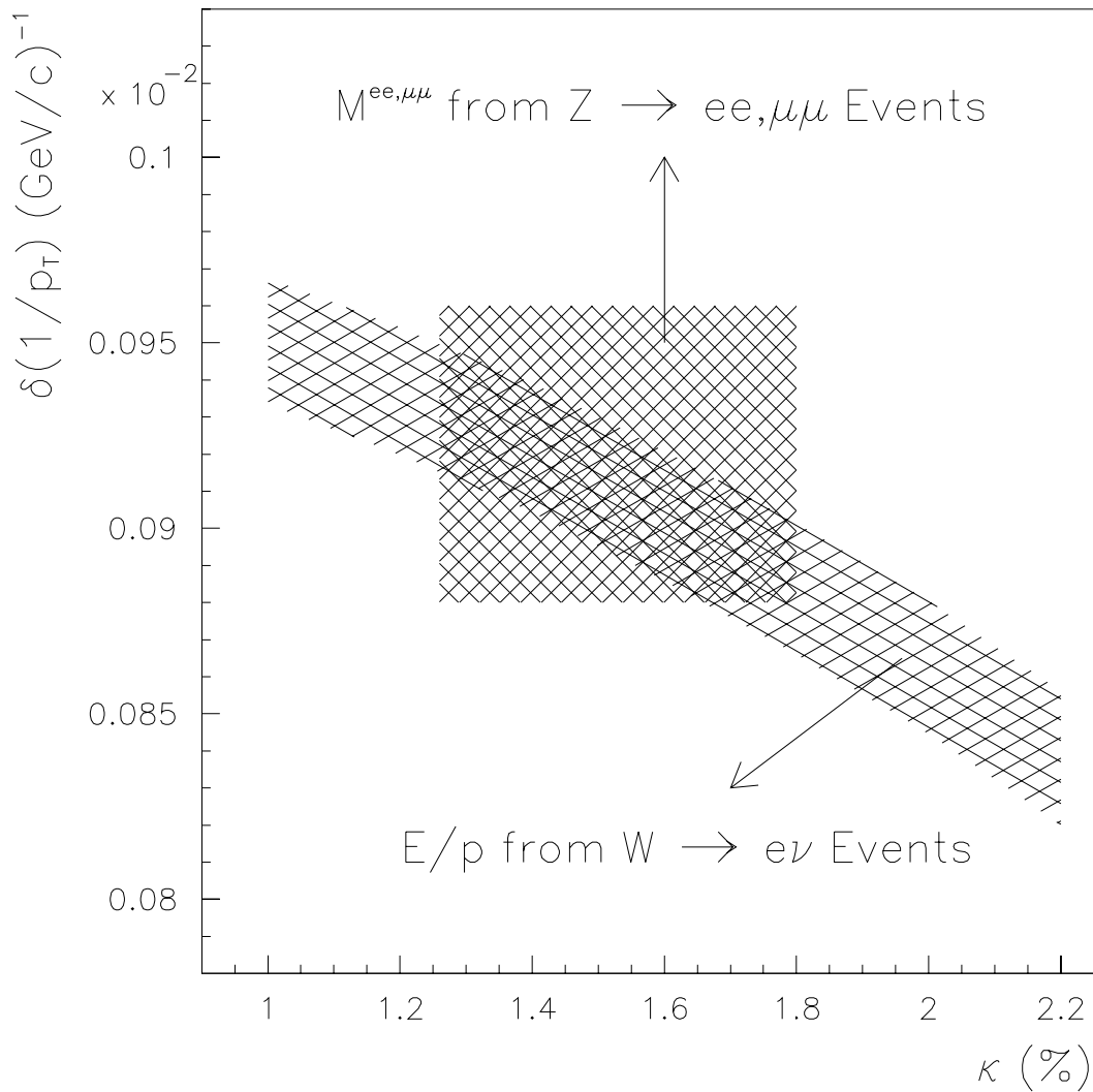
Figure 4.6: The energy resolution \kappa and tracking resolution \delta(1/p_T) as determined from fits to the E/p distribution in W \rightarrow e\nu events, compared to the same resolutions determined from the Z \rightarrow e^+e^- and Z \rightarrow \mu^+\mu^- data.
