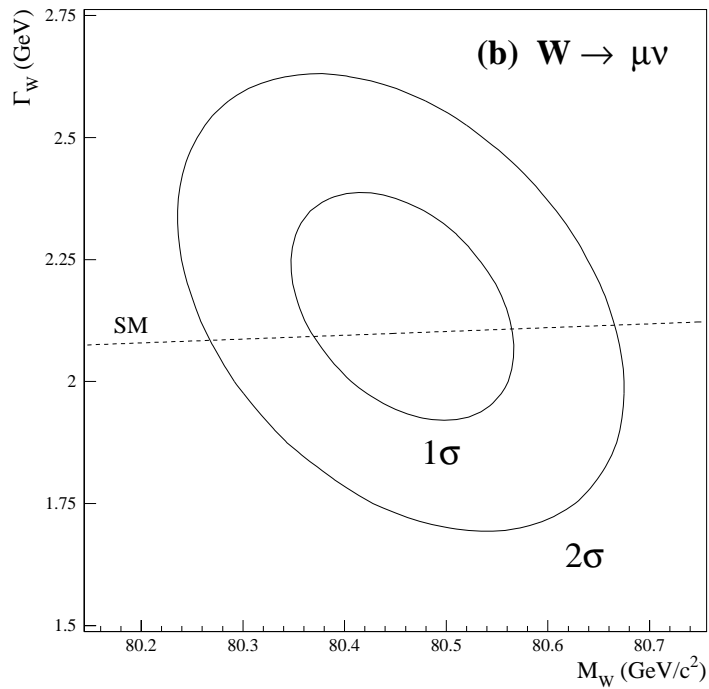
Figure 8.5: The 1\sigma and 2\sigma contours in \Gamma_W versus M_W of the transverse mass fit when the width is floated for (a) the W \rightarrow e\nu channel and (b) the W \rightarrow \mu\nu channel. The dashed lines are the predicted \Gamma_W as a function of M_W .
