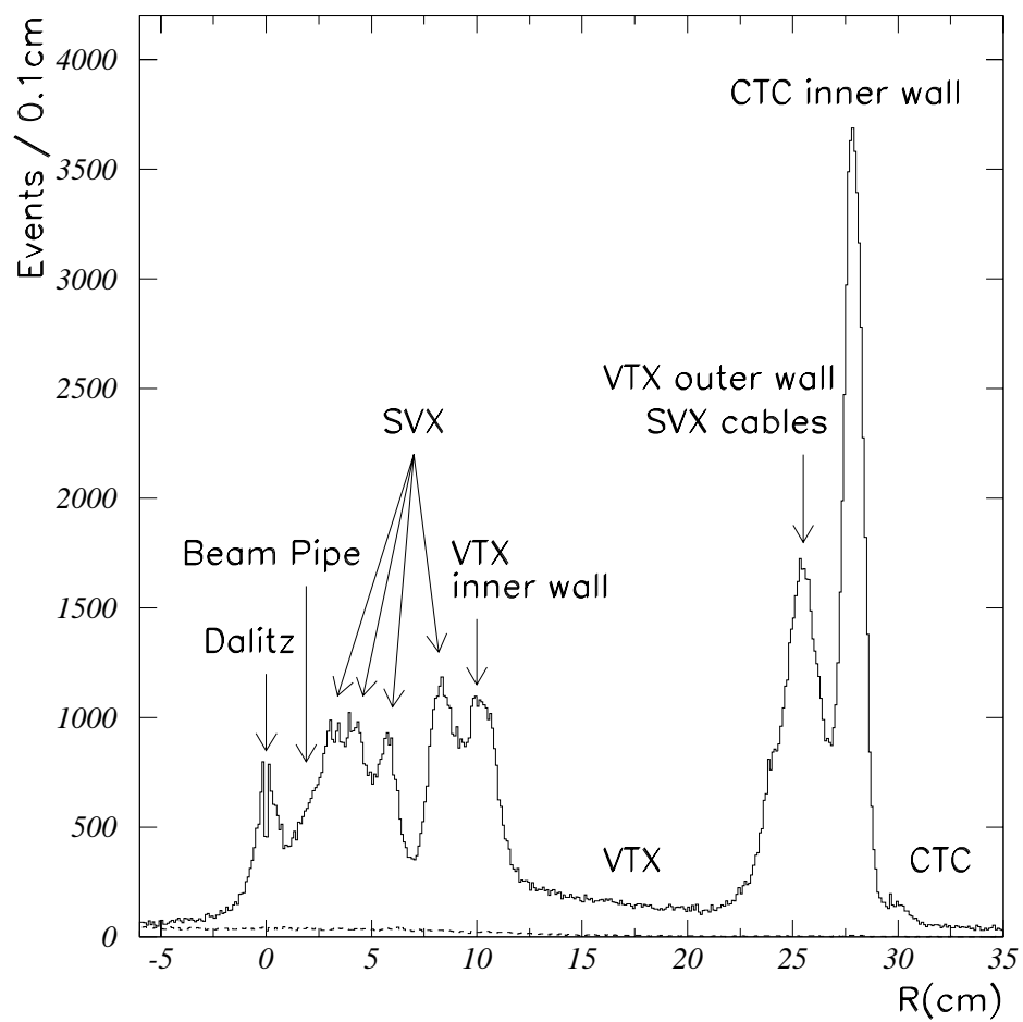
Figure 3.2: The radial ( R ) distributions for conversions (solid line) and background (dashed line) for the Run IA inclusive electron sample. R is negative when the photon momentum direction is opposite to the vector from the beam spot to the conversion position due to the detector resolution.
