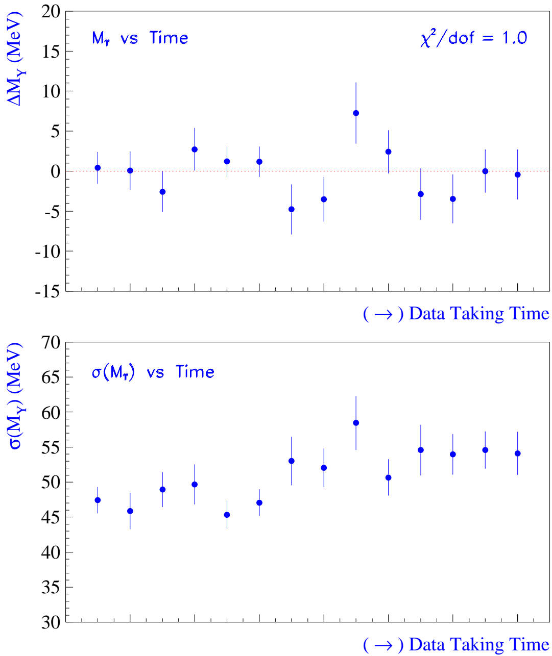
Figure 3.11: Variation of the measured \Upsilon(1S) mass (Top) and width (Bottom) as a function of time. The left side of the plot corresponds to January 1994 and the right side of the plot to July 1995. \Delta M_\Upsilon is difference between the measured mass for a given time period and the mass using all the data.
