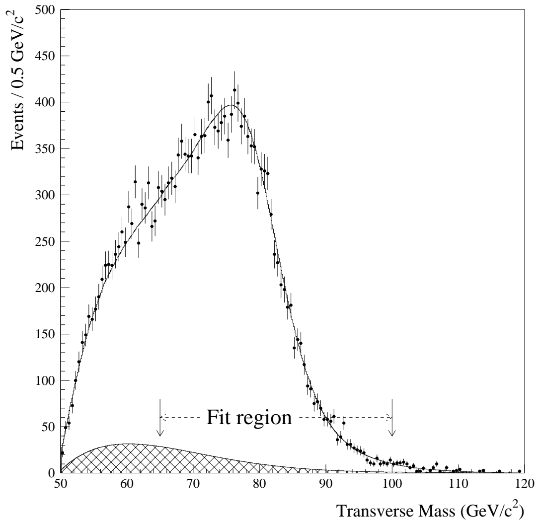
Figure 8.4: W Transverse mass distributions compared to the best fit for the W \rightarrow \mu\nu channel.
