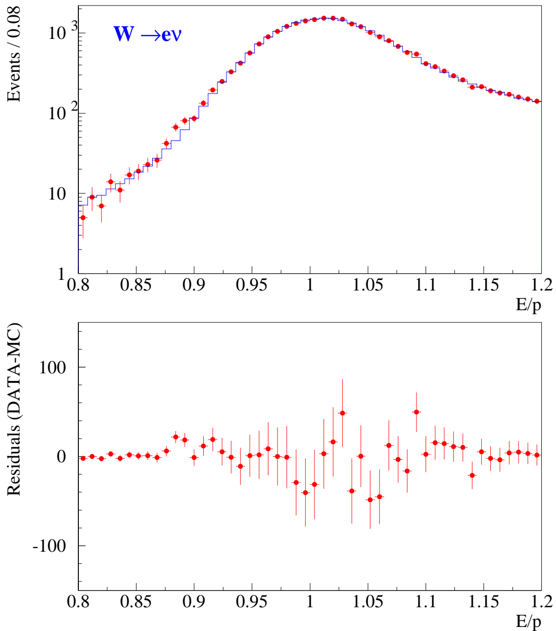
Figure 4.5: Top: E/p distribution for W events (points) and the best Monte Carlo fit. The solid histogram is the Monte Carlo fit normalized to data, and the points are the data. The fit reproduces the shape very well as indicated by the \chi^2/\text{dof}=0.86 . Bottom: The difference between the data and the best fit simulation.
