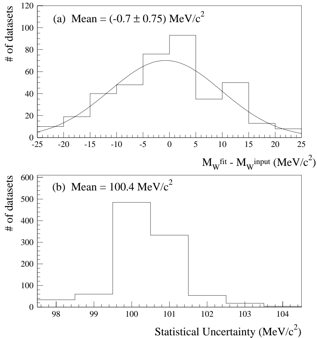
Figure 8.1: (a) Difference between the input M_W values and the returned values by fits to Monte Carlo pseudo-samples. Each sample is 100 times the size of the W \rightarrow \mu\nu data. (b) The (statistical) error returned by fitting 1000 Monte Carlo pseudo datasets of the same size as the W \rightarrow \mu\nu data.
