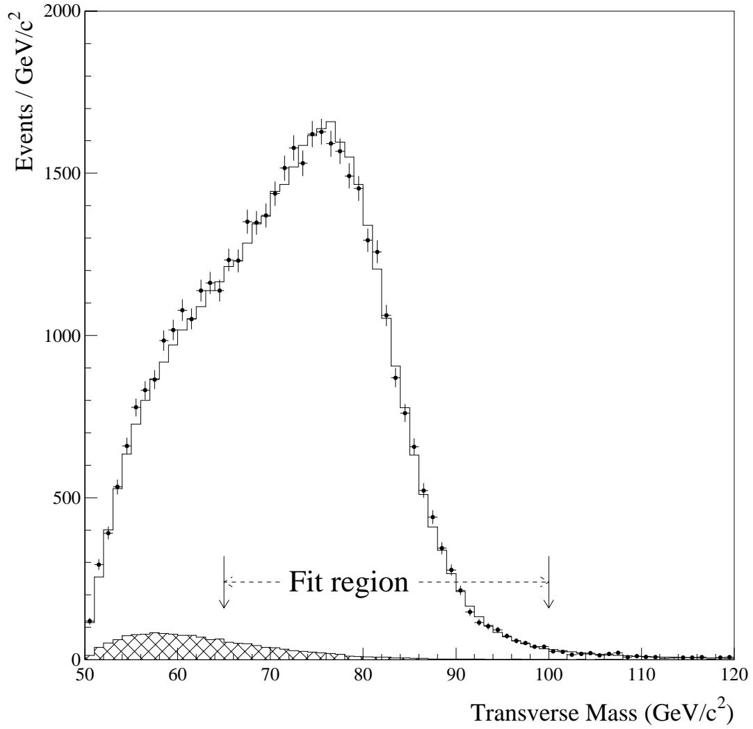
Figure 8.3: W Transverse mass distributions compared to the best fit for the W \rightarrow e\nu channel.
