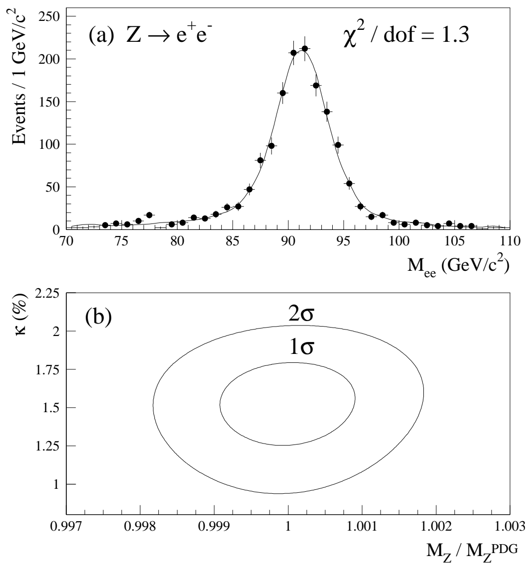
Figure 4.3: Results of fit to Z mass and energy resolution. (a) Invariant mass distribution. The points are the data, and the solid line is the Monte Carlo simulation (normalized to the data) with best fit. (b) Correlation between the scale factor ( S_E ) and the constant term ( \kappa ) in the resolution function.
