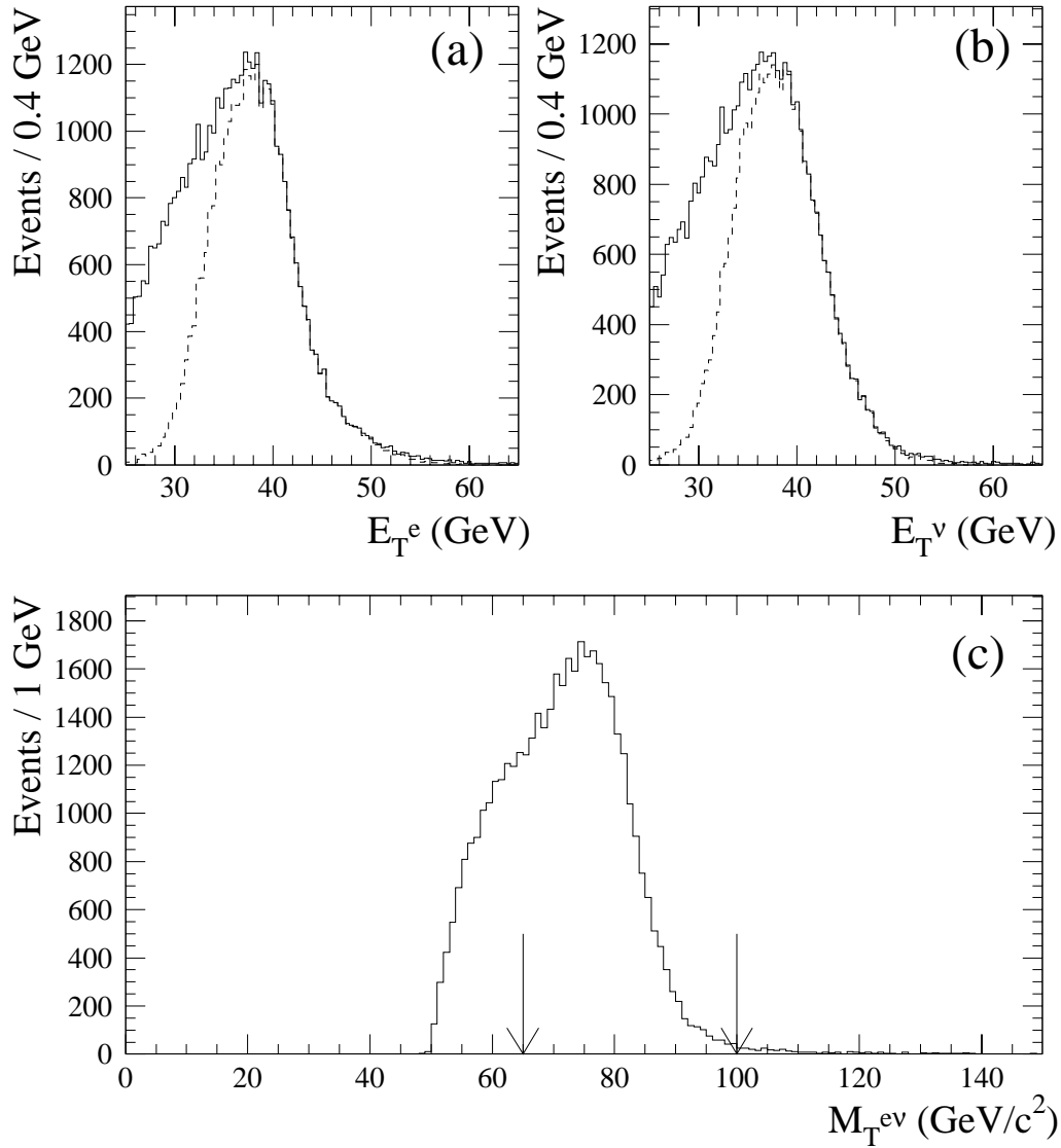
Figure 4.2: Kinematic quantities from the final W \rightarrow e\nu sample. E_T distributions of (a) electrons and (b) neutrinos. The dashed curves show the events in 65 < M_T < 100 GeV, the fit region for the W mass measurement. (c) Transverse Mass distribution. The arrows indicate the region used in the W mass fit.
