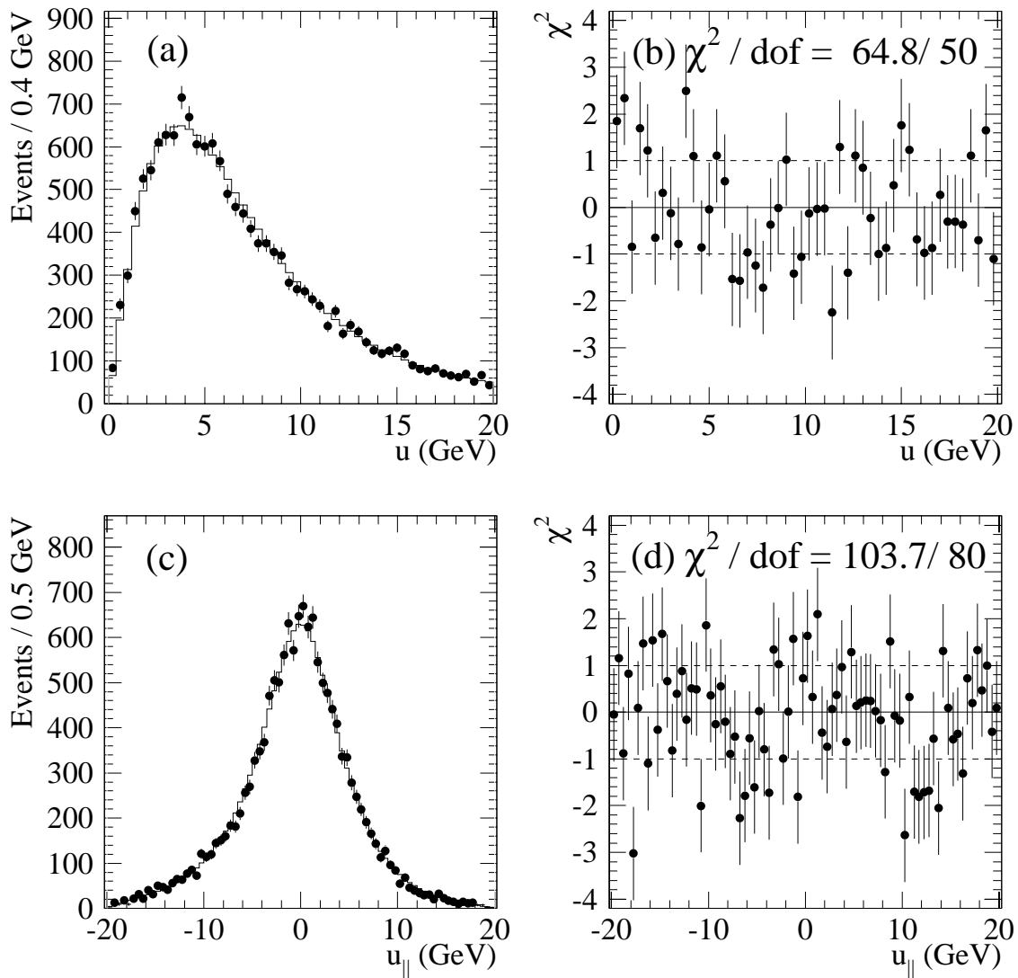
Figure 7.11: The (a) |\mathbf{u}| and (c) u_{\parallel} distribution for the W \rightarrow \mu\nu sample. The points (histograms) are the data (simulation). The differences between the data and the simulation normalized by the statistical uncertainty are shown in (b) and (d).
