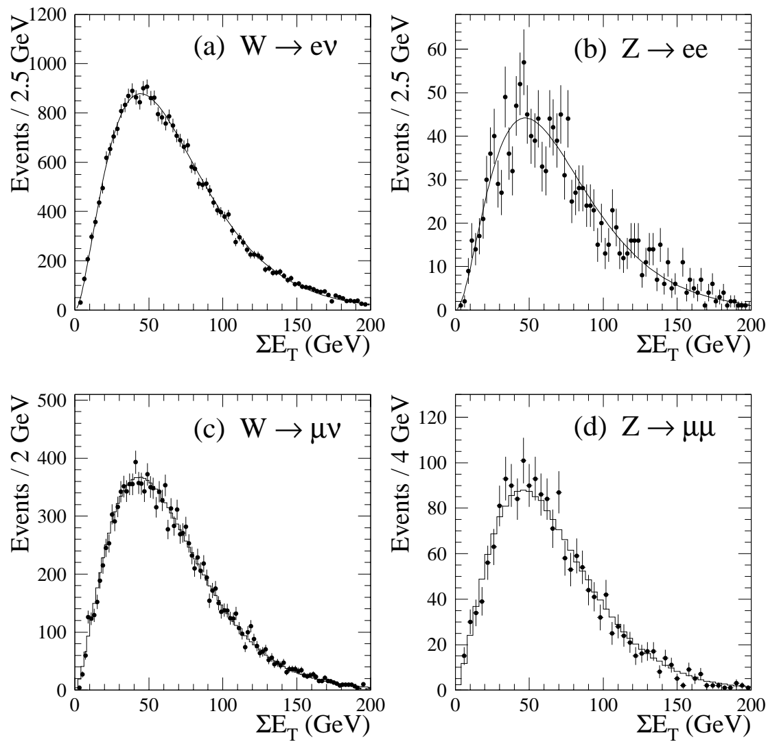
Figure 7.3: The \Sigma E_T distributions for (a) the W \rightarrow e\nu sample, (b) the Z \rightarrow e^+e^- sample, (c) the W \rightarrow \mu\nu sample, and (d) the Z \rightarrow \mu^+\mu^- sample. The solid lines are fits to the functions described in Eq. 7.7.
