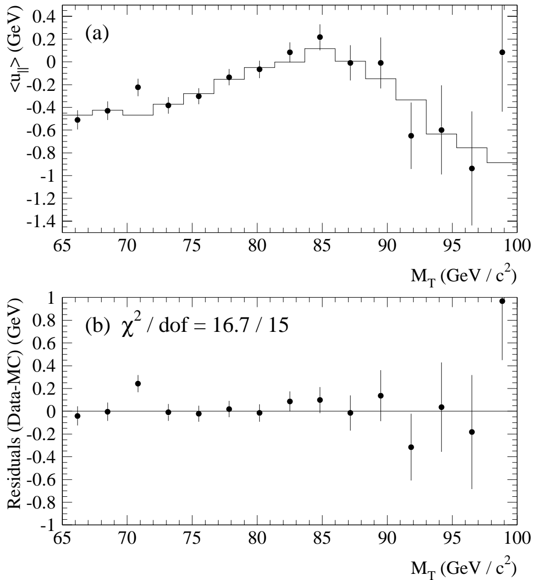
Figure 7.15: (a) The average value of u_{||} as a function of M_T for the W \rightarrow e\nu sample. The points are the data, and the solid histogram is for the simulation. (b) Residuals between the data and the simulation.
