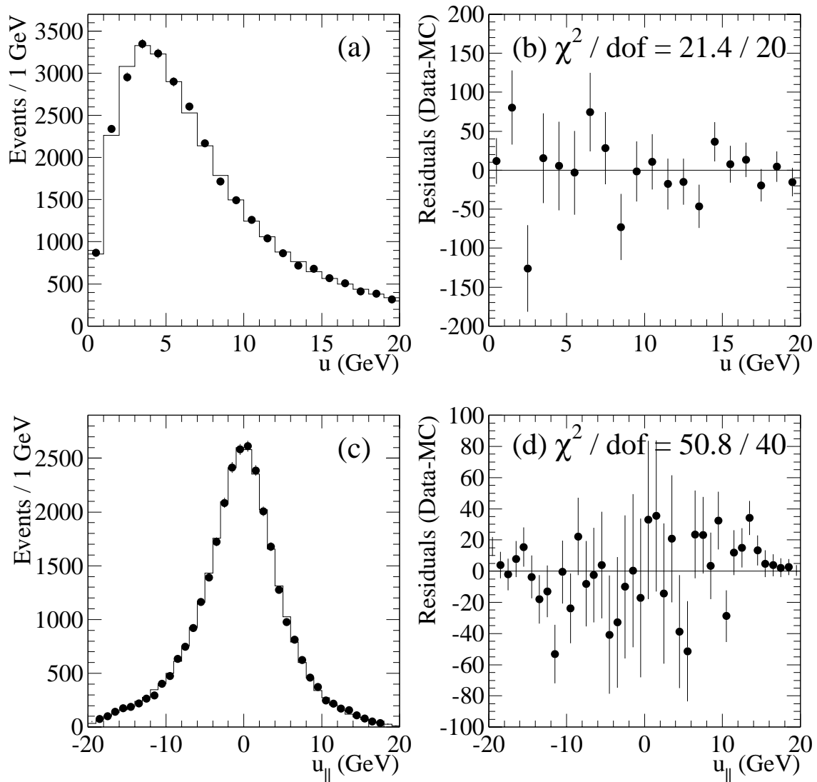
Figure 7.10: Left: The (a) |\mathbf{u}| and (c) u_{\parallel} distribution distribution for the W \rightarrow e\nu sample. The points (histograms) are the data (simulation). The differences between the data and the simulation are shown in (b) and (d).
