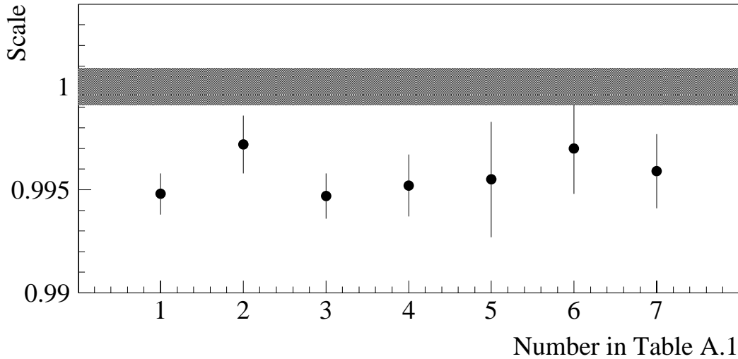
Figure A.2: Required energy scales for various data samples. The shaded area represents the energy scale determined by the Z \rightarrow e^+ e^- mass.
