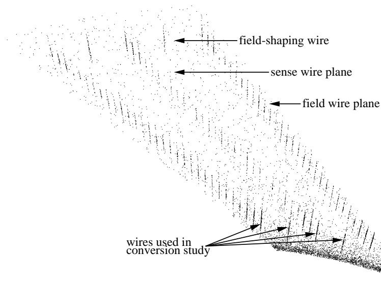
Figure 3.3: Reconstructed photon conversion vertex density in the r - \phi plane for the innermost superlayer in the CTC, folded into 1/30 of the circumference (this layer has 30-fold symmetry). Each point represents one reconstructed vertex.
