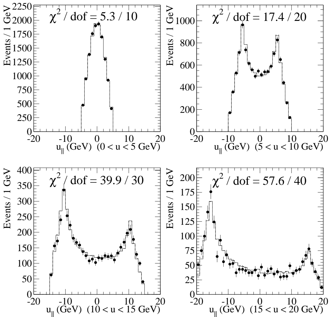
Figure 7.13: The u_{\parallel} distributions for the W \rightarrow e\nu sample in four bins of |u| . The points are the data, and the histograms the simulation.
