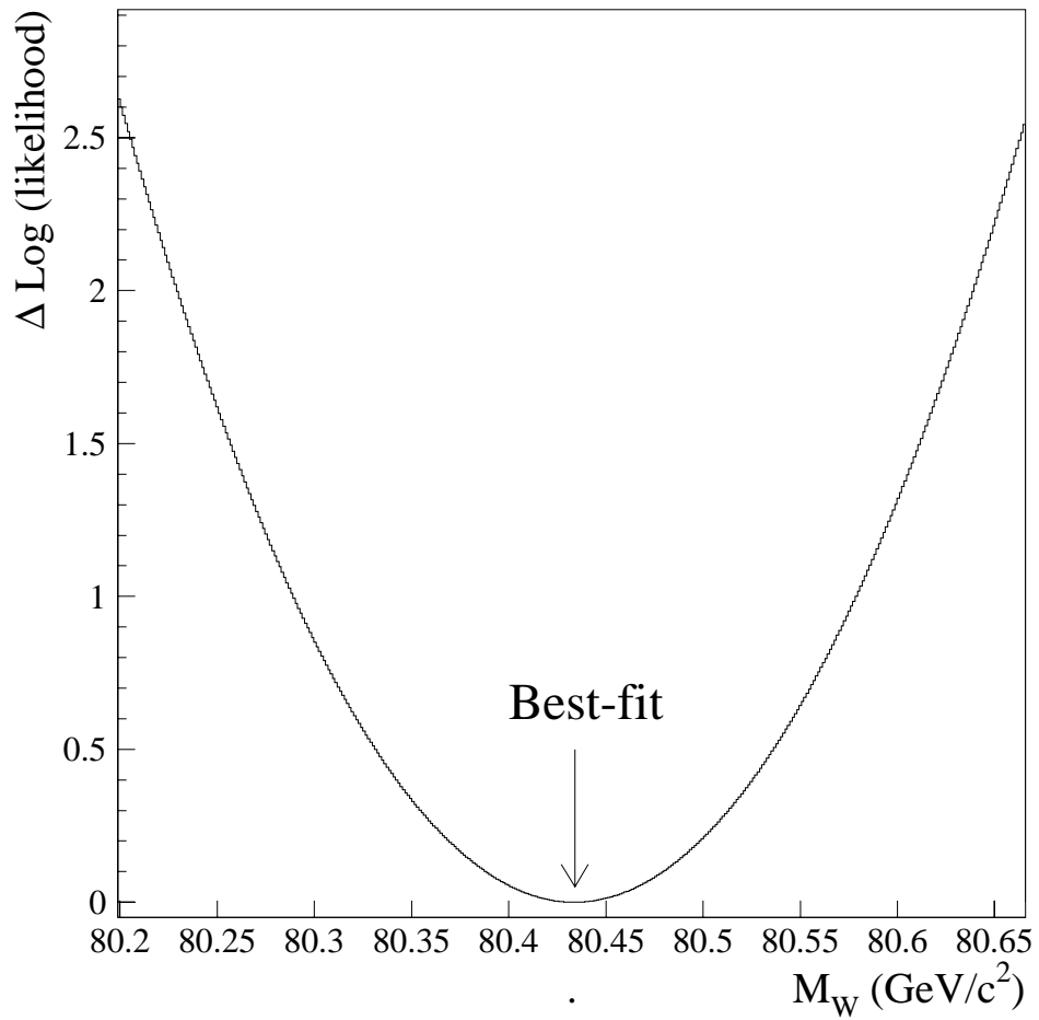
Figure 8.2: The deviation of the negative log likelihood from the minimum for the W \rightarrow \mu\nu sample. The W width is fixed at the Standard Model value in the fit.
