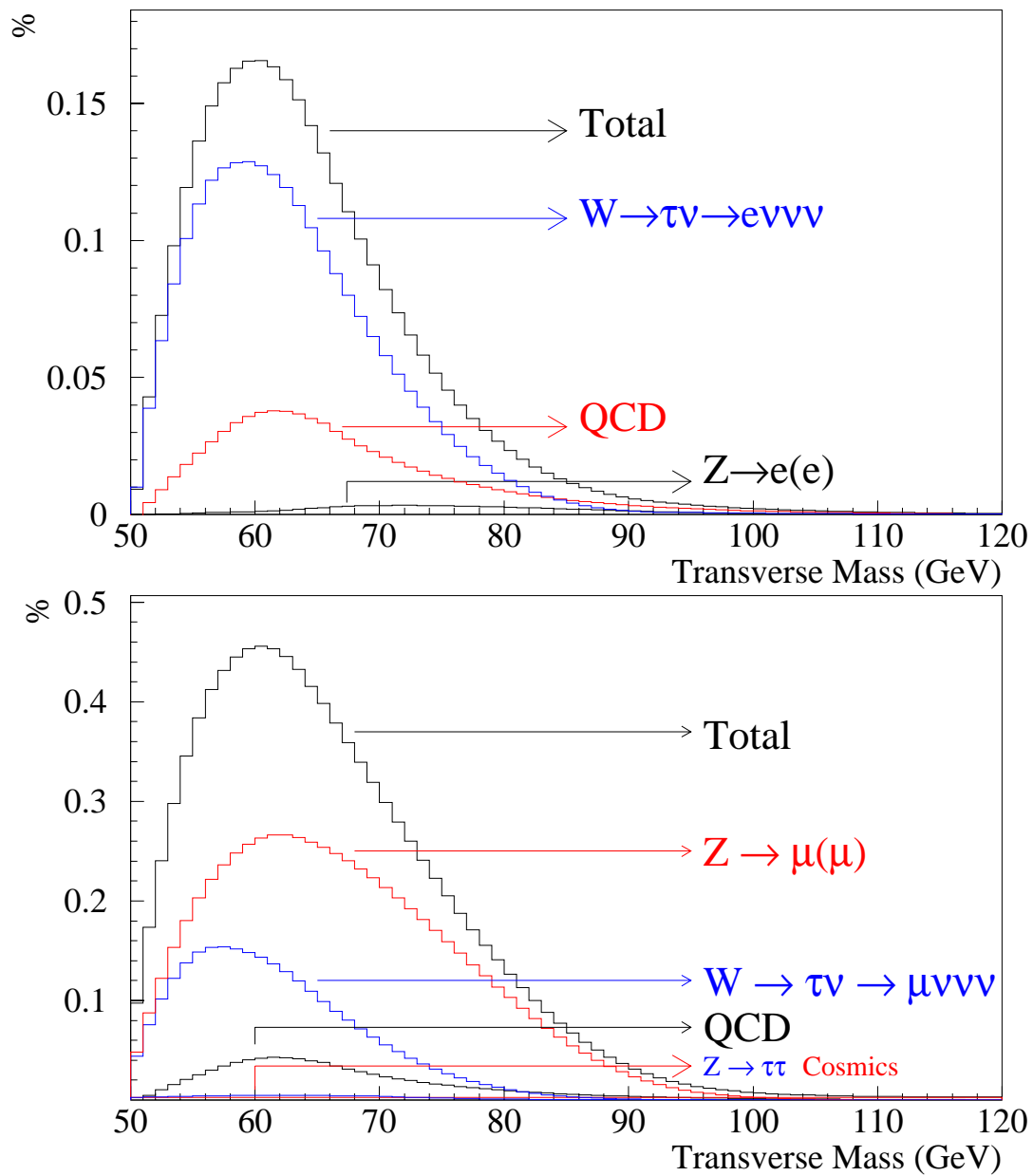
Figure 5.1: The fractions (%) of backgrounds as a function of transverse mass distribution for the W \rightarrow e\nu sample (Top) and the W \rightarrow \mu\nu sample (Bottom). The smallest contributor, W \rightarrow \tau\nu \rightarrow \text{hadrons} + \nu\nu , is not shown in this figure.
