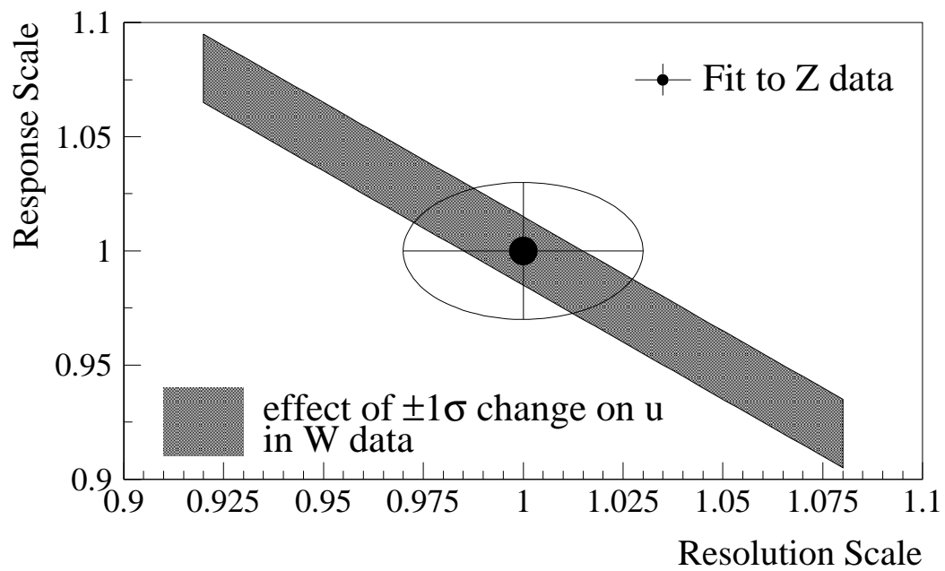
Figure 7.8: The muon Z fits separately constrain resolution and response, as shown by the ellipse, while the W data gives a further correlated constraint, as shown by the band. This is obtained from the Monte Carlo studies.
