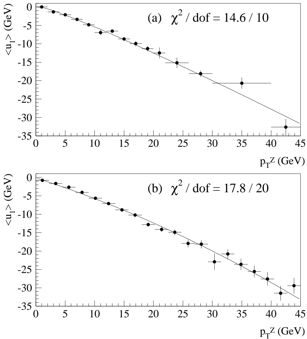
Figure 7.4: The \langle u_1 \rangle versus p_T^Z (solid lines) as derived from Z sample fits for (a) the electron channel and (b) the muon channel. The fits are compared with the data points.
