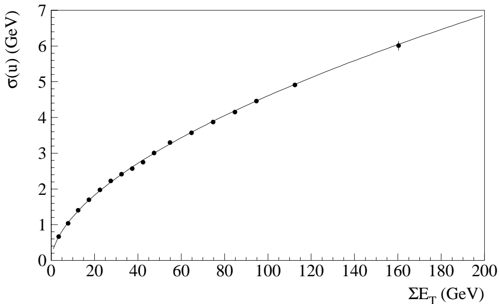
Figure 7.1: The fit for the rms of the u_x and u_y distributions as a function of \Sigma E_T using the minimum bias sample.
