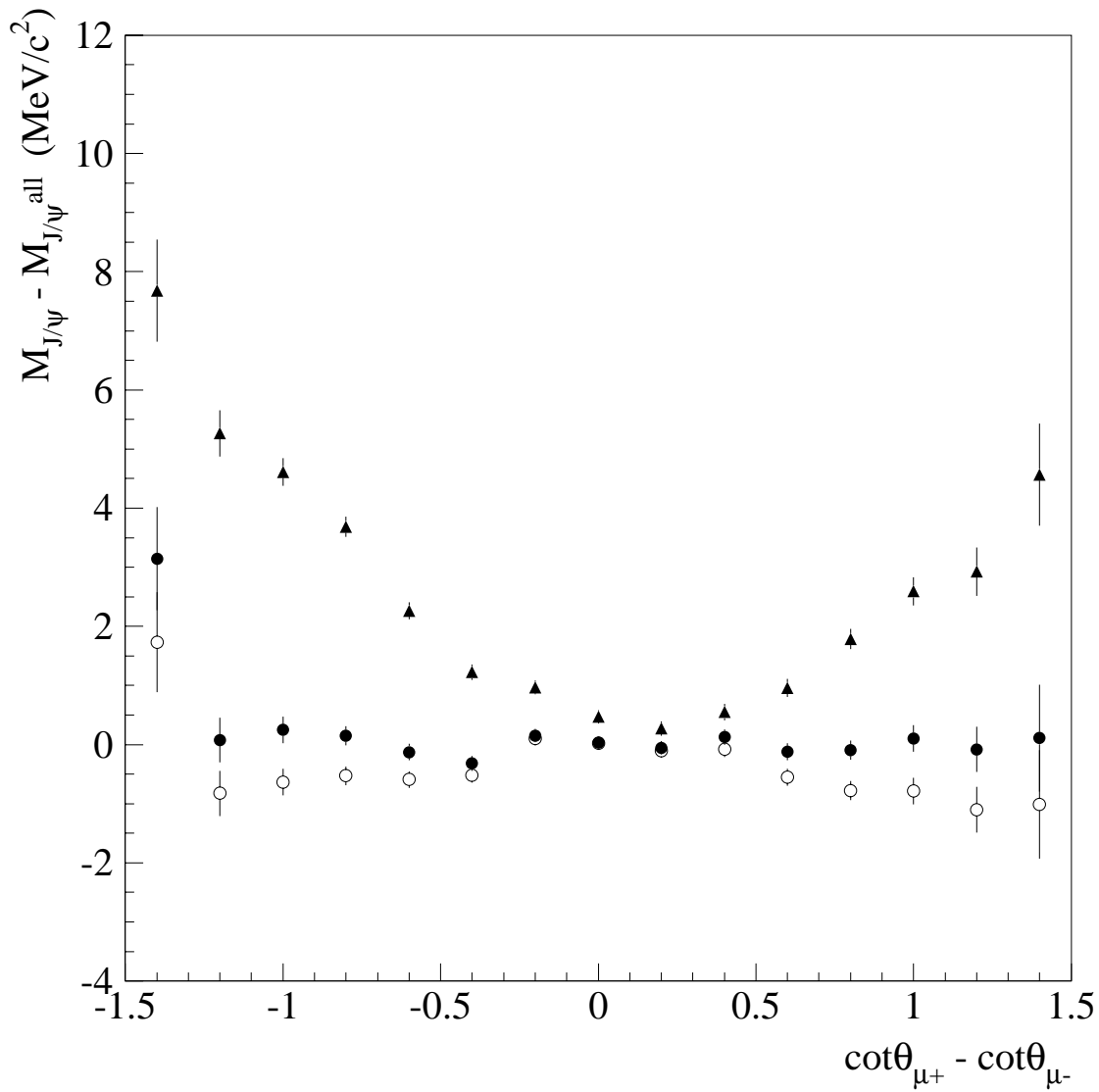
Figure 3.6: Measured J/\psi mass relative to the overall final mass measurement as a function of \Delta\cot\theta = \cot\theta_{\mu^+} - \cot\theta_{\mu^-} . The solid triangles and open circles are before and after the Run IB calibration and alignment, respectively. Solid circles show the distribution with the \cot\theta correction of 1.0004 \times \cot\theta .
