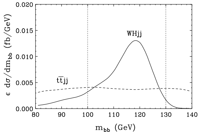
FIG. 1. b\bar{b} invariant mass distribution of the WHjj signal (solid) for M_H = 120 GeV and t\bar{t}jj background (dashed) after the cuts of Eqs. (1),(2), a minijet veto and application of expected detector ID efficiencies as discussed in the text; \epsilon = 0.25 . Vertical dotted lines denote the mass bin used for calculating statistical significance of the signal.
