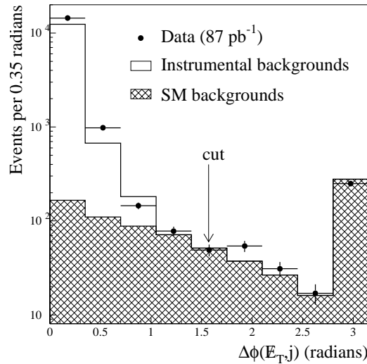
FIG. 1. The distribution of \Delta\phi(\not{E}_T, j) for events before the \Delta\phi cut is applied (points), compared to the instrumental backgrounds inferred from the control sample (white area) and the Standard Model backgrounds (shaded area).
