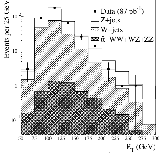
FIG. 2. The distribution of \cancel{E}_T for data (points) compared to the central value expectations from Z + jet events (white area), W + jet events (shaded area) and for t\bar{t} + WW + WZ + ZZ events (hatched area).
