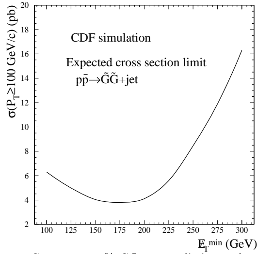
FIG. 4. The 95% C.L. upper limit on the cross section for \tilde{G}\tilde{G} + jet events with P_T^{\tilde{G}\tilde{G}} \geq 100 GeV/c expected for no signal.
