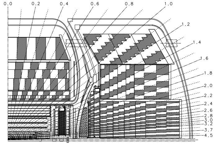
Figure 30. One quadrant of the DØ calorimeter and drift chamber, projected in the x - z plane. Radial lines illustrate the detector pseudorapidity and the pseudoprojective geometry of the calorimeter towers. Each tower is of size \Delta\eta \times \Delta\phi = 0.1 \times 0.1 .
