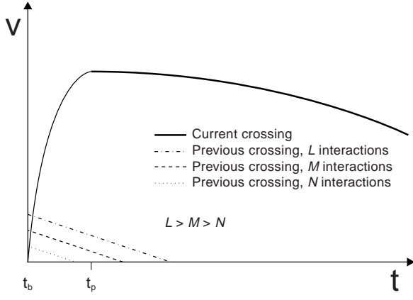
Figure 22. Schematic of voltage in a calorimeter cell as a function of time. The solid line shows the contribution for a given event (the current crossing). The cell is sampled once at t_b , just before a p\bar{p} bunch crossing, to establish a base voltage. The voltage rises during the time it takes electrons to drift in the liquid argon gap ( \sim 500 ns), and reaches a peak value at t_p \approx 2 \mu\text{s} , which is set by pulse-shaping amplifiers in the signal path. The cell is sampled again at t_p , and the voltage difference \Delta V = V(t_p) - V(t_b) is proportional to the raw energy in the cell. Because the decay time of the signal \tau \approx 30 \mu\text{s} is much larger than the accelerator bunch crossing time t_x = 3.5 \mu\text{s} , V(t_b) may have a contribution from a previous bunch crossing. The size of this contribution is related to the number of p\bar{p} interactions in the previous crossing, which depends on the beam luminosity. The dashed lines show an example contribution from a previous bunch crossing containing three different numbers of p\bar{p} interactions. The figure is not drawn to scale.
