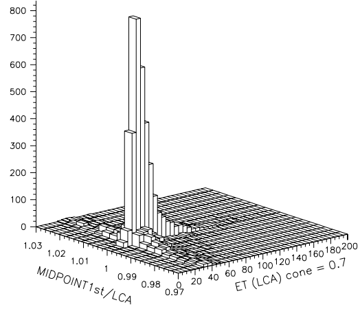
Figure 16. E_T ratios for leading jets. The ratio of leading jet E_T in the midpoint algorithm is plotted as a function of the legacy cone jet's E_T .
