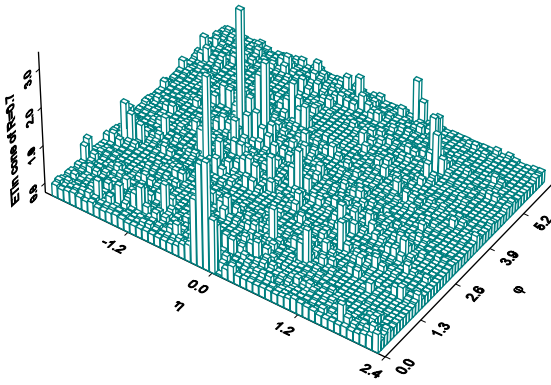
Figure 9. A sample event from data. Tower E_T lego plot for an event passing the D\bar{O} W \rightarrow jets trigger.
