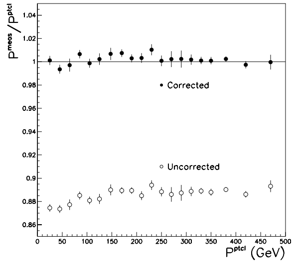
Figure 34. Monte Carlo verification test. The vertical bars are statistical errors. Systematic errors (not shown) are of the order of 0.01–0.02. The corrected p_{jet}^{meas}/p_{jet}^{ptcl} ratio is consistent with unity within errors.
