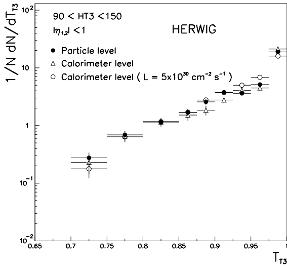
Figure 37. Same as Fig. 36 but only the three leading jets contribute to T_T , now T_{T3} . H_{T3} is the scalar sum p_T of the three leading jets in the event.
