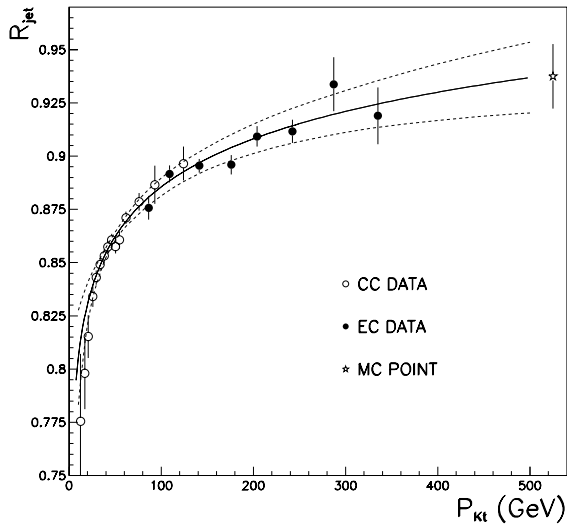
Figure 33. R_{jet} versus K_T jet momentum. The solid lines are the fit and the dashed band the error of the fit. (The three lowest points have nearly fully correlated uncertainties and are excluded from the fit.)
