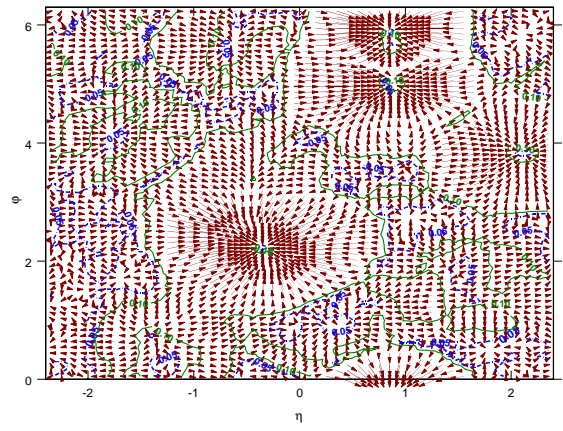
Figure 8. Energy flow for the cones in the large- E_T jet event of Figs. 6–7. The contours bound flow regions with vector magnitude < 0.1 (solid contours) and < 0.05 (dashed contours) in \eta \times \phi .
