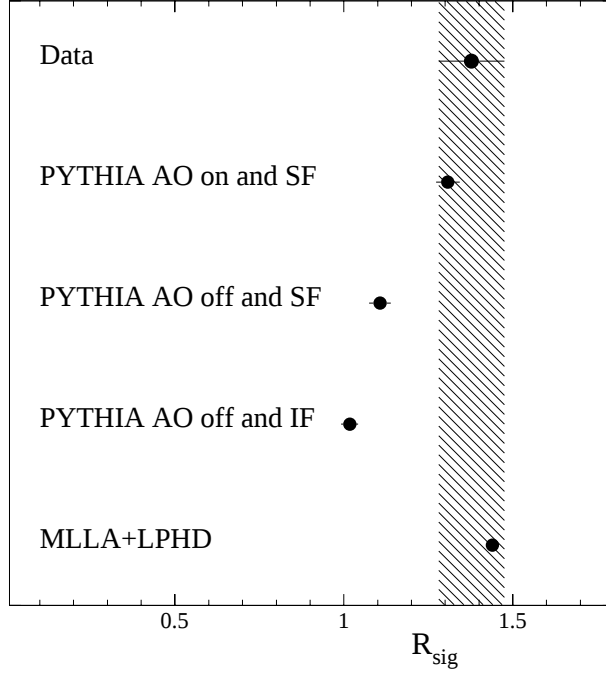
FIG. 5. R_{\text{sig}} for D0 data, PYTHIA with various coherence implementations, and a MLLA+LPHD QCD calculation. The errors are statistical only and the shaded band shows the statistical uncertainty on the R_{\text{sig}} variable for the data.
