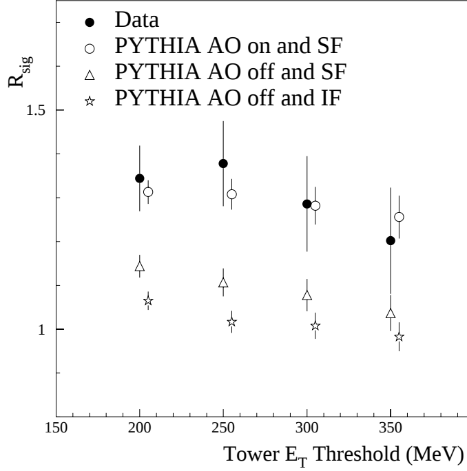
FIG. 6. R_{\text{sig}} as a function of the tower E_T threshold for the data (solid circles) and for the various PYTHIA predictions. All uncertainties are statistical only.
