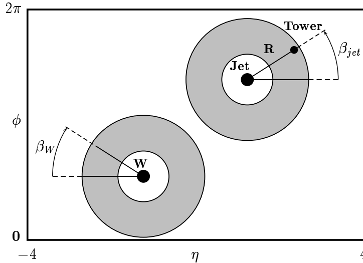
FIG. 1. Annular regions around the W boson and the tagged jet in (\eta, \phi) space.
