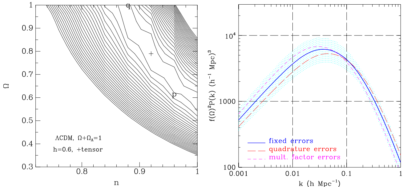
Fig. 3.— Left panel: Contour plot of \ln\mathcal{L} in the \Omega - n plane for the SFI sample, for the tilted \Lambda CDM model with tensor fluctuations and h = 0.6 , using the original error estimates. The best-fit point is marked with a ‘+’. The maximum likelihood locations when varying the errors in quadrature (‘q’) or by a multiplicative factor (‘p’) are also marked. Right panel: The most-likely PS for this model, for these three variants of the errors. The dotted region around the PS represents the 90% confidence limit for the case of the original errors (thick line), obtained from the high-likelihood ridge shown in the contour map.
