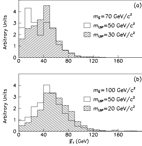
FIG. 1. The expected distributions of \cancel{E}_T for m_{\tilde{b}} values of 70 (a) and 100 (b) \text{GeV}/c^2 , for the indicated values of m_{\text{LSP}} [7].
