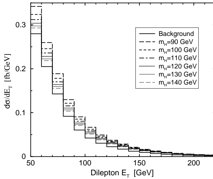
Figure 2: The distribution of the background and signal+background for ZH_{\text{inv}} \rightarrow l^+l^- + \cancel{E}_T as a function of the dilepton E_T , or equivalently, \cancel{E}_T . This distribution is plotted after all cuts and efficiencies have been applied except the cut on E_T .
